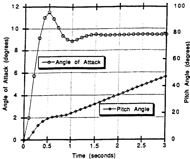
Figure 10. Typical Pitch Response to Step Elevator Deflection
