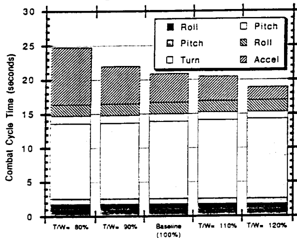
Figure 15. CCT Variation with Thrust Load
