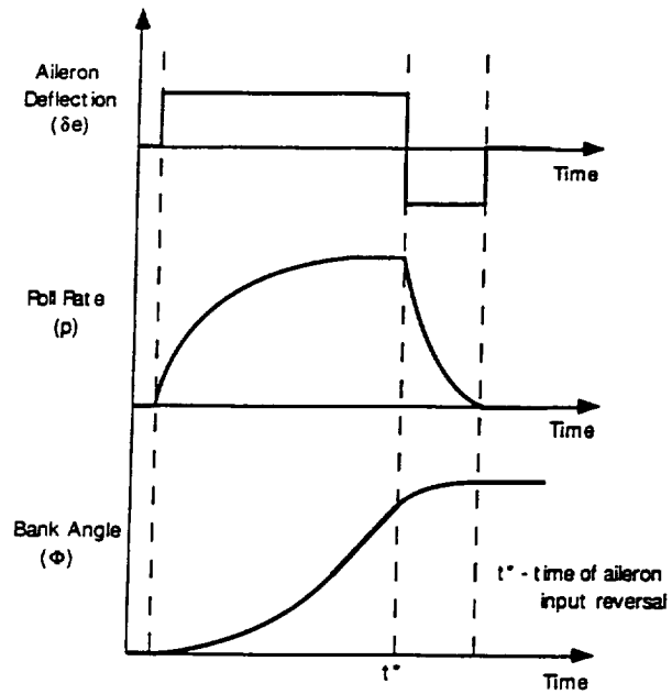
Figure 9. Roll Maneuver
