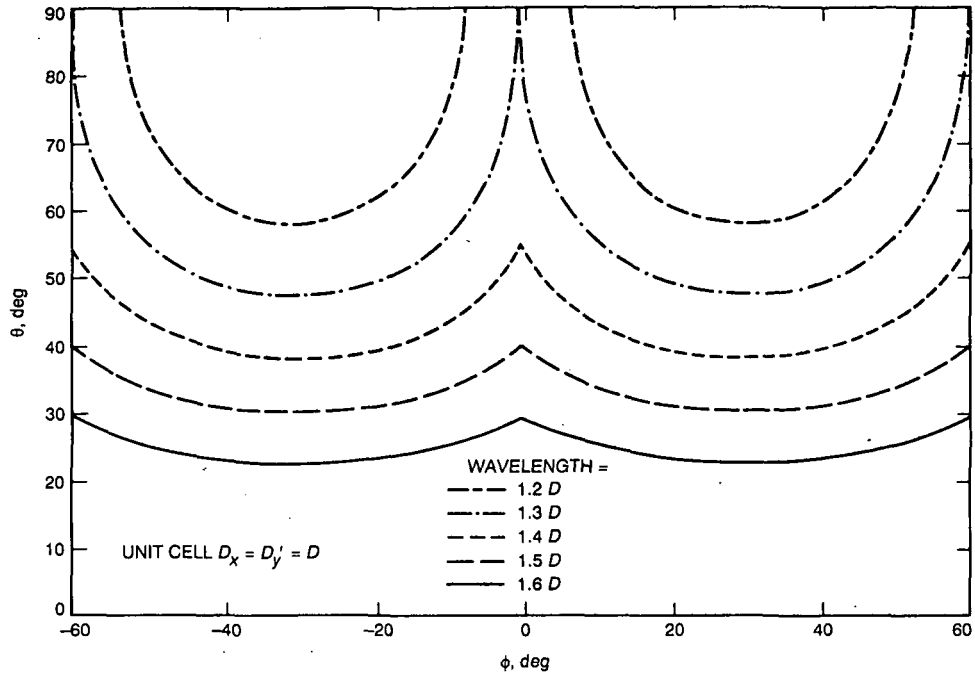
Fig. 8. Grating lobe curves for various frequencies (wavelength = 1.2 D to 1.6 D ) with a cell of D_x = D , D_y = 0.866D , and \Omega = 60.0 \text{ deg} , where D is a unit length.
