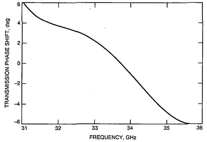
Fig. 6. Phase shift between TE and TM polarization versus frequency for X-/Ka-band dichroic plate.
