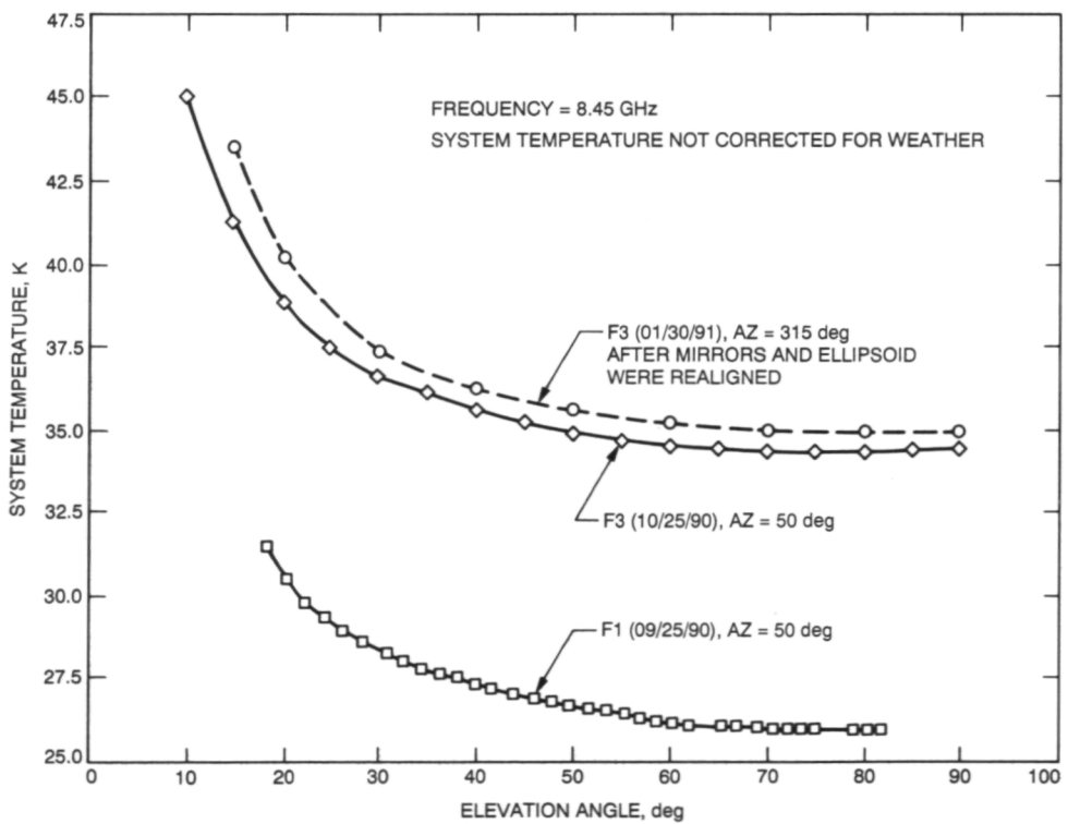
Fig. 8. X-band tipping curves at F1 and F3.
