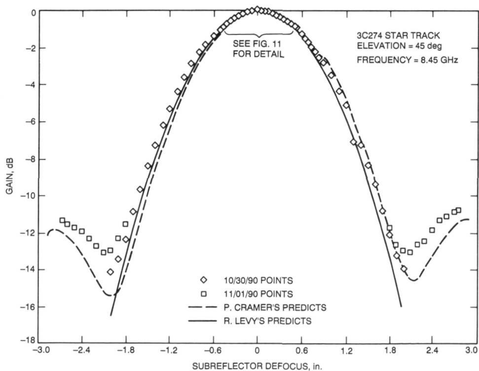
Fig. 10. X-band subreflector Z-defocus curve measured at F3.
