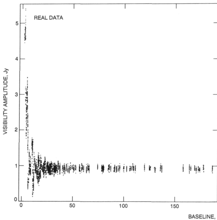
Fig. 6. Comparison of data (Fig. 4) and simulation (Fig. 5) for the VLA observations on September 28, 1990.
