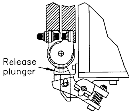
Plunger Assembly, Released Top View
