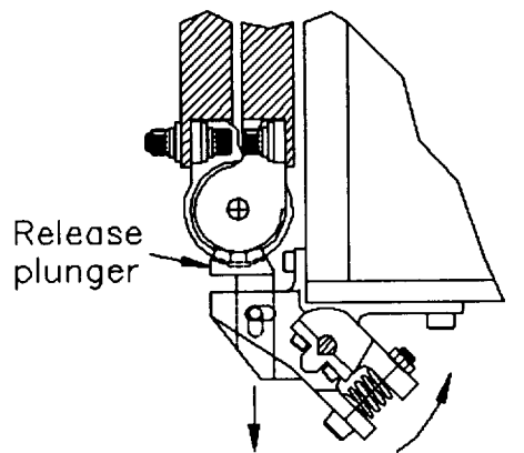
Plunger Assembly, Stowed Top View
