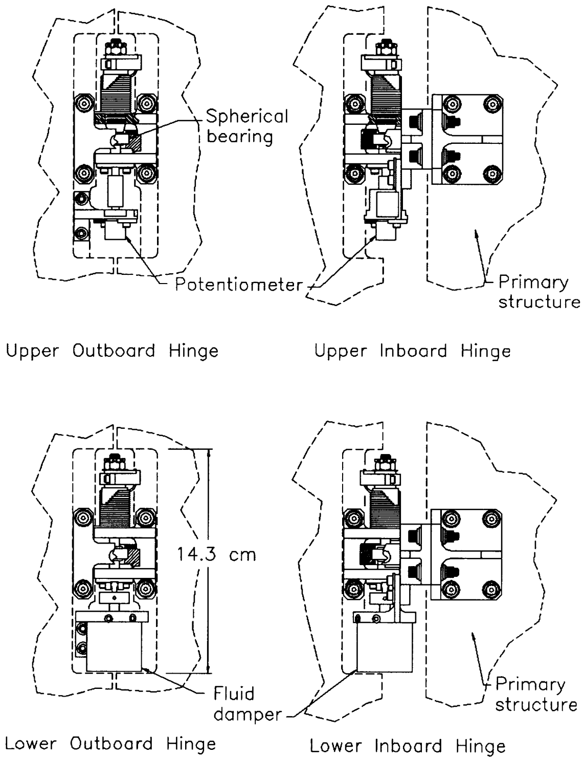
Figure 4: Solar Array Hinges
