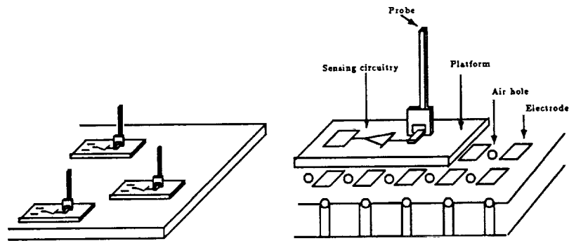
Figure 2. Probing platforms floating on air bearing
