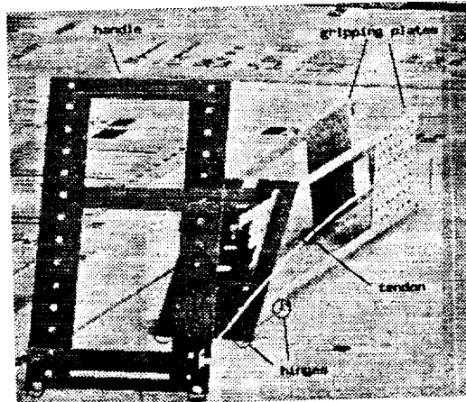
Figure 8. A parallel plate gripper. The gripper is normally closed, with a gap of 100\text{ }\mu\text{m} between the plates. Pulling the vertical bar (left side) causes the jaws to open. Opening of 0.5 millimeter is possible with no damage to the device.
