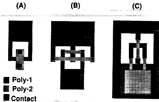
Figure 6. Three basic hinge types (A) A substrate hinge, which is used to hinge released structures to the substrate. (B) A 'concave down' scissor hinge, used to hinge released structures to each other. (C) A 'concave up' scissor hinge.
