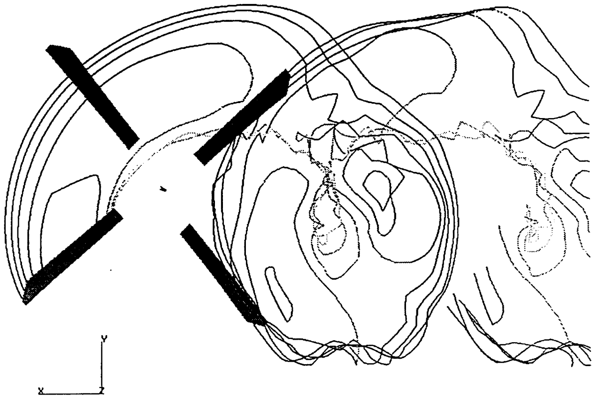
c) Reference blade at \Psi = 225^\circ
