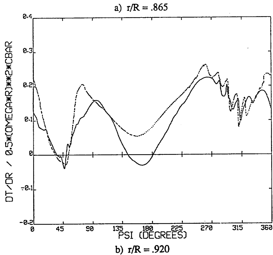
Figure 7-22. Sikorsky UH-60A dC_T/dx for Test Point 1126; 20 filaments and 32 time steps reconstructed to 960 time steps; refined vortex core with low vortex age parameter (solid = measured, dotted = predicted).
