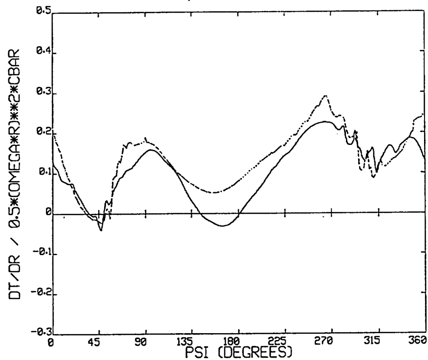
Figure 7-15. Sikorsky UH-60A, dC_T/dx for Test Point 1126 with 256 time steps per blade revolution; refined vortex core model (solid = measured, dotted = predicted).
