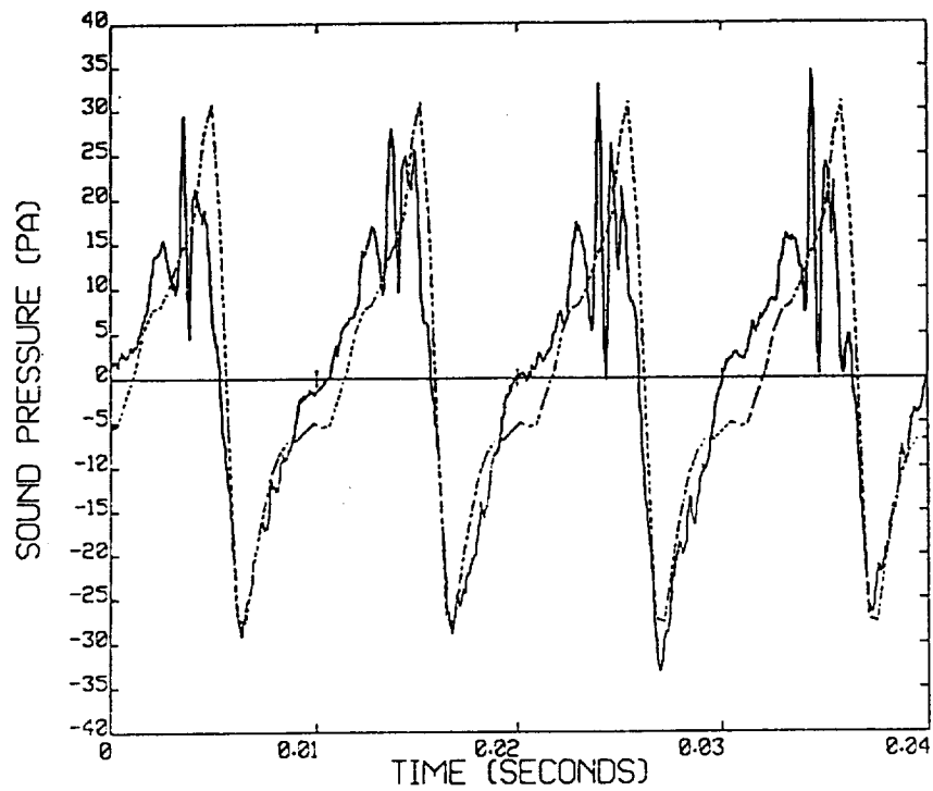
a) Microphone 3
