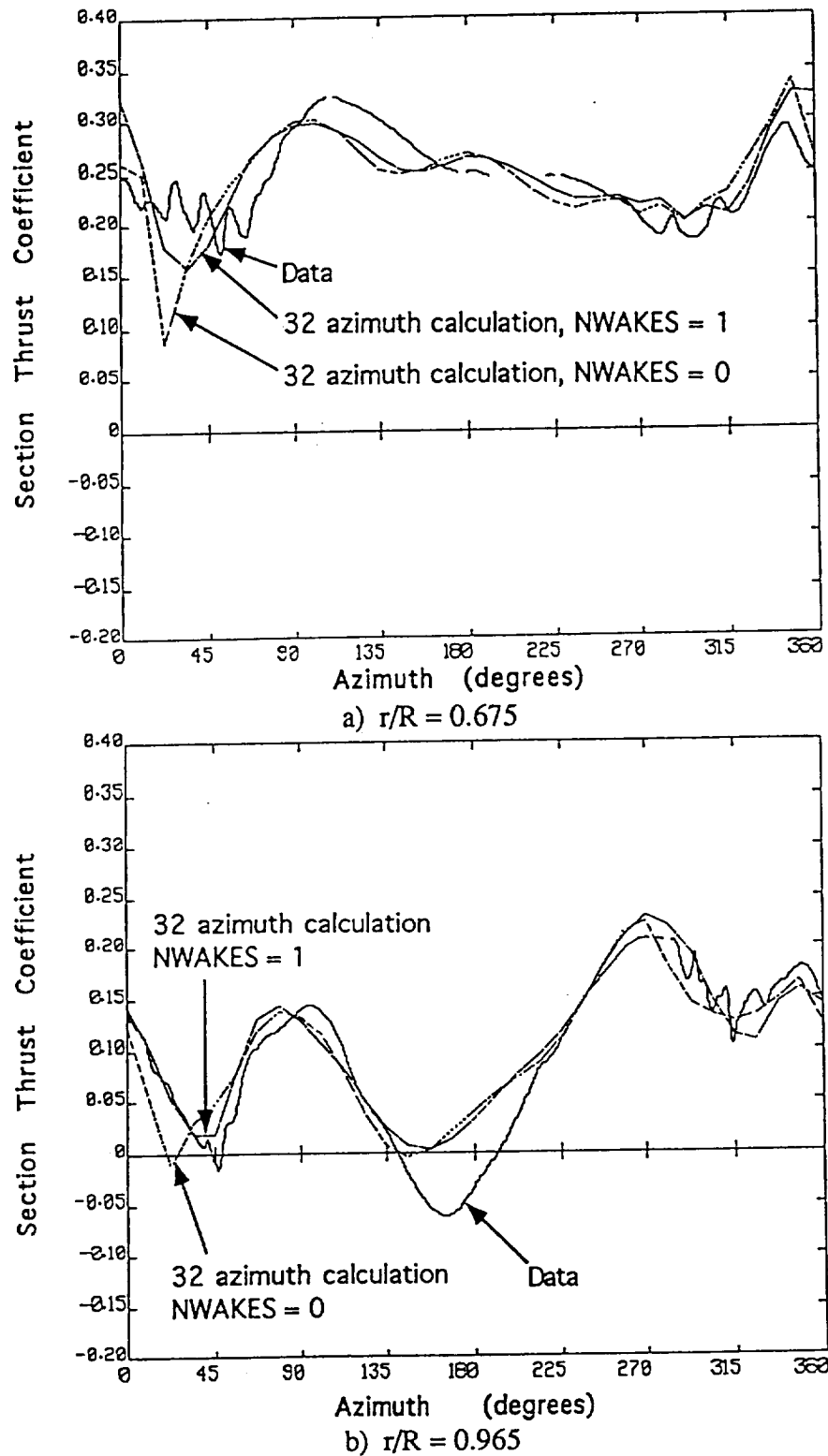
Figure 7-8. Sikorsky UH-60A model rotor dC_T/dx for Test Point 1126: comparison of measured data and predictions with and without full wake-on-wake influence.
