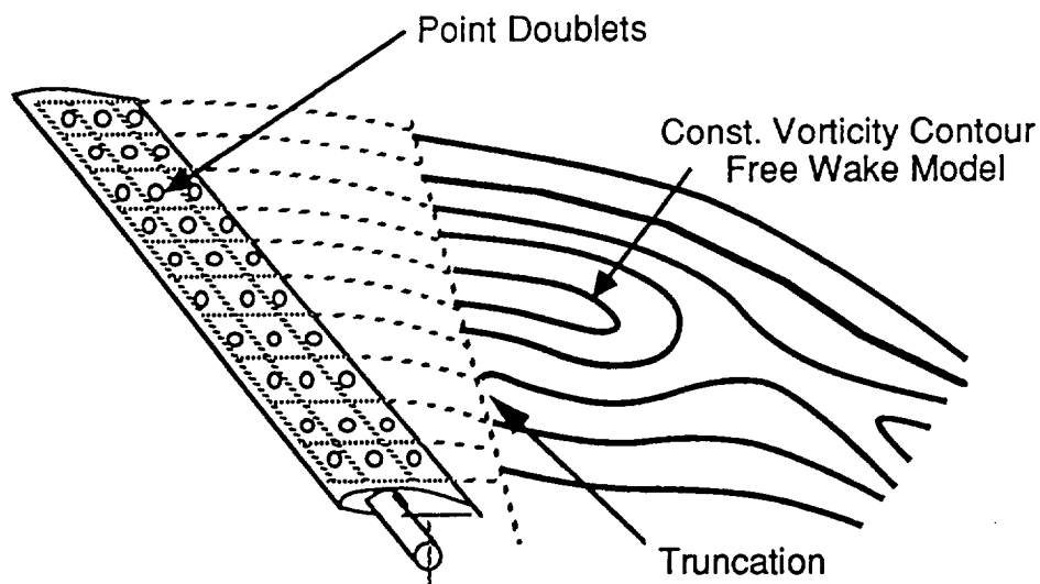
b) Truncation of the near wake for coupling to rotor wake model
