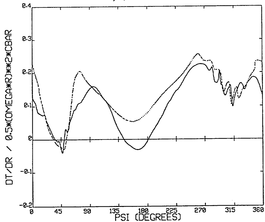
Figure 7-21. Sikorsky UH-60A dC_T/dx for Test Point 1126; 20 filaments and 32 time steps reconstructed to 960 time steps; baseline Scully core model (solid = measured, dotted = predicted).
