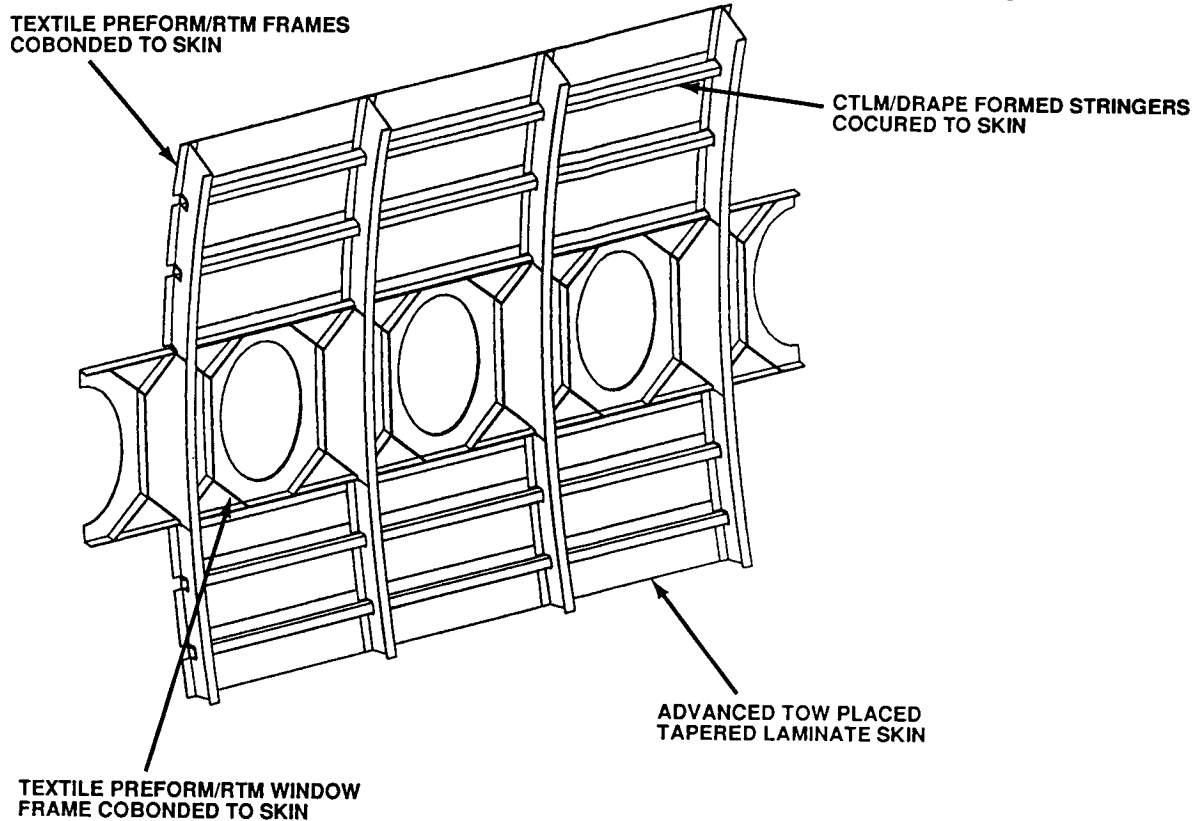
Figure 4-4: Side Baseline Design Concept and Fabrication Processes Near the Window Belt
