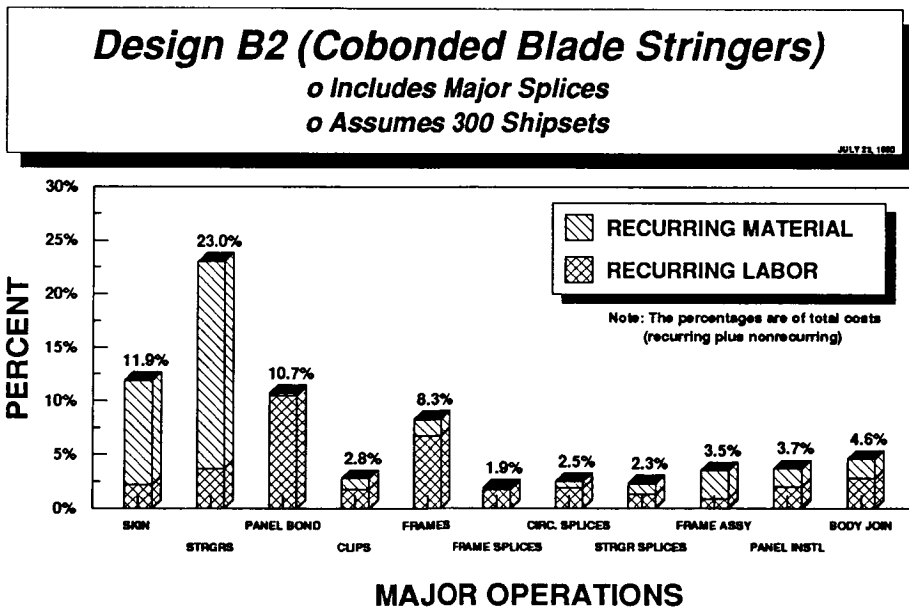
Figure 5-9: Recurring Costs by Major Operation of Design B2
