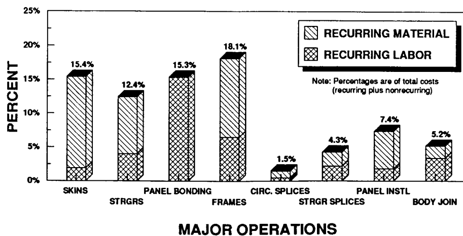
Figure 5-17: Recurring Costs by Major Operation of Design C2
