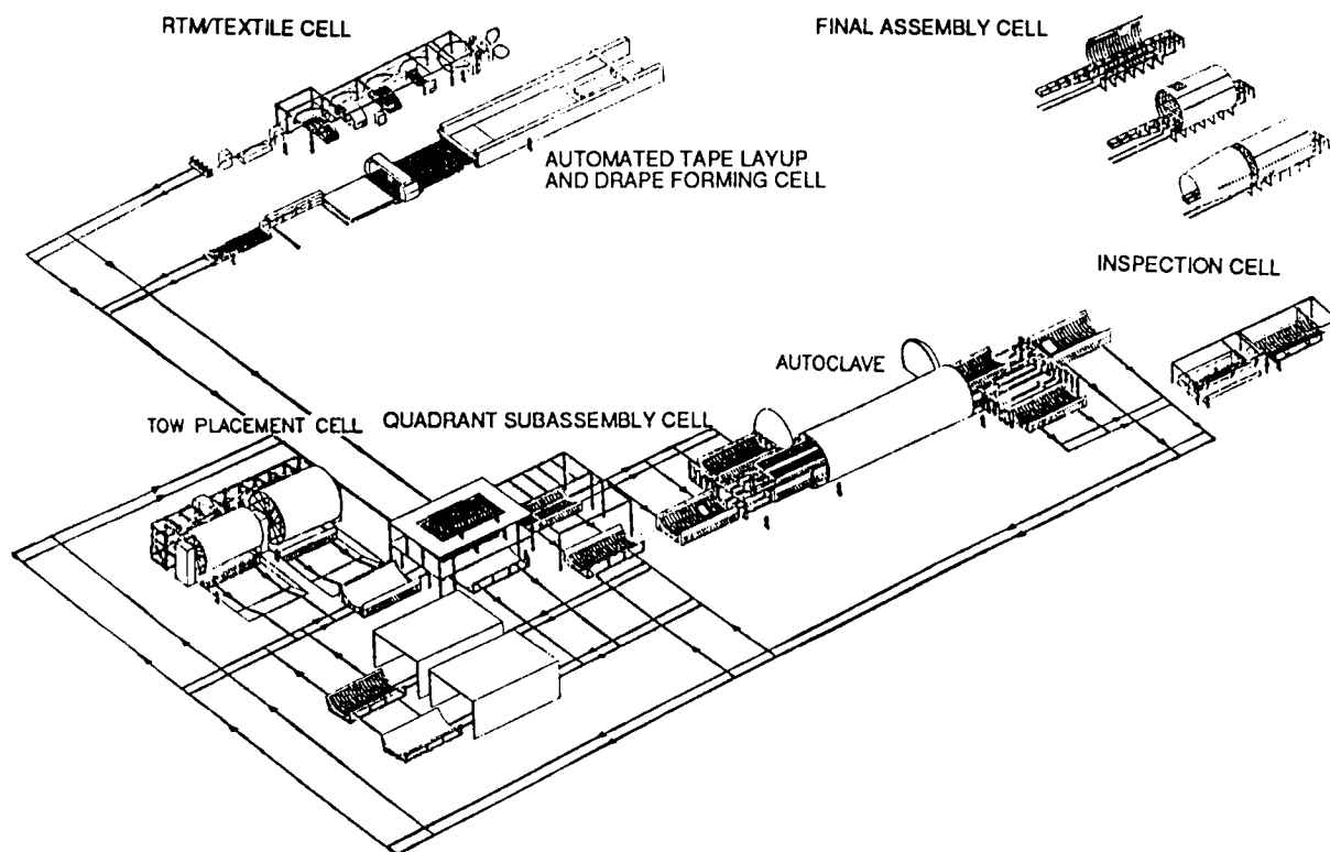
Figure 4-6: Full Factory Layout
