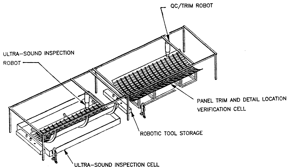
Figure 4-12: Inspection Work Station
