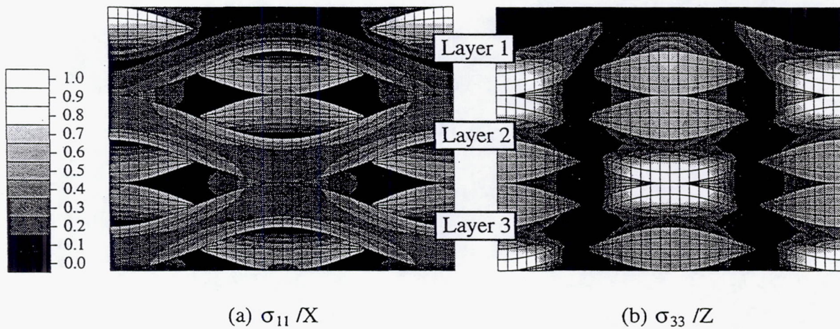
Fig. 13. Contour plots of normalized stresses for upper 3 mats. The stresses were transformed to the material coordinate systems and normalized by the strengths.
