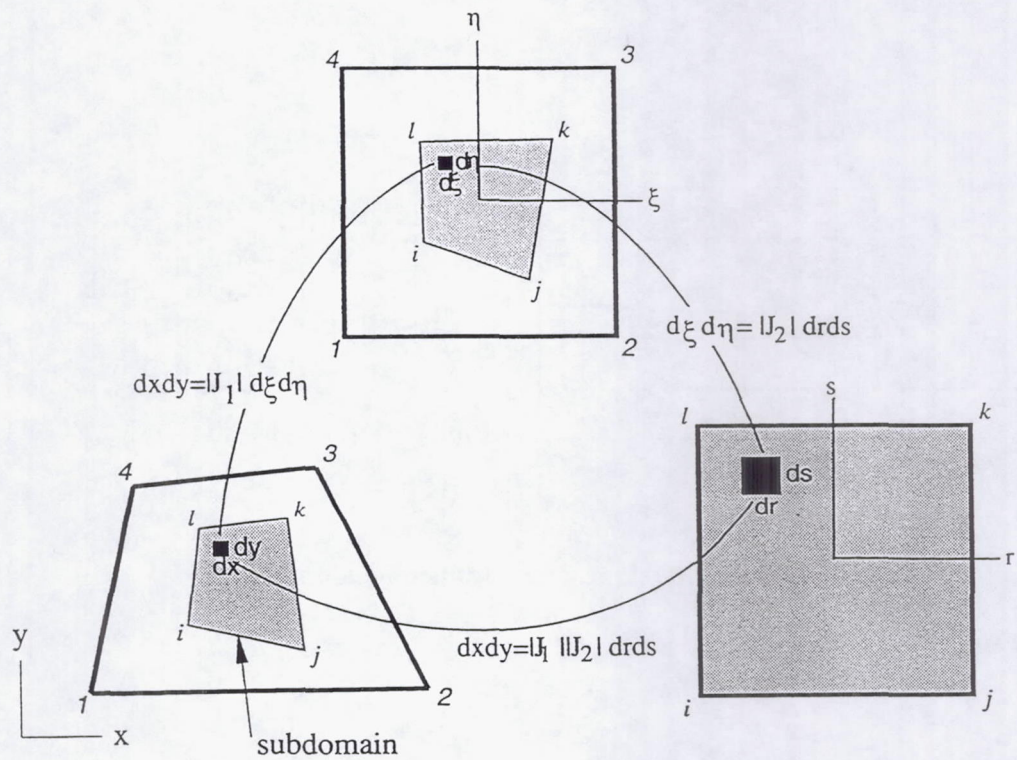
Fig.4. Mapping in three coordinate systems.
