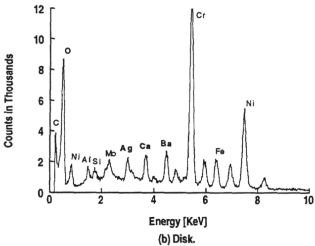
Figure 12.—EDS spectra of specimen wear tracks after 750 °C test showing increased oxygen and lubricant transfer from block to disk.
