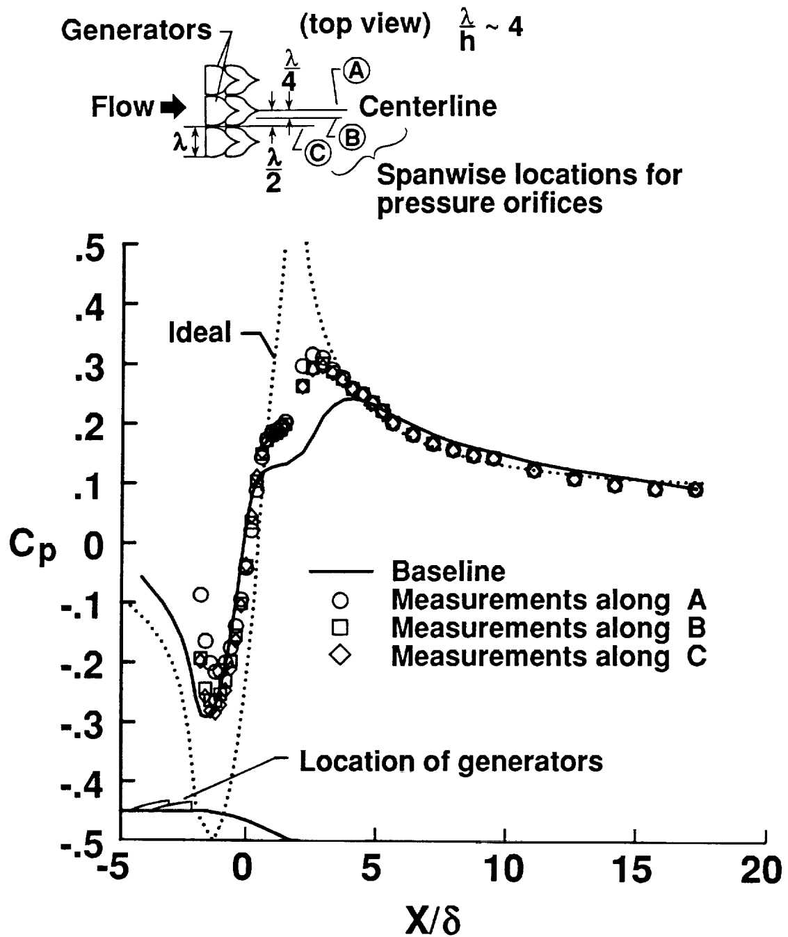
(a) 0.4\delta high doublet vortex generators.
