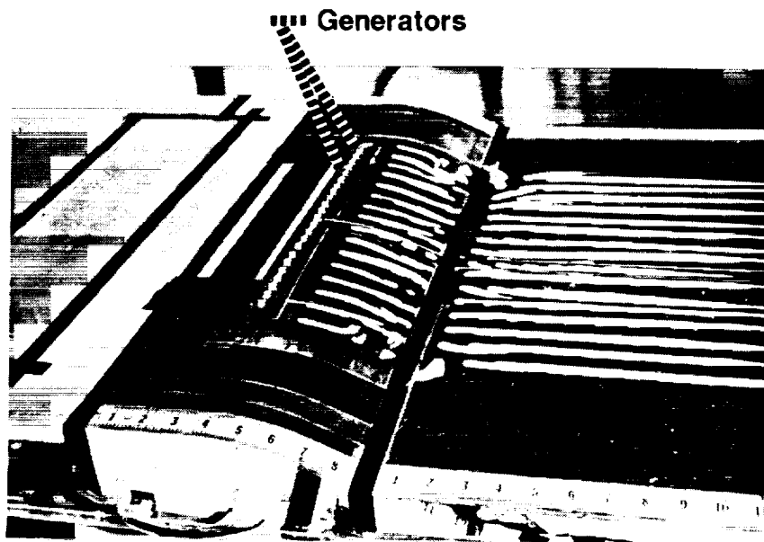
(a) 0.1\delta high vane-type vortex generators.
