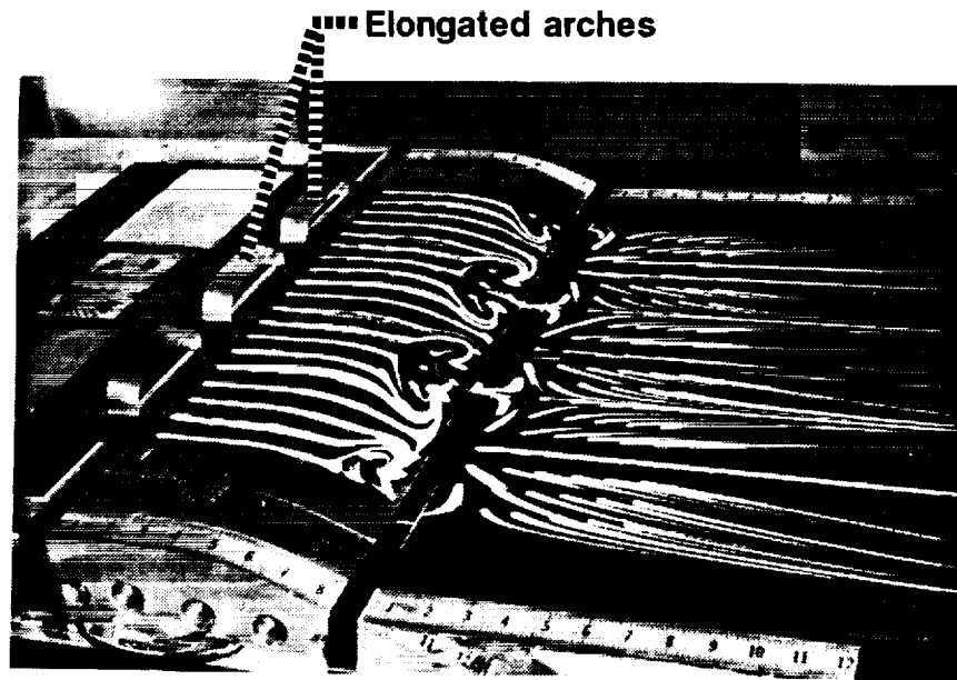
(a) Arches at 5\delta upstream of baseline separation.
