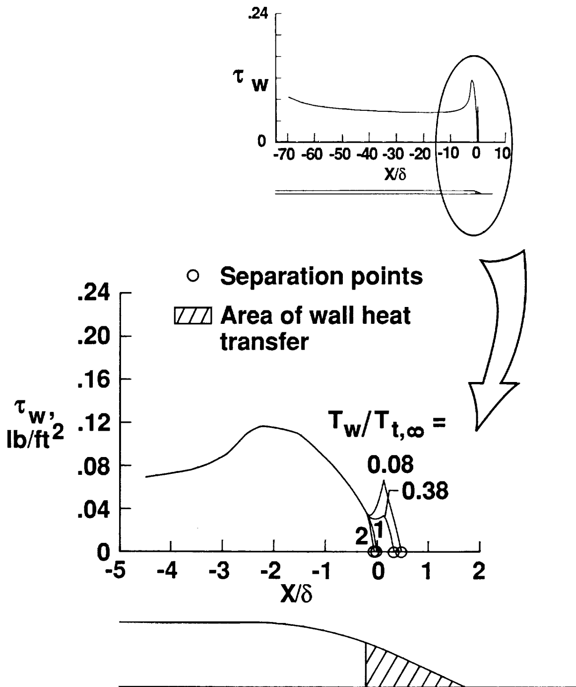
(c) Partial surface coverage from 0.2\delta upstream of the adiabatic reference separation.
