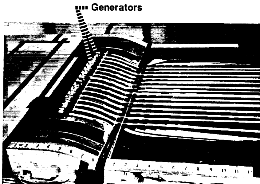
(b) 0.2\delta high vane-type vortex generators.
