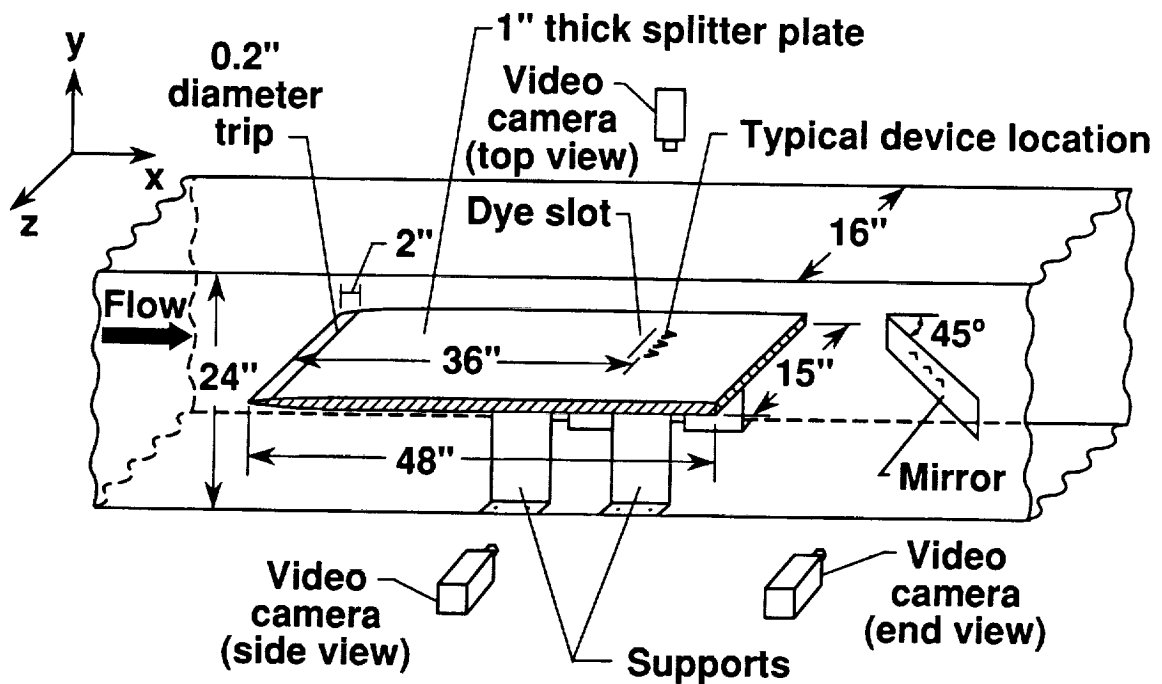
(b) Test configuration in water tunnel.
