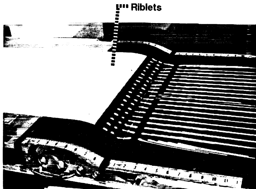
(a) 0.003-in.-high C_f -reducing riblets.
