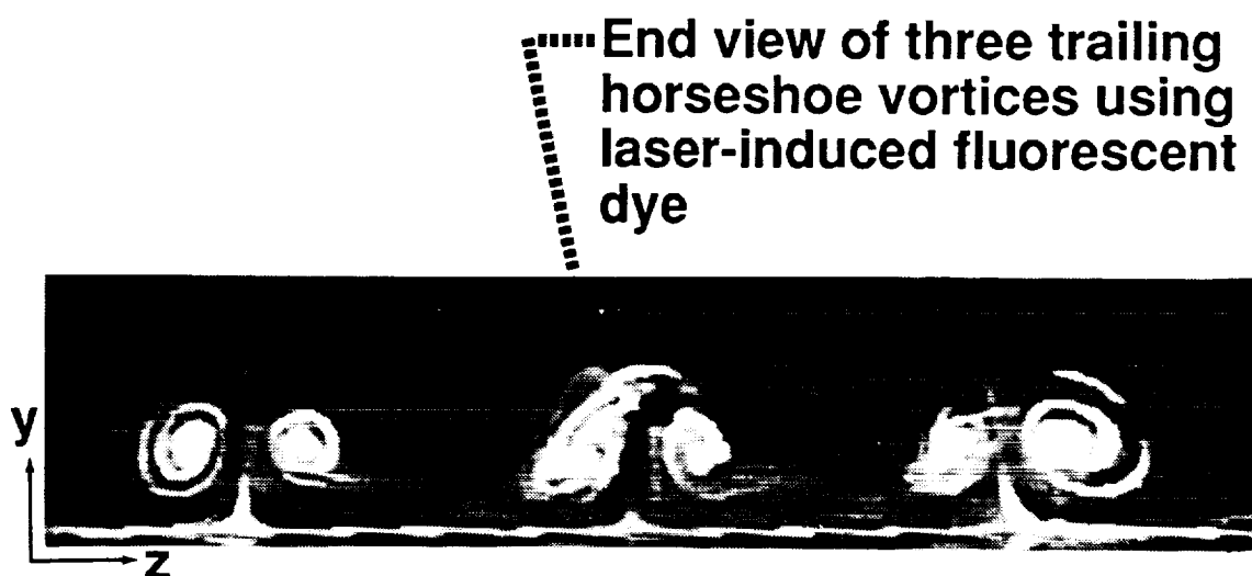
Figure 3.2 Example of dye-flow visualization for forward-facing wishbone vortex generators at U_{\infty} = 1 in/s.
