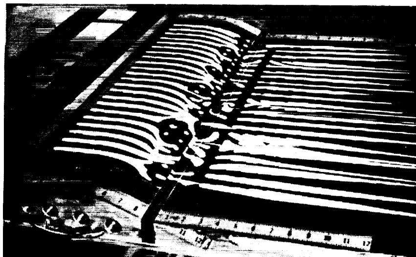
(b) Arches at 40\delta upstream of baseline separation.
