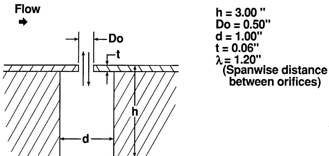
(i) Helmholtz Resonators.
