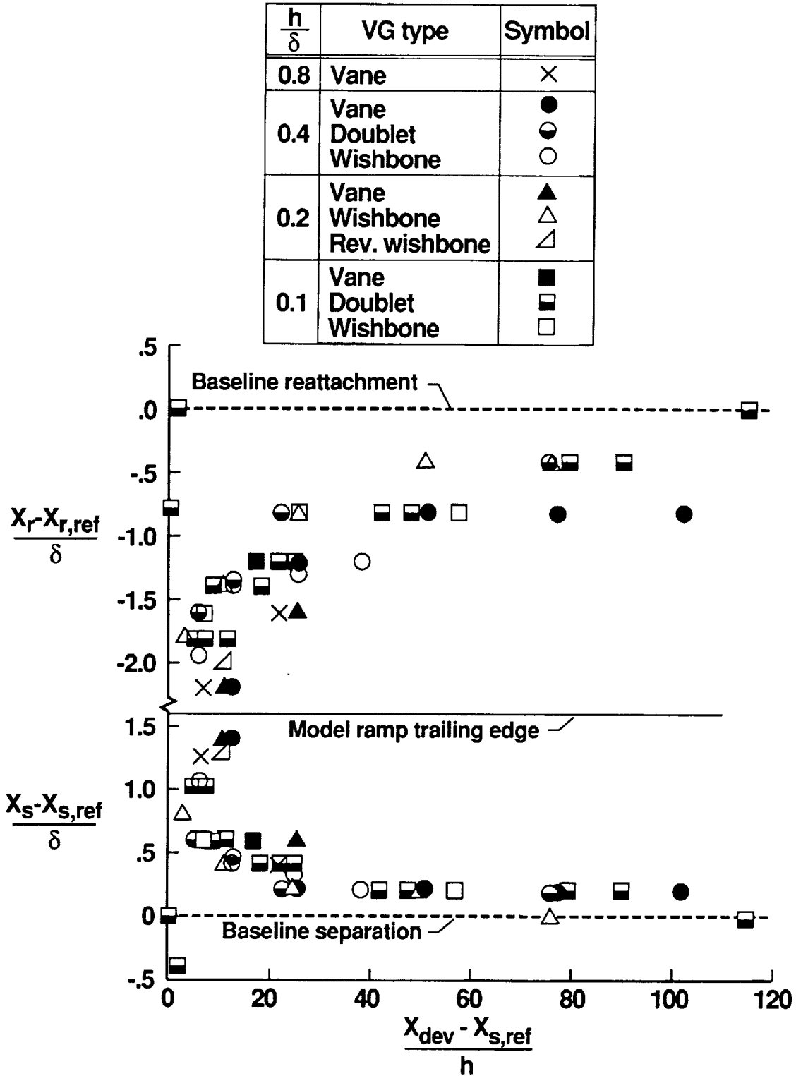
Figure 4.24 Effect of streamwise device location on separation control for all vortex generators.
