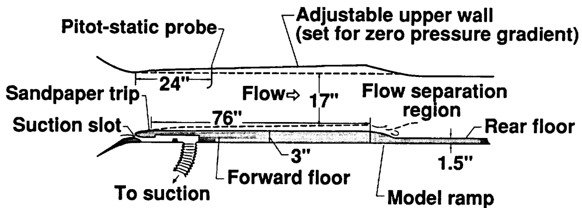
(b) Test configuration in wind tunnel.
