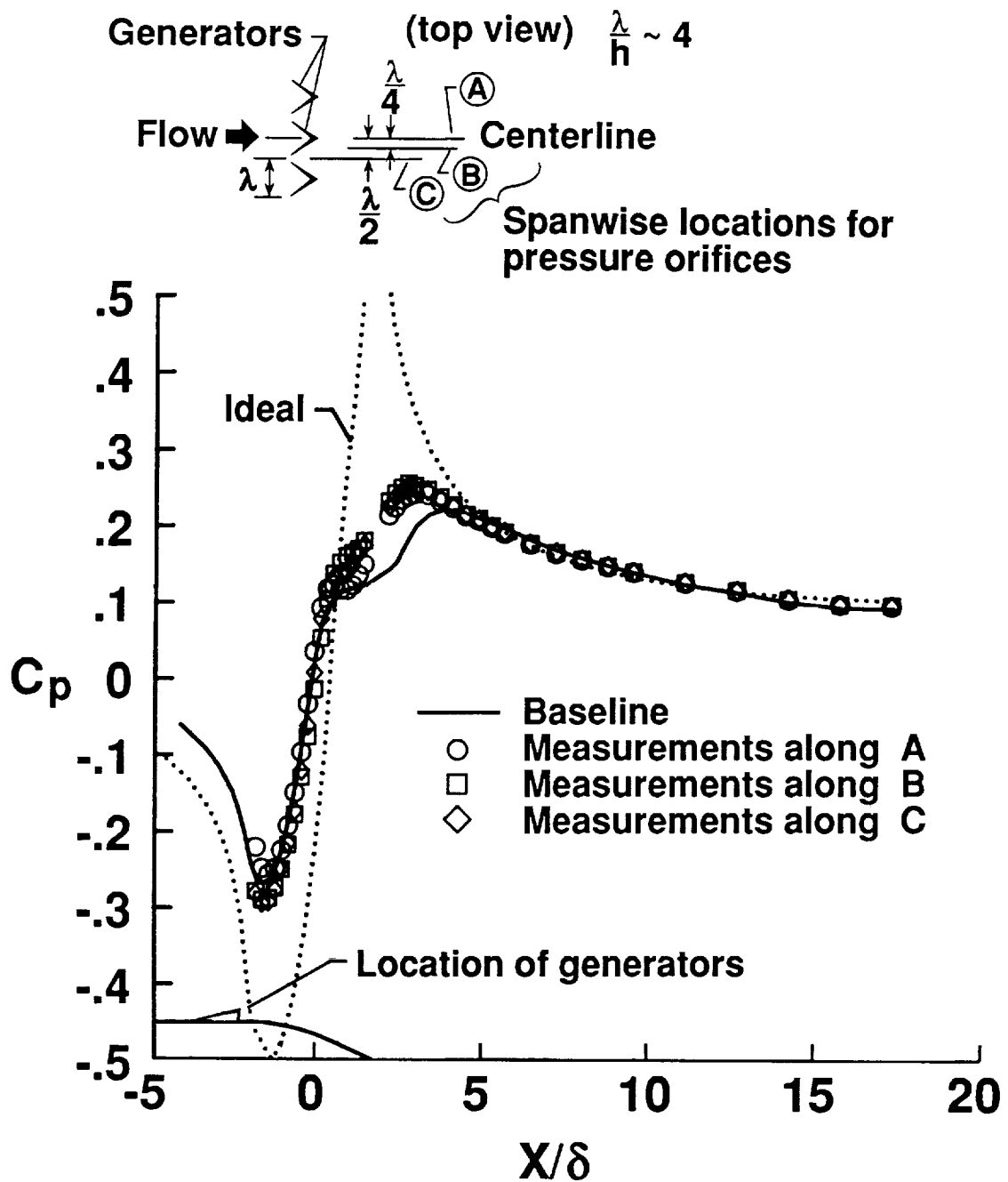
(a) Generators in forward configuration.
