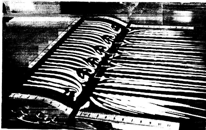
(b) Generators at 15\delta upstream of baseline separation.
