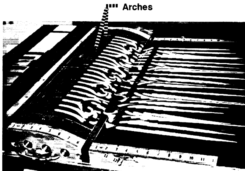
(a) Arches at 2\delta upstream of baseline separation.
