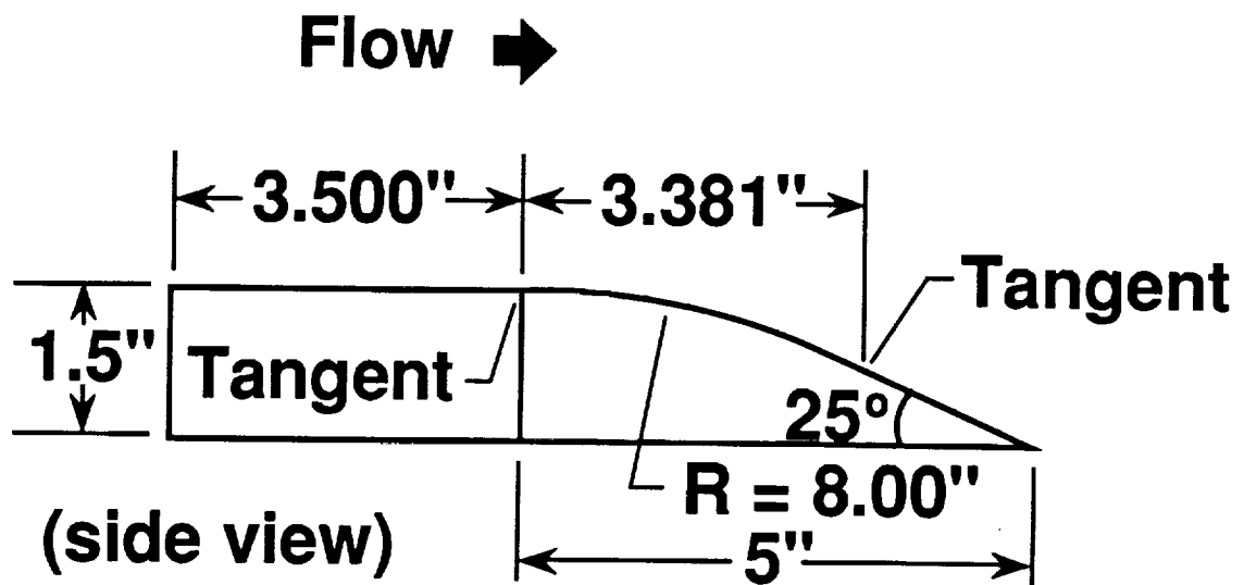
(a) Geometry of model ramp.
