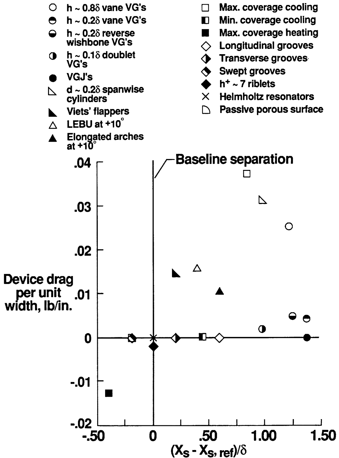
Figure 4.58 Summary of device aerodynamic drag versus separation control effectiveness.
