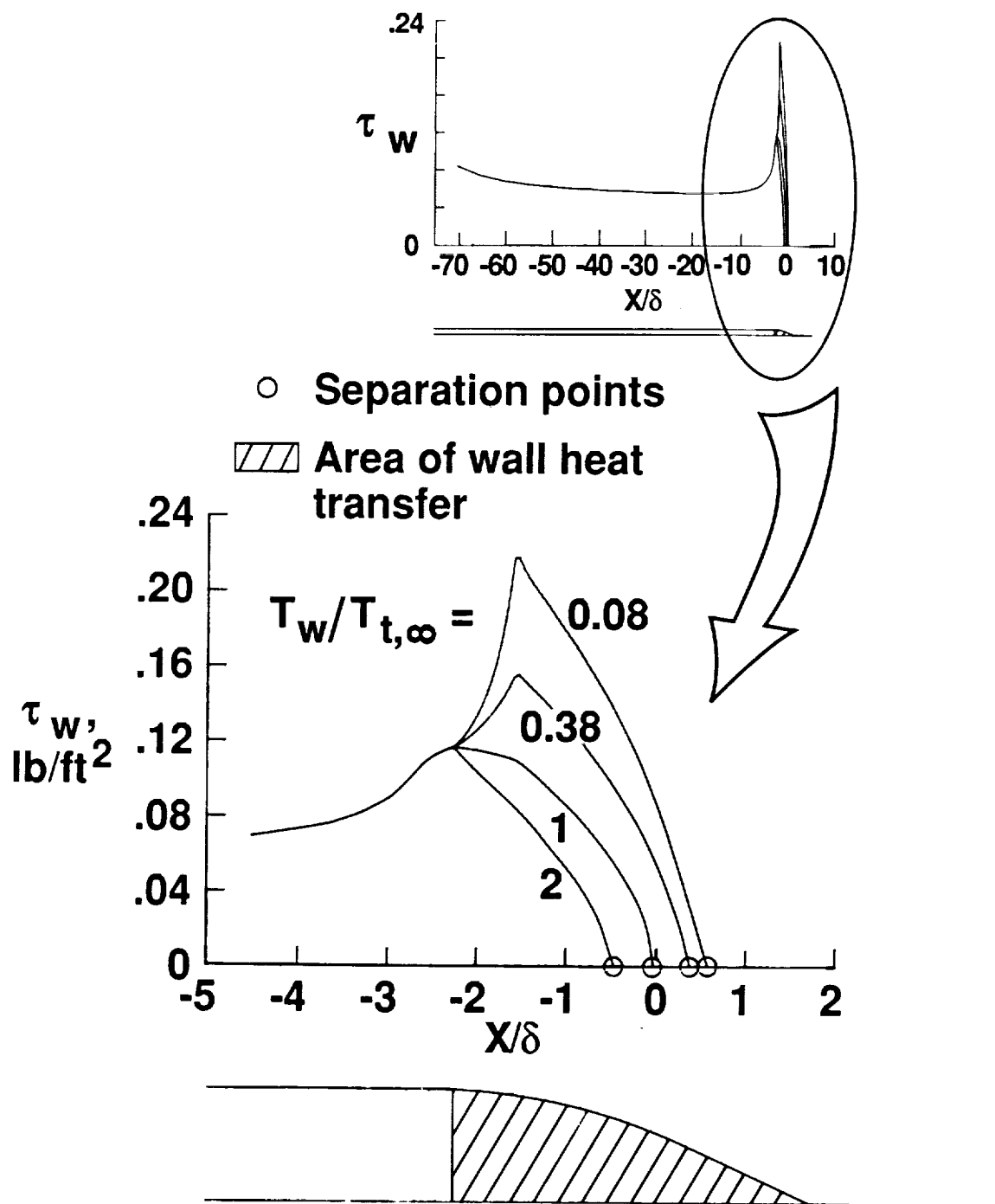
(b) Partial surface coverage from 2\delta upstream of the adiabatic reference separation.
