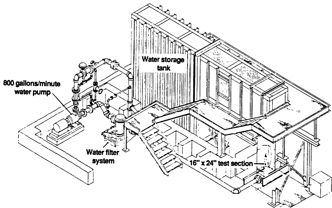
(a) Sketch of water tunnel.
