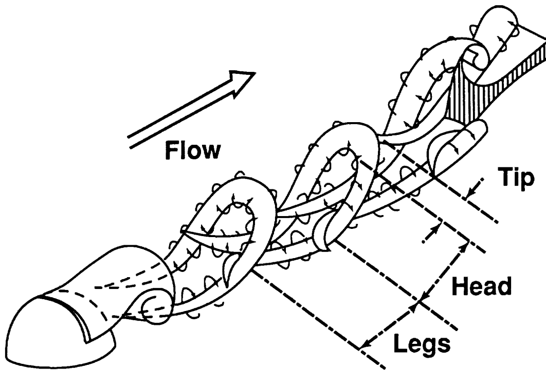
(a) By a hemisphere (Acarlar and Smith [92]).
