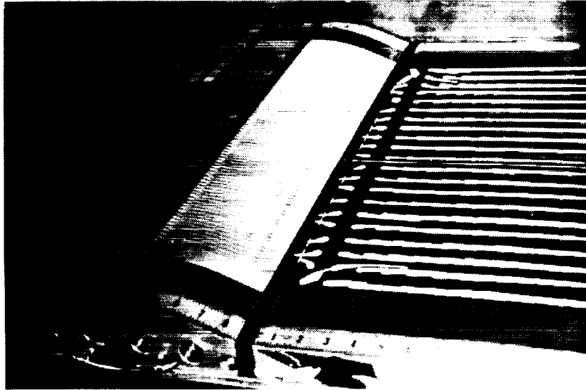
(a) 0^\circ swept (longitudinal) grooves.
