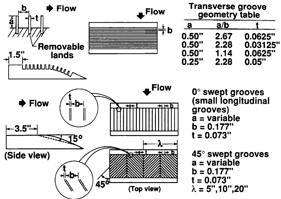
(a) Transverse and swept grooves.
