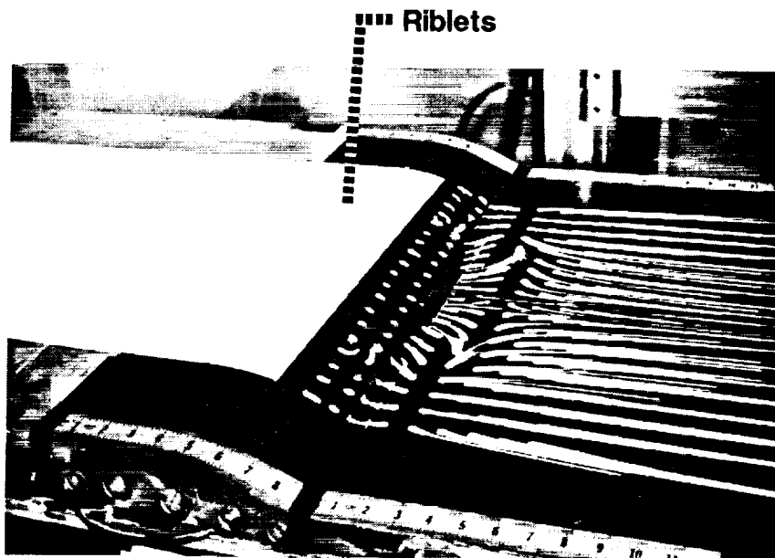
(b) 0.020-in.-high C_f -increasing riblets.
