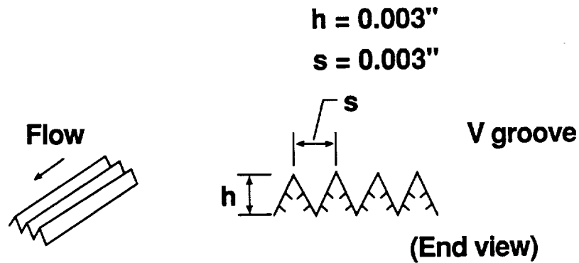
(a) Transverse and swept grooves.
