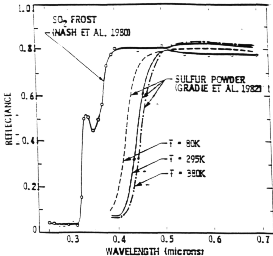
Laboratory reflectance spectra of sulfur powder and sulfur dioxide frost. Both materials have a steep absorption band edge in the ultraviolet and are otherwise bright and featureless in the visible and near infrared. The absorption edge position of sulfur is temperature sensitive, shifting to shorter wavelength as temperature decreases; at typical Io surface temperature (135 K) ordinary yellow sulfur appears white. In the ultraviolet near 0.25 to 0.30 \mu\text{m} , \text{SO}_2 frost is less reflective than sulfur by \sim 1/2 . (Nash, et al 1986)
