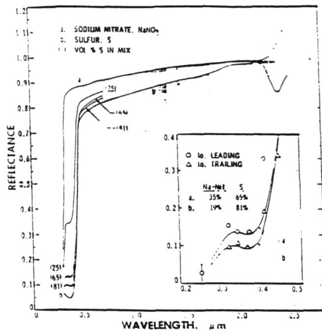
Spectra of sodium nitrate, sulfur, and mixtures. Inset shows detailed comparison of spectra of sodium nitrate/sulfur mixtures with Io data from the ultraviolet.
