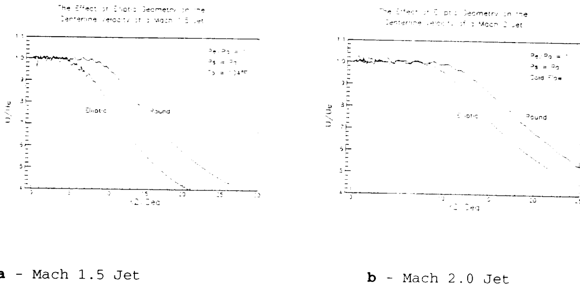
Figure 22. The effect of elliptic geometry on the centerline velocity distribution.
