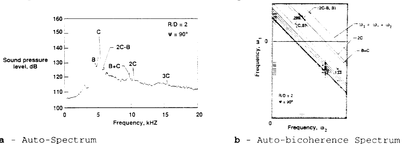
Figure 33. Spectral analysis of the acoustic emission from an unheated round conical nozzle operating at M_j = 1.44 .
