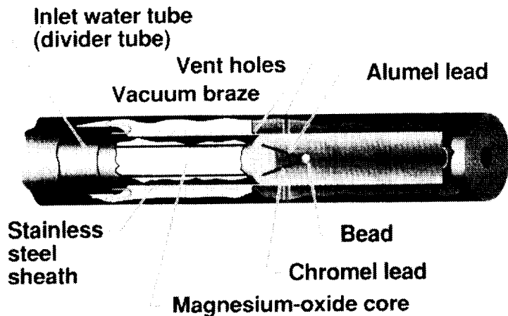
Figure 13. Cut-away view of cooled total temperature probe tip.
