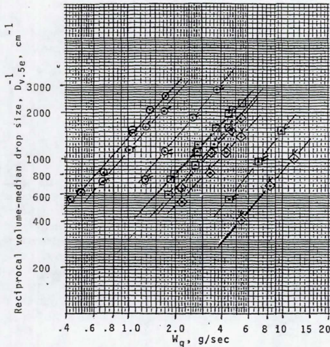
Figure 4.—Variation of experimentally determined volume-median drop size, D_{v,5e} , with atomizing-gas flowrate, W_g .
