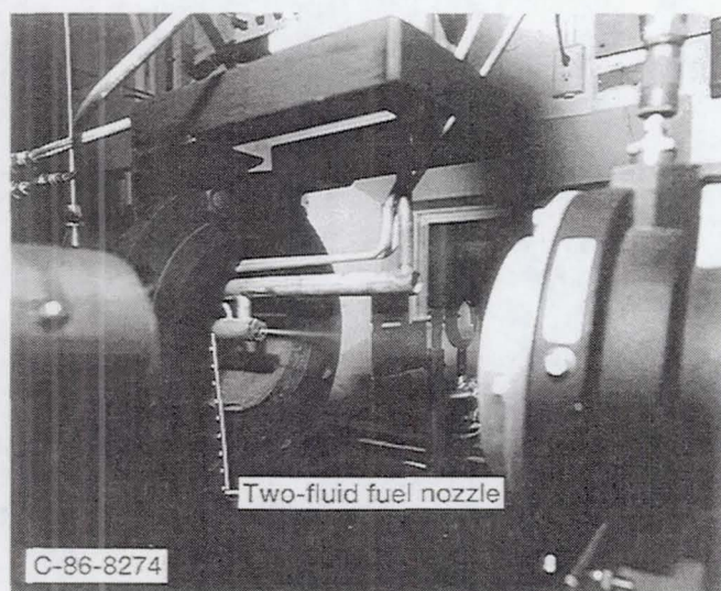
Figure 1.—Apparatus and auxiliary equipment.
