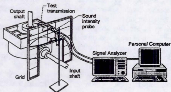
Fig 4. Sound intensity measurement system.
