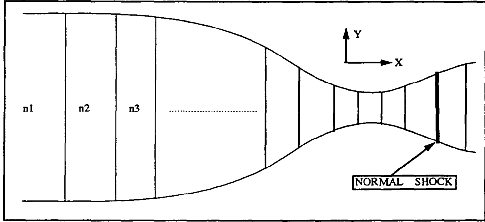
Figure 3: Discretization of the refractive index within the nozzle.
