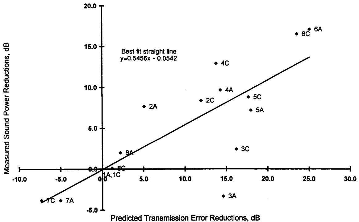
Fig. 14. Comparison of Predicted Transmission Error with Measured Sound Power Levels for the Mesh Frequency Harmonic at 5000 rpm (Data Reported as Reductions from Baseline Spur Gear set).
