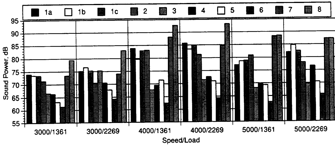
Fig. 2. Summary of the Sound Power at Twice Mesh Frequency (Including Two Adjacent Sideband Pairs) for Each of the Test Gear Pairs
