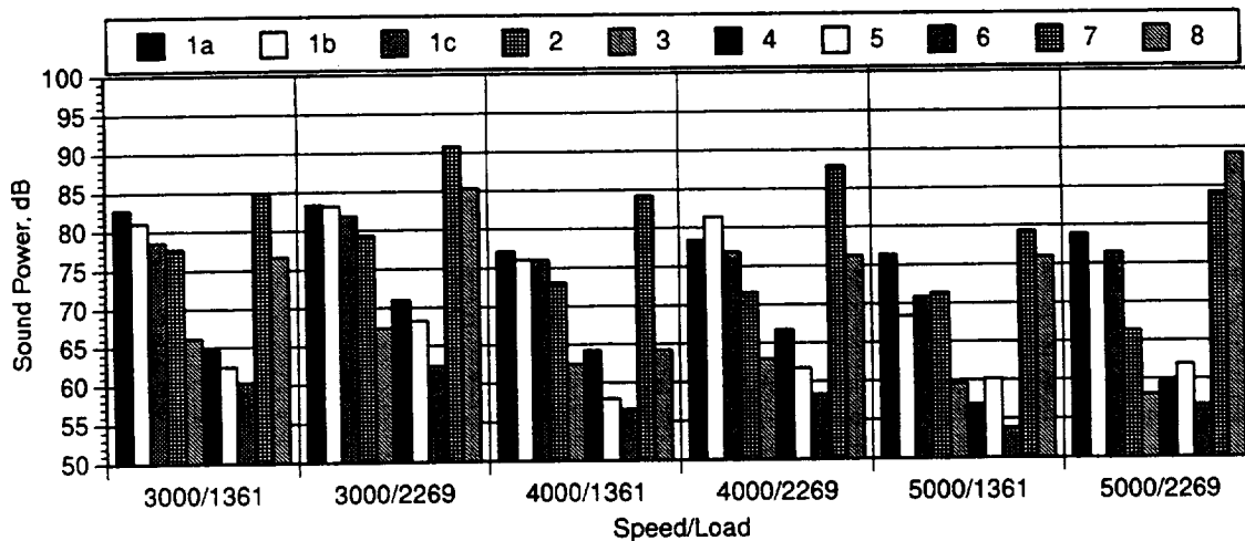
Fig. 3. Summary of the Sound Power at Three Times Mesh Frequency (Including Two Adjacent Sideband Pairs) for Each of the Test Gear Pairs
