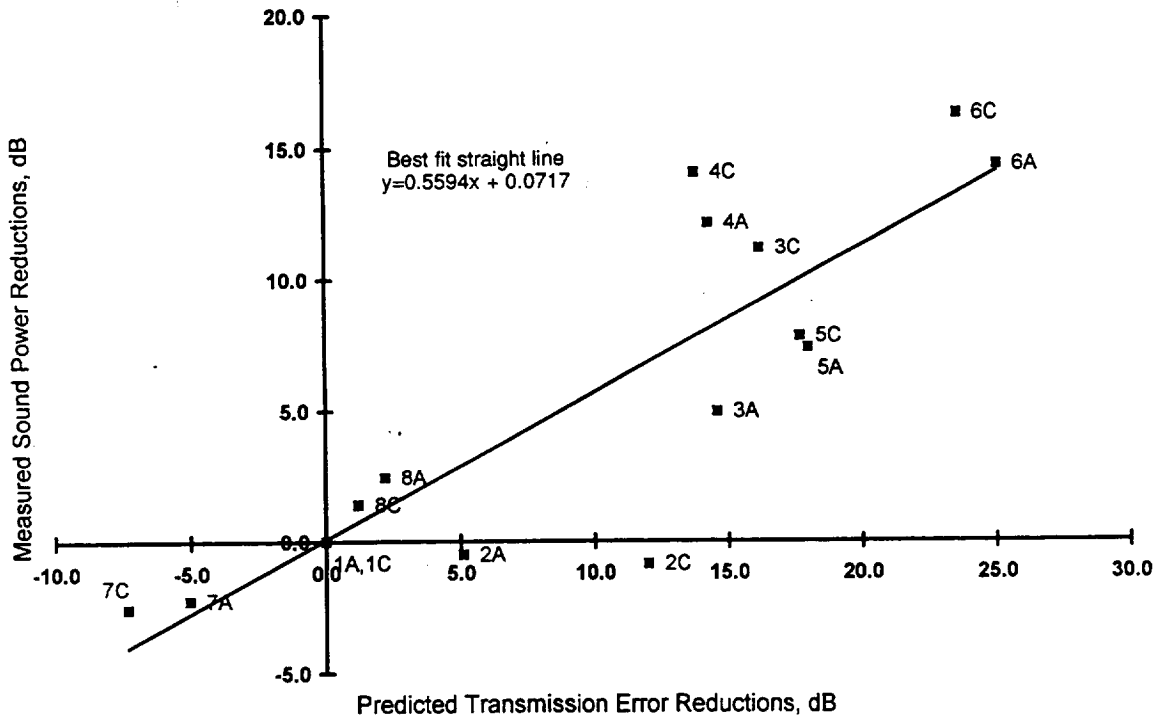
Fig. 12. Comparison of Predicted Transmission Error with Measured Sound Power Levels for the Mesh Frequency Harmonic at 3000 rpm (Data Reported as Reductions from Baseline Spur Gear set).
