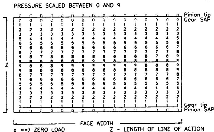
Fig. 9. Predicted Load Intensity Distribution for the High Contact Ratio Spur Gear Pair Operating at 2269 lbf-in.
