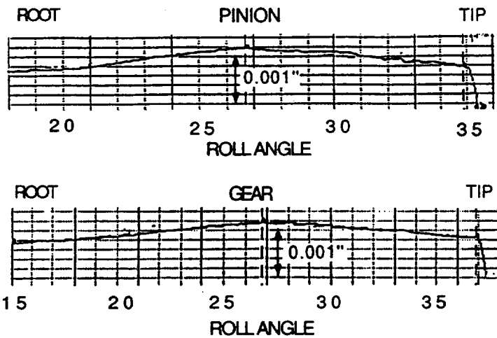
Fig. 4. Measured Profiles of the Baseline Spur Gear Pair
