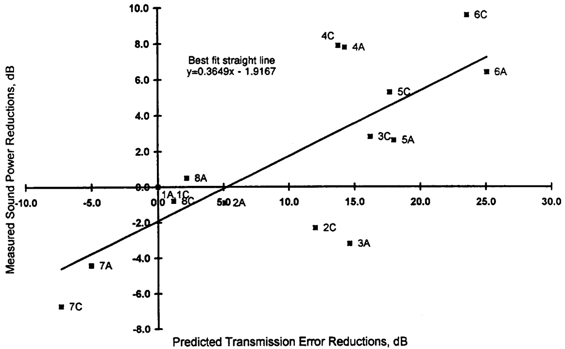
Fig. 13. Comparison of Predicted Transmission Error with Measured Sound Power Levels for the Mesh Frequency Harmonic at 4000 rpm (Data Reported as Reductions from Baseline Spur Gear set).
