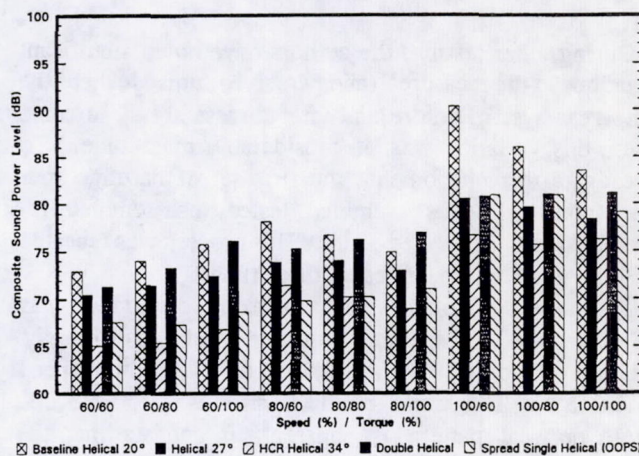
Fig. 8 - Helical gear composite noise levels
