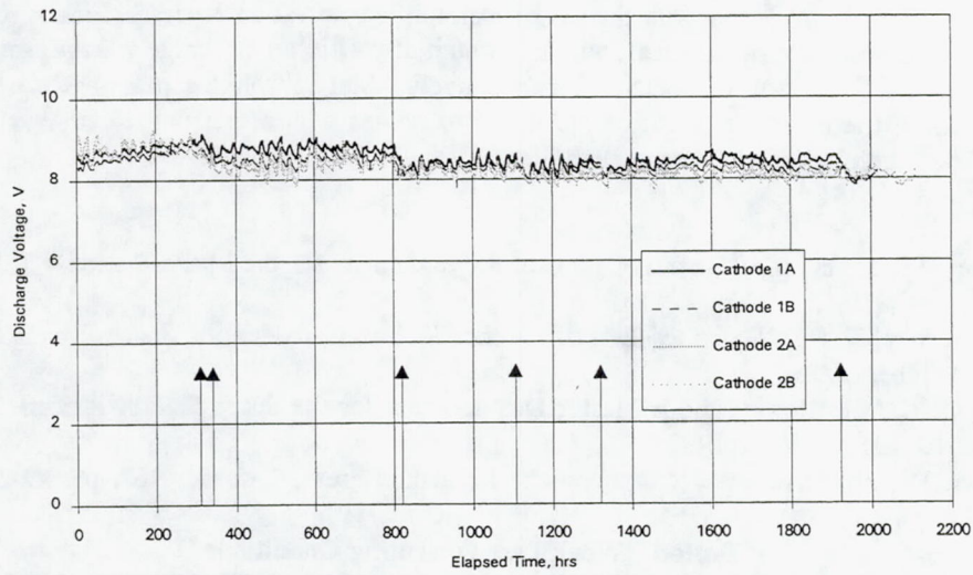
Fig. 2 Cathode Discharge Voltages (Arrows Indicate Shutdowns Due To Facility Failures or Xenon Bottle Replacements)
