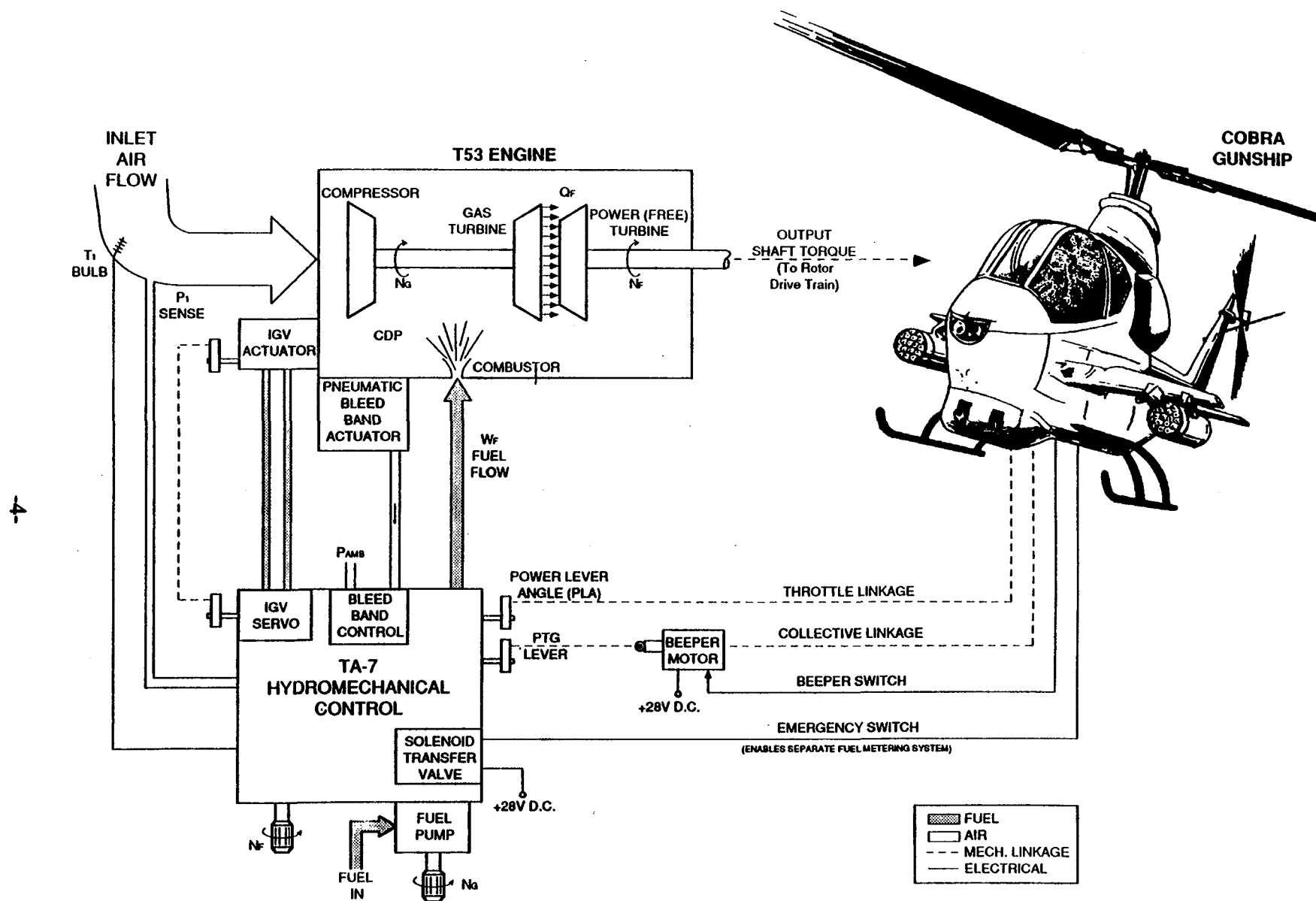
AH-1 / T53 ENGINE CONTROL SYSTEM
