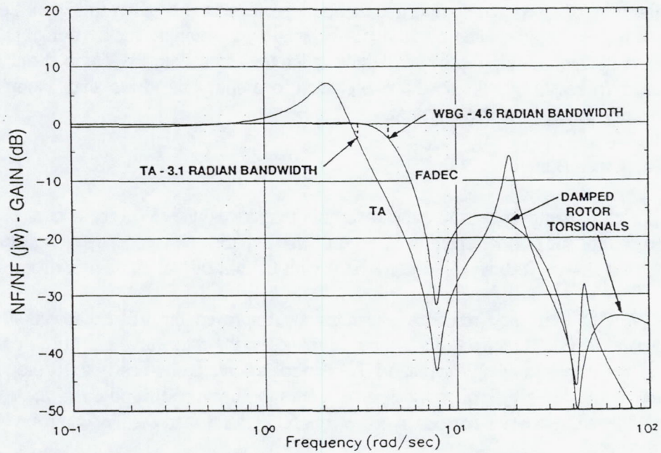
FREQUENCY RESPONSE COMPARISON OF POWER TURBINE SPEED CONTROL - NF/NF WIDEBAND GOVERNOR vs. TA CONTROL
