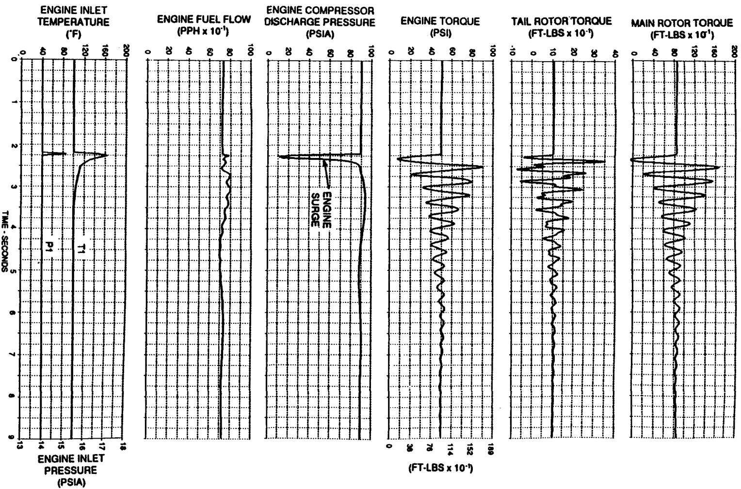
SIMULATION OF MK66 ROCKET FIRE FLIGHT TEST (1 PAIR) Figure 11
