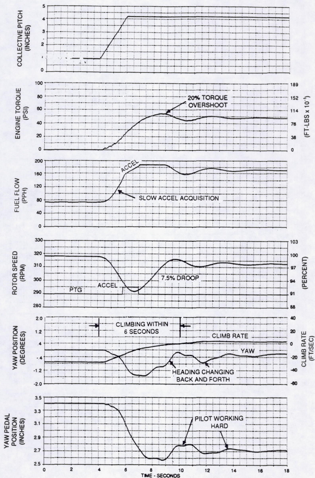
TA HYDROMECHANICAL PTG PERFORMANCE 2 Second Collective Pull from Low to High Power
