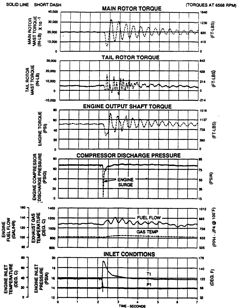
MK66 ROCKET FIRE FLIGHT TEST DATA (1 PAIR)
