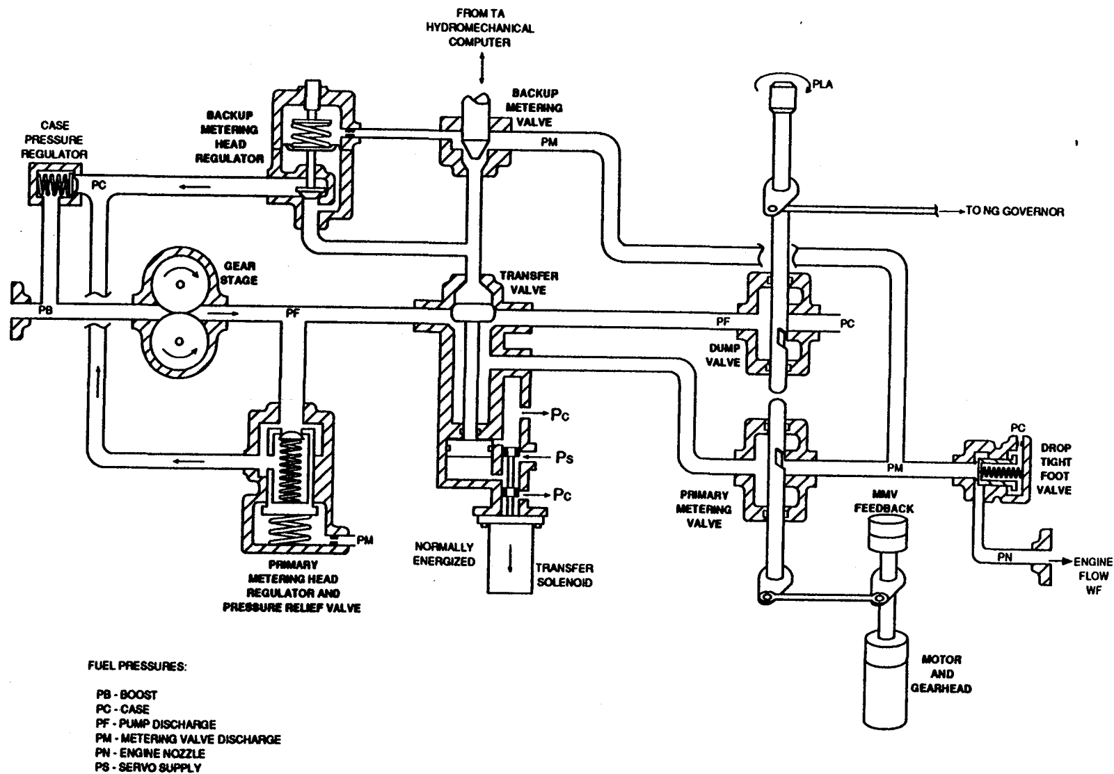
MODEL TA-7 "MODIFIED" FUEL METERING SECTION Figure 26
