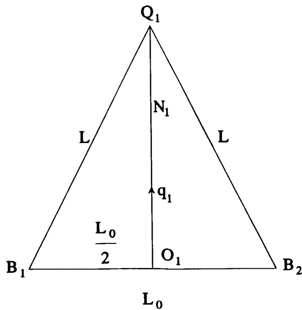
Figure B.3 Lower Cross Longerons Face Geometry
