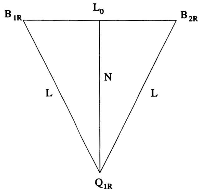
Figure B.4 Upper Cross Longerons Face Geometry
