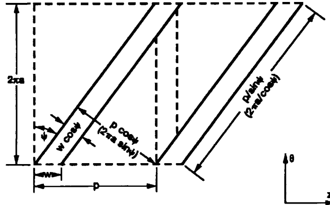
Figure 3 - The developed helix model with parameters for the equivalent helix structure.
