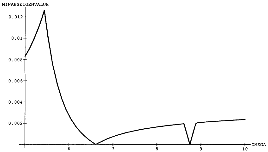
Figure 4 Minimum Absolute Eigenvalue: 86-mode Truth Model
