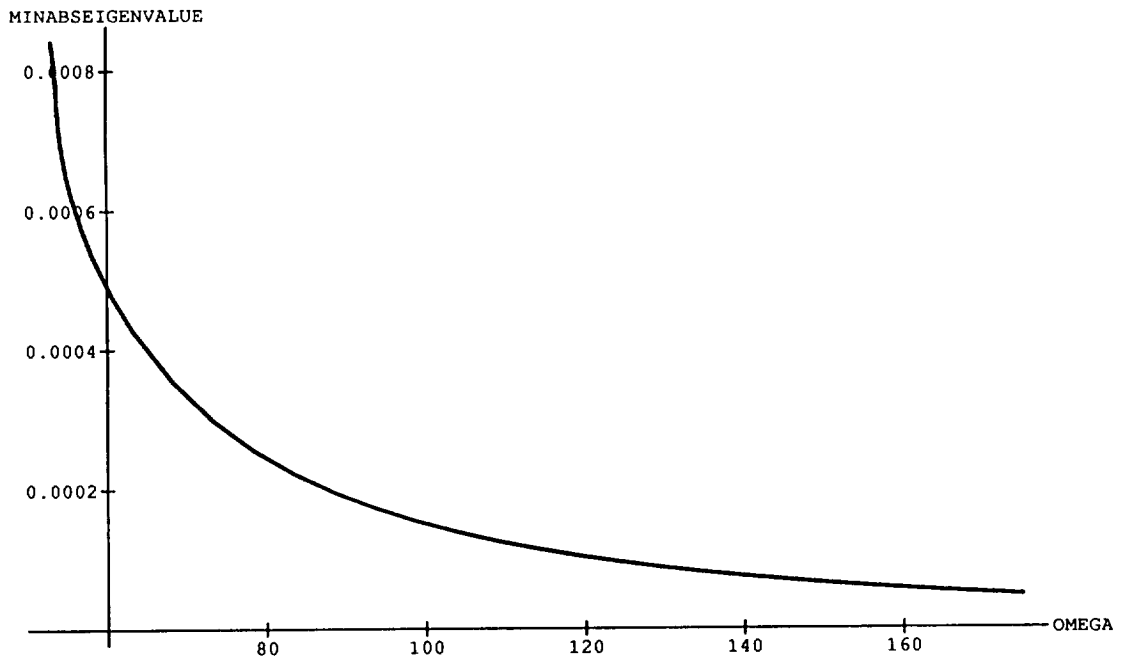
Figure 10 Minimum Absolute Eigenvalue: 86-mode Truth Model
