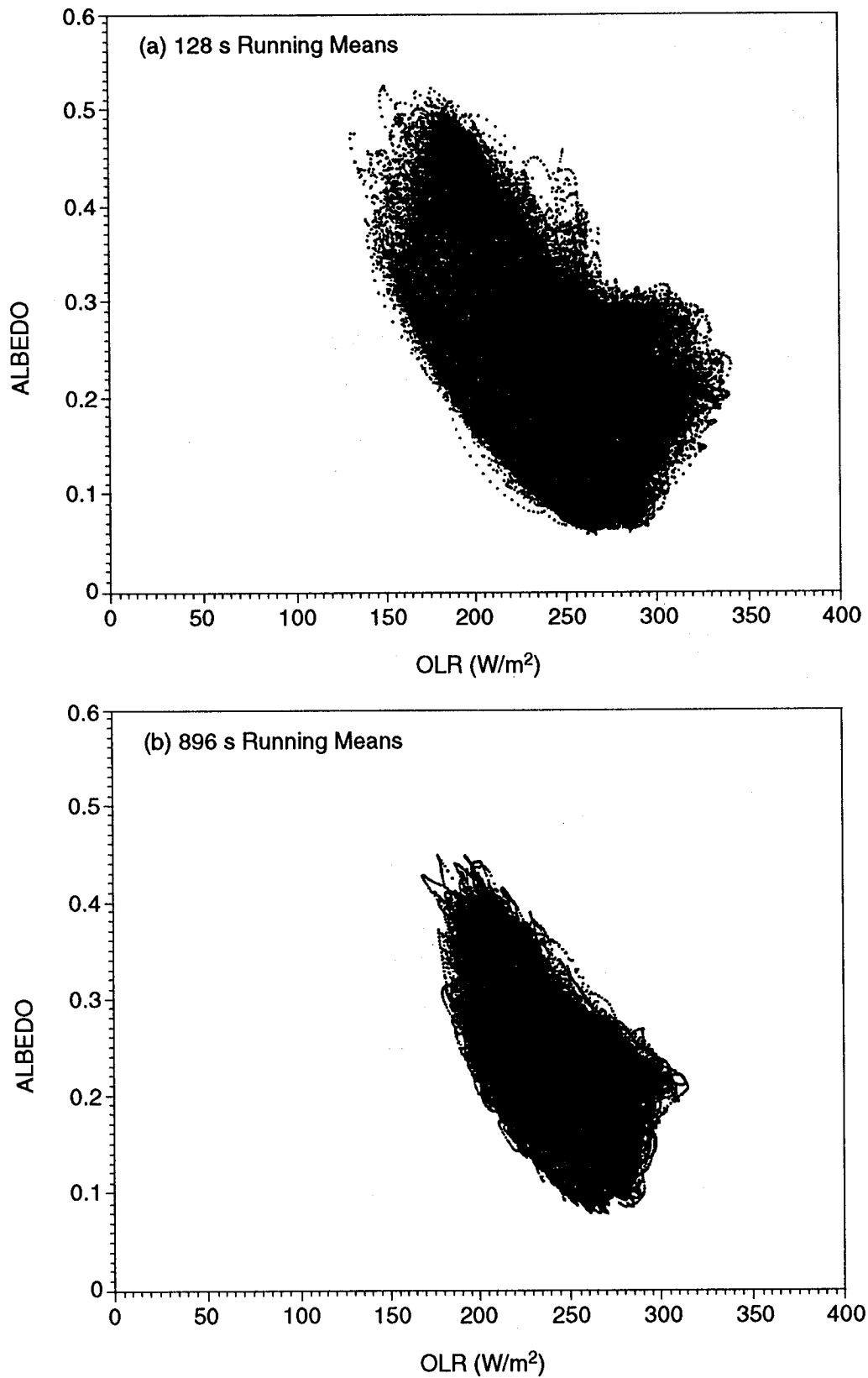
Figure 9-8. Albedo-OLR correlated pairs for 90^\circ inclination orbits (page 1 of 2).
