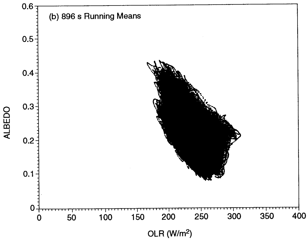
Figure 9-7. Albedo-OLR correlated pairs for 60^\circ inclination orbits (page 1 of 2).
