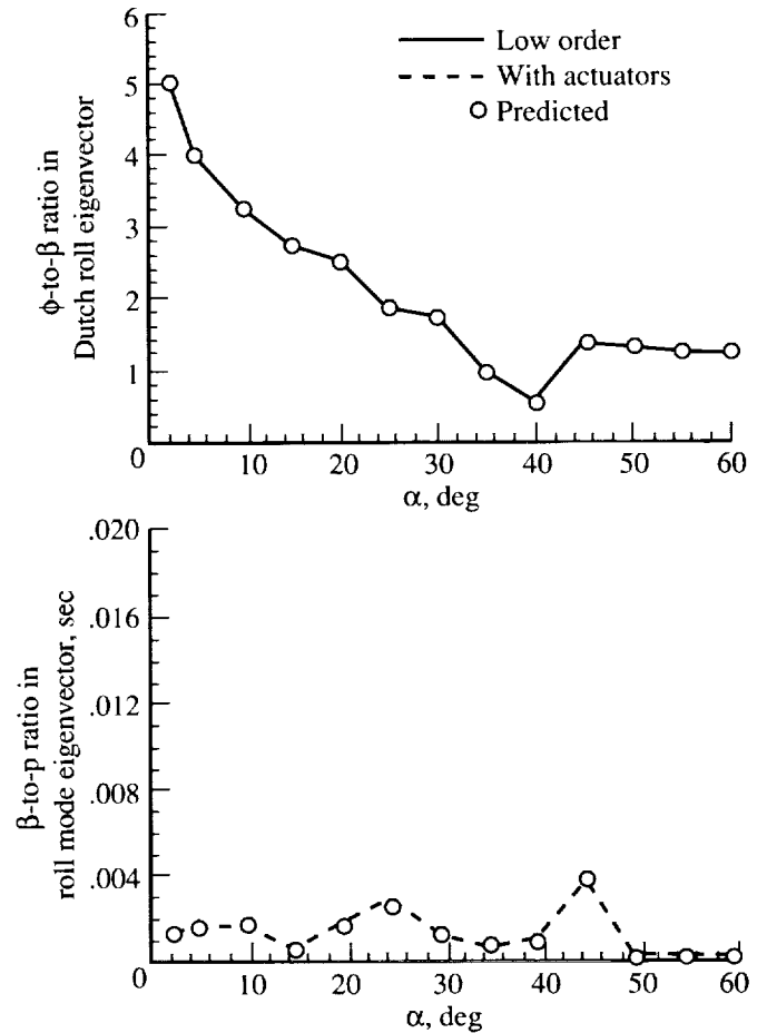
Figure 13. Eigenvector prediction with actuator models.
