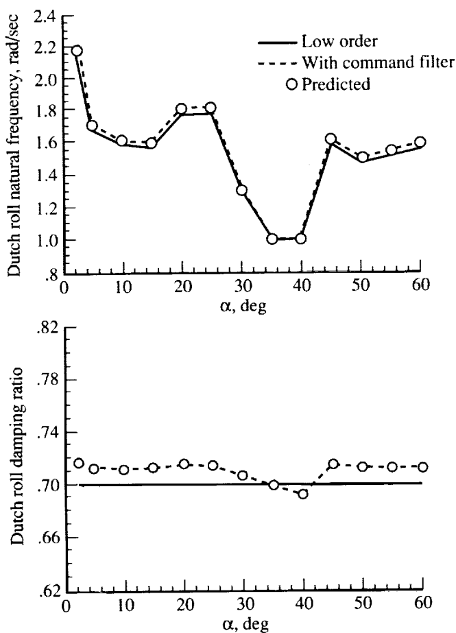
Figure 20. Dutch roll mode pole prediction with command second-order filters.
