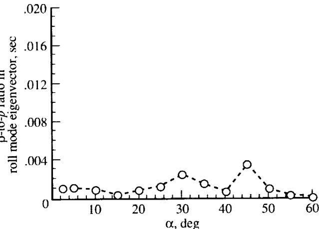
Figure 21. Eigenvector prediction with command second-order filters.
