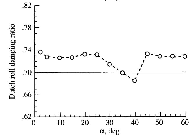
Figure 16. Dutch roll mode pole prediction with roll-off filters.
