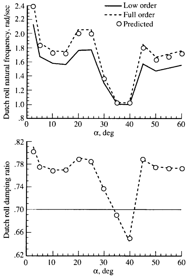
Figure 26. Dutch roll mode pole prediction with full-order model.
