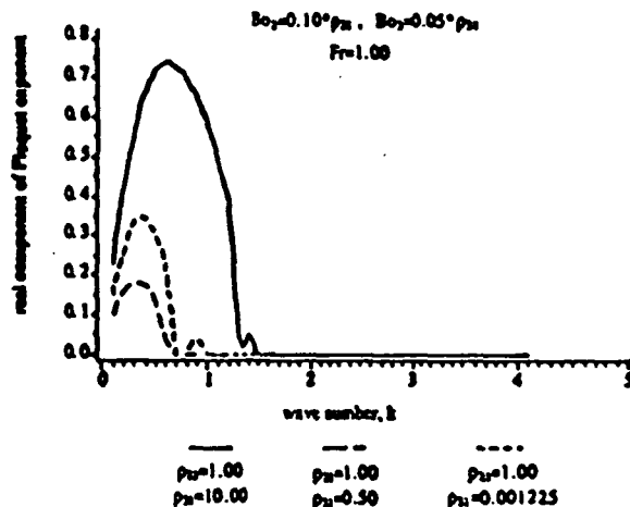
Fig. 10 Effect of density ratios on stability: Bo_2 = 0.10 \times \rho_{21} ; Bo_1 = 0.05 \times \rho_{21} ; Fr = 1.00 .
