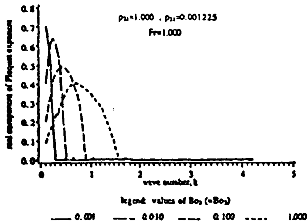
Fig. 3 Effect of Bo on stability: p_{21} = 1.00 ; p_{31} = 0.001225 ; Fr = 1.00 .
