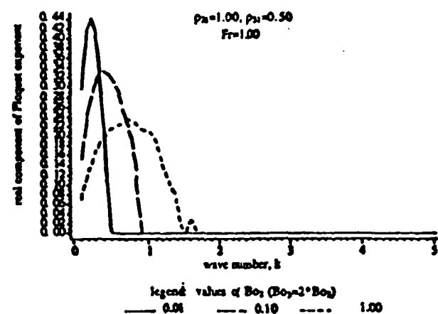
Fig. 7 Effect of Bo on stability: p_{21} = 1.00 ; p_{31} = 0.50 ; Fr = 1.00 ; Bo_2 = 2 \times (Bo_3) .
