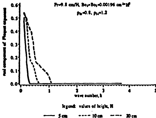
Fig. 9 Effect of height variation: Fr = 9.8 \text{ cm/H} ; Bo_2 = Bo_1 = 0.00196 \times \text{H}^2 \text{ cm}^{-2} ; \rho_{21} = 0.80 ; \rho_{22} = 1.20 .
