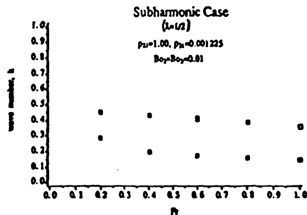
Fig. 11 Subharmonic mode at (Fr, \lambda) values for Bo_2 = Bo_1 = 0.01 ; \rho_{21} = 1.00 ; \rho_{22} = 0.001225 .
