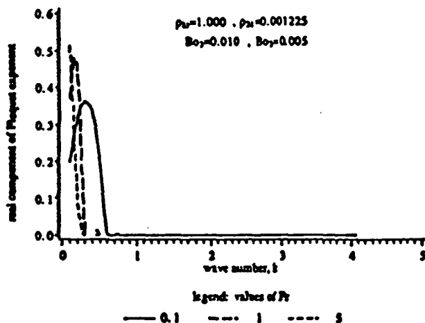
Fig. 8 Effect of Fr on stability: \rho_{21} = 1.00 ; \rho_{22} = 0.001225 ; Bo_2 = 0.01 ; Bo_1 = 0.005 .
