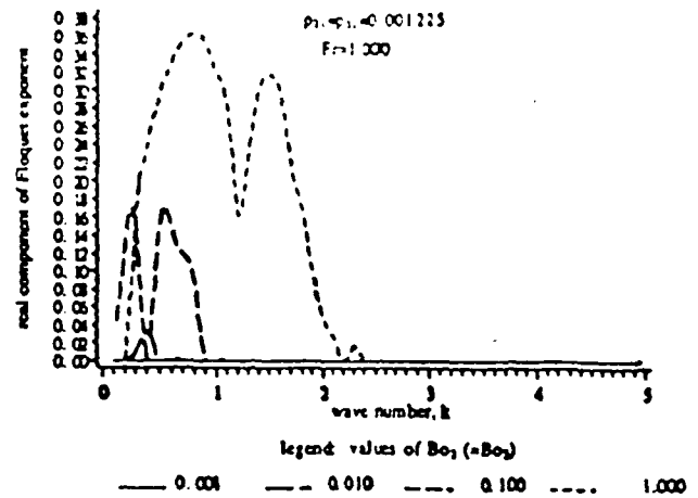
Fig. 5 Effect of Bo on stability: p_{21} = p_{31} = 0.001225 ; Fr = 1.00 .
