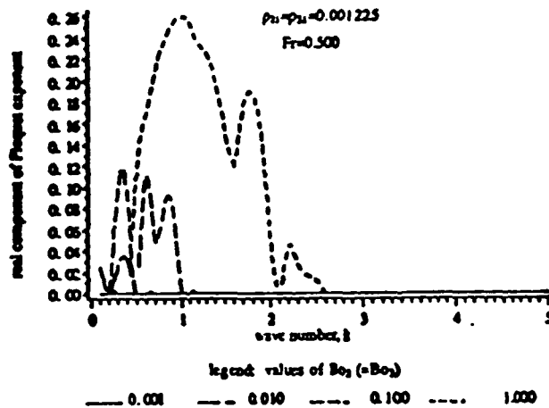
Fig. 4 Effect of Bo on stability: p_{21} = p_{31} = 0.001225 ; Fr = 0.50 .
