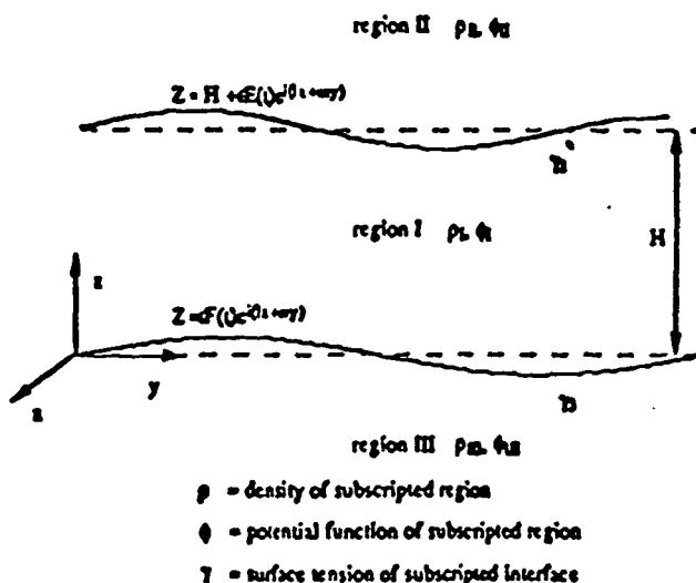
Fig. 1 Multilayer fluid configuration geometry schematic.
