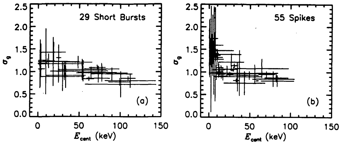
Fig. 1 (a and b). 1a shows a plot of the best-fit model parameters, along with their uncertainties, for the short-duration bursts. 1b shows the same information for the short spikes within the long-duration bursts.
