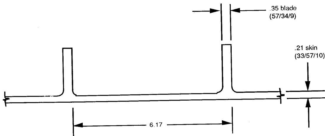
Figure 6, Optimized Upper Cover Cross Section For Modular Wing Box Concept.
