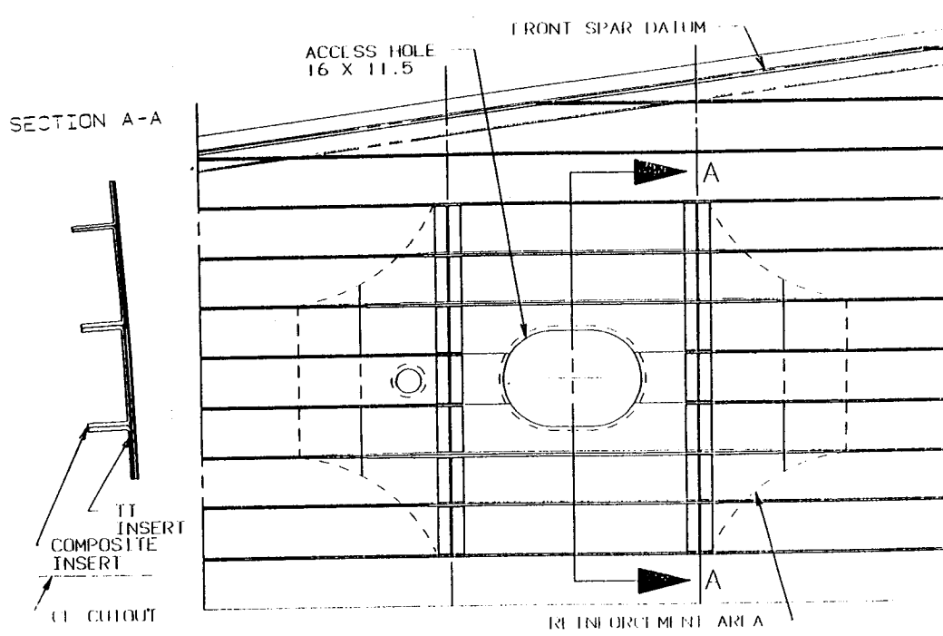
Figure 57, Cutout Concept #2.
