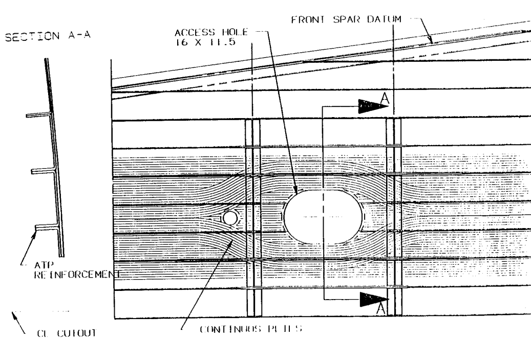
Figure 58, Cutout Concept #3.
