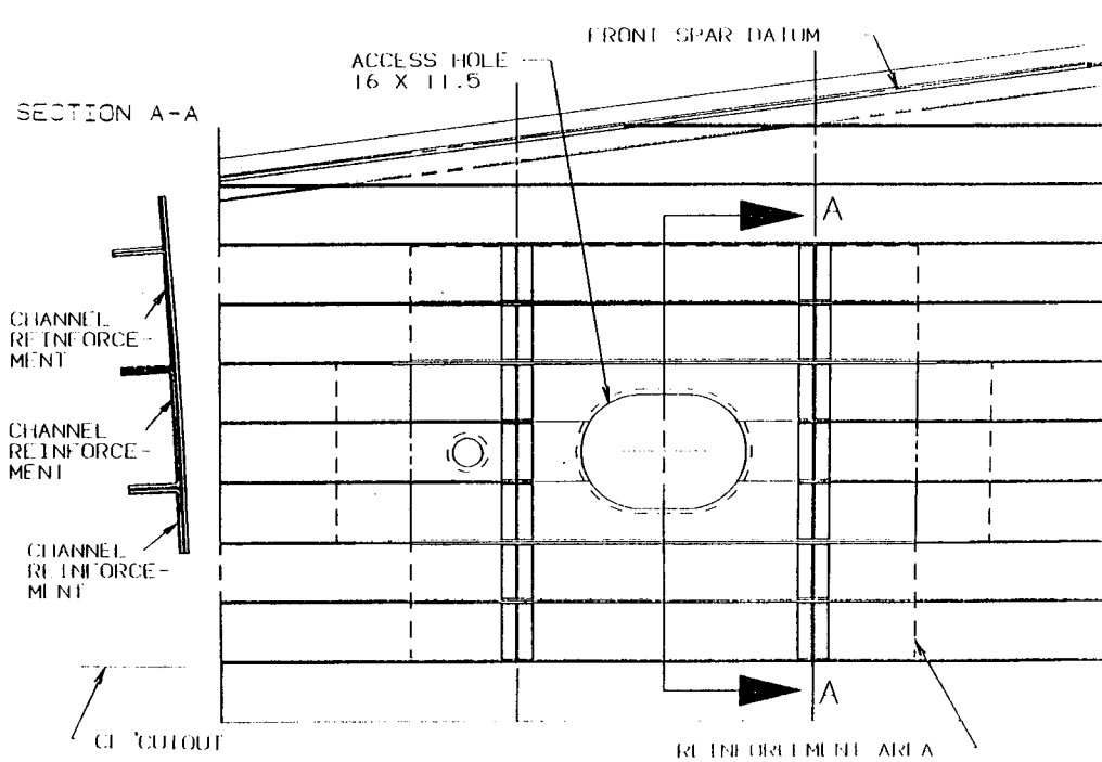
Figure 56, Cutout Concept No. 1.
