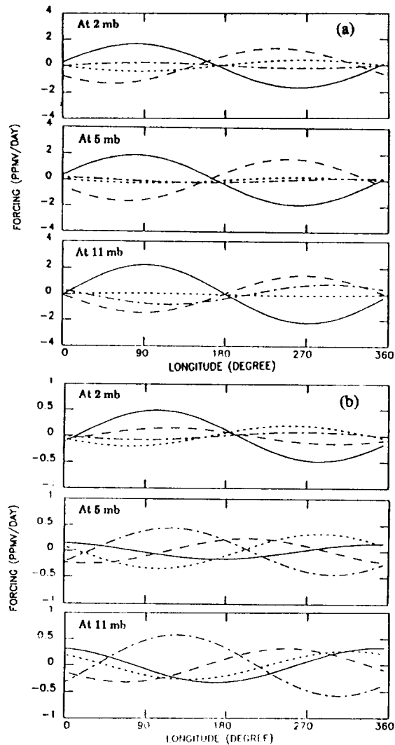
Figure 3(a) The comparison of the linear advection terms with the nonlinear advection terms for wavenumber 1 at 60^\circ N for January. The solid line denotes the linear term \bar{v} \frac{\partial \chi'}{\partial x} , the short-dashed line the nonlinear term \bar{v} \frac{\partial \chi'}{\partial x} , the long-dashed line the linear term \sqrt{\frac{\partial \bar{\chi}}{\partial y}} , the dot-dashed line the nonlinear term \sqrt{\frac{\partial \bar{\chi}}{\partial y}} .
