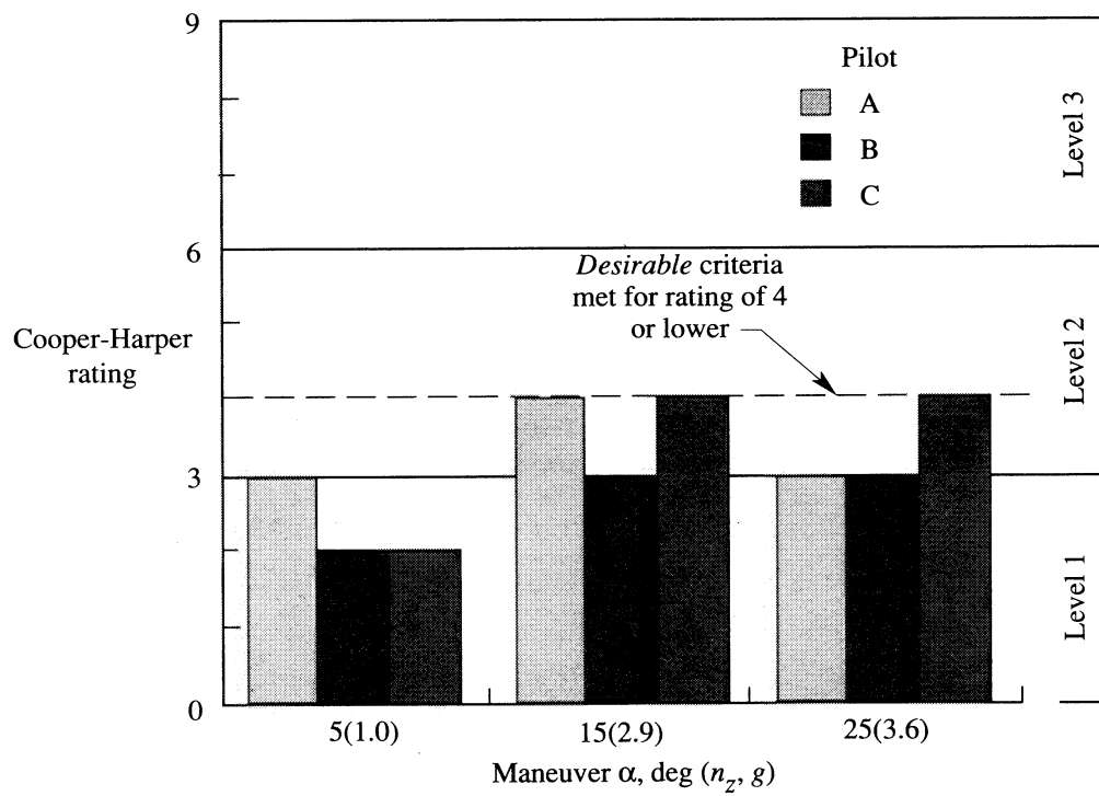
Figure 30. Angle-of-attack regulation during loaded rolls at Mach 0.6 and 25 000 ft.
