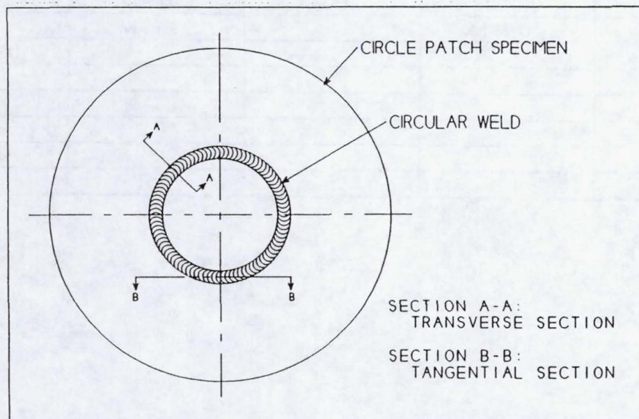
Fig. 2. Circular Weld Sectioning Techniques
