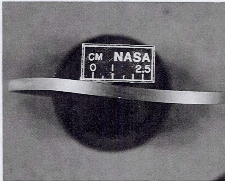
Fig. 9. Severe Warping in 16.5 cm Diameter Specimen.
