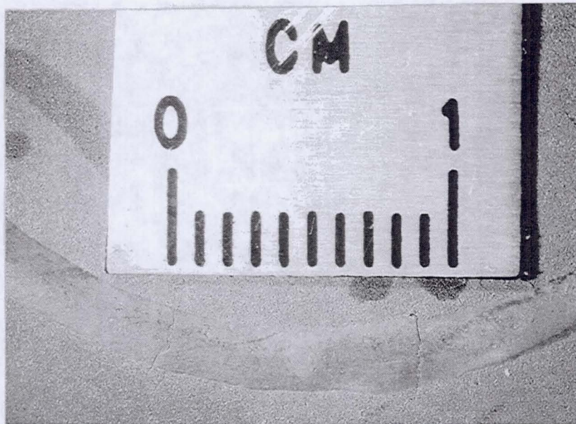
Fig. 7. Strain-age Cracking in a Welded and Solution Treated 10.2 cm Diameter Specimen.
