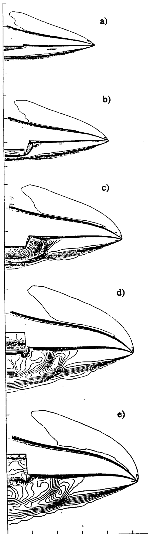
Fig. 12 CFD predicted density contours at various axial locations.
