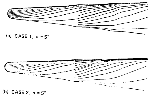
8. Computed oilflow lines a) for case 1 ( V = 5 \text{ km/s} ; Re = 10^5 ) b) for case 2 ( V = 5 \text{ km/s} ; Re = 10^6 ).
