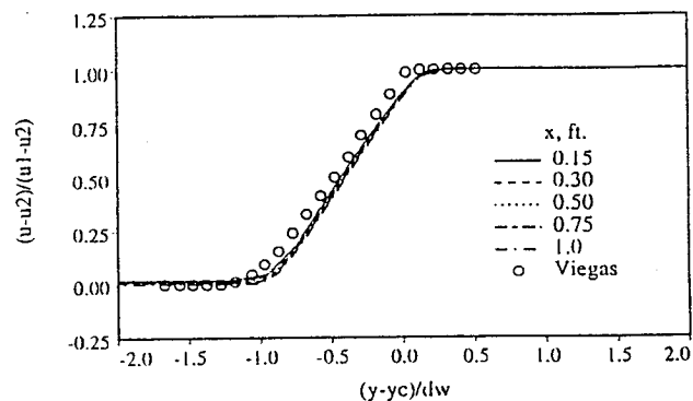
Fig. 3 Velocity profiles
