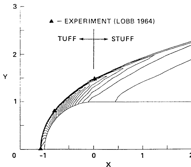
Fig. 16 Pressure Contours with Shock Standoff Comparison
