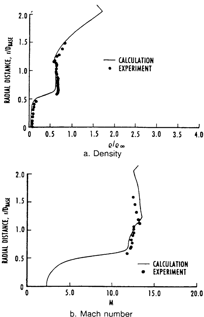
Fig. 5. Distributions across the wake at X/D = 10.0 for a sharp cone at M_\infty = 16.35 .
