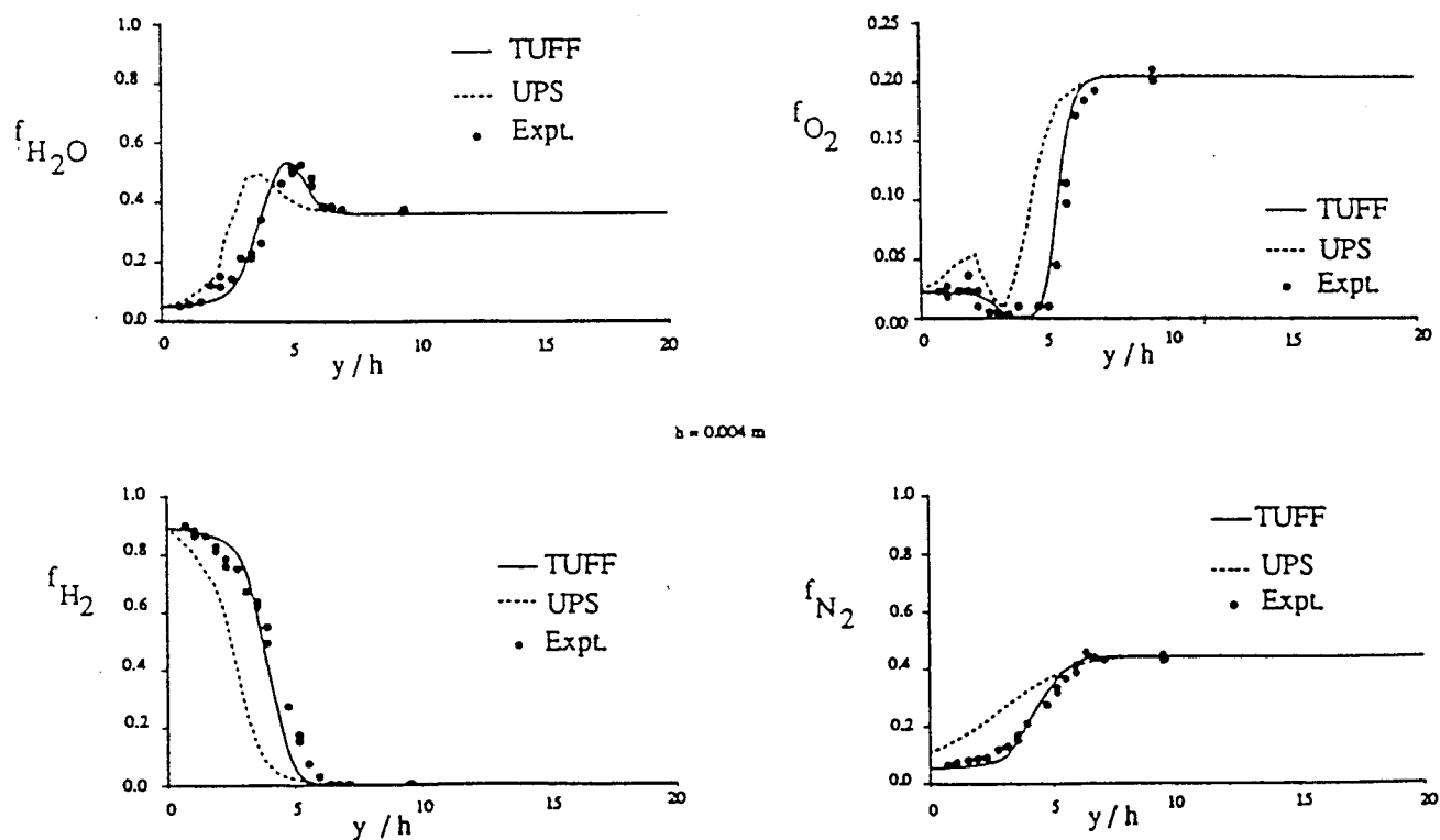
Fig. 5 Burrows-Kurkov expt. : species mole fractions at exit
