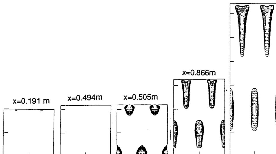
Figure 21: \text{C}_2\text{H}_4 Mass Fractions Contour at Indicated Axial Locations
