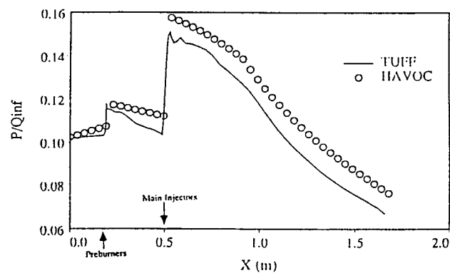
Fig. 25 Pressure as a function of axial location
