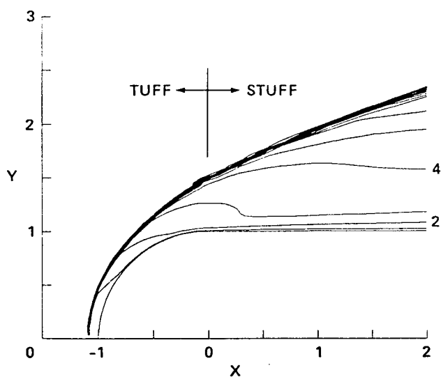
Fig. 19 Frozen Mach Number Contours
