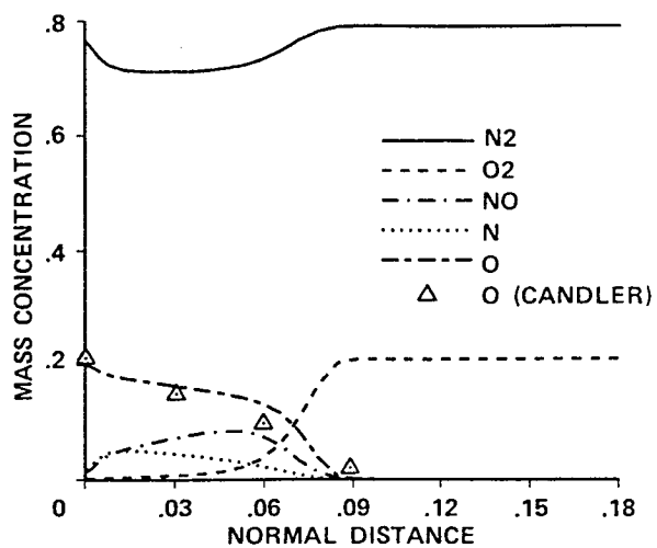
Fig. 17 Mass Concentrations on Stagnation Streamline
