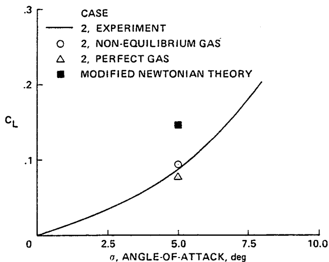
9. Experimental and computed C_L vs angle-of-attack for case 2 ( V = 5 \text{ km/s} ; Re = 10^6 ).
