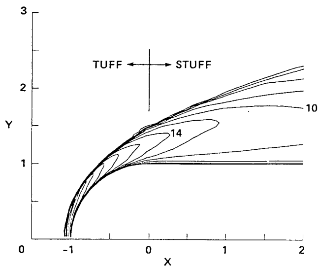
Fig. 18 Temperature Contours
