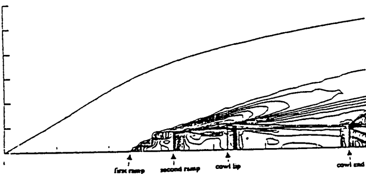
Fig. 19 CFD predicted surface pressure plot.
