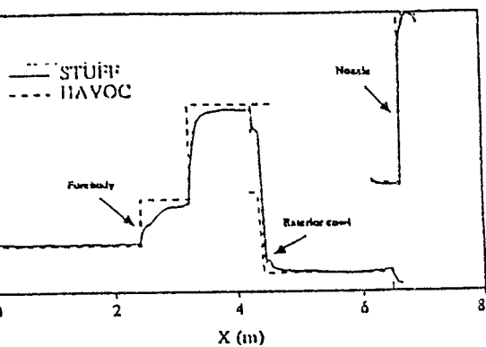
Fig. 16 Keel line pressure comparison.
