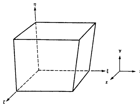
Fig. 1 Three-dimensional Finite-Volume Cell
