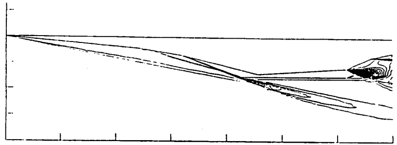
Fig. 9 CFD predicted pressure contours on vehicle symmetry plane.
