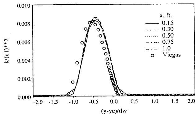
Fig. 4 Turbulent kinetic energy profiles
