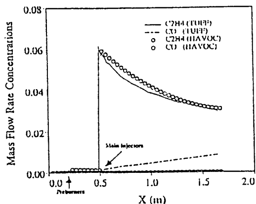
Fig. 10 C_2H_4 and CO mass concentrations as a function of axial location
