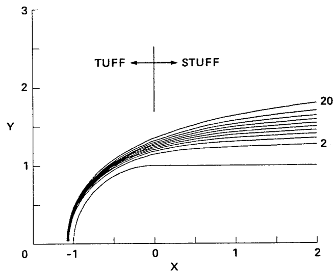
Fig. 20 Percent O_2 Mass Concentration Contours
