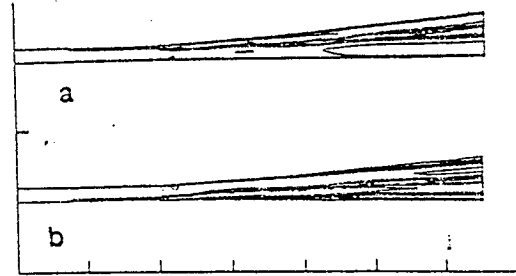
Fig. 4 Temperature contours at a) symmetry plane of top injectors, b) symmetry plane of bottom injectors.
