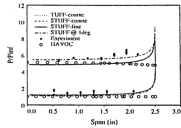
Fig. 5 Pressure comparison at x=0.156845m
