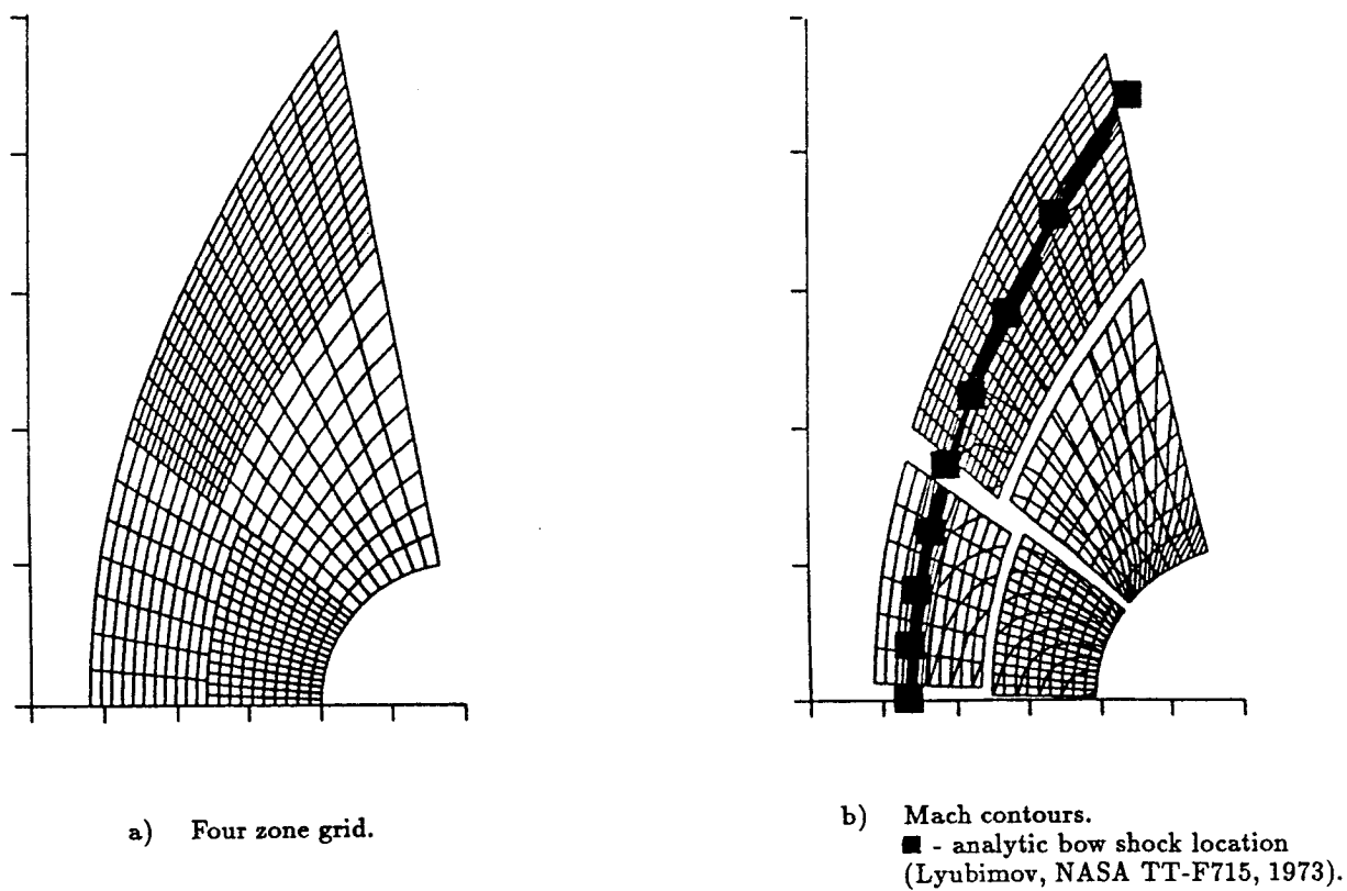
Figure 9. Axisymmetric inviscid blunt body flow at M_{\infty} = 2.0 .
