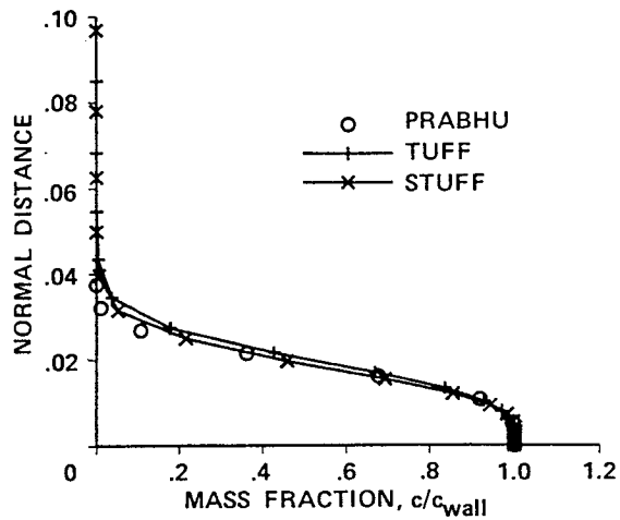
Fig. 7 O Mass Fraction Profiles at x = 3.5
