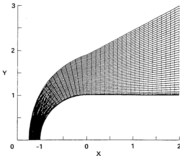
Fig. 14 Grid Used in Sphere-Cylinder Test Case
