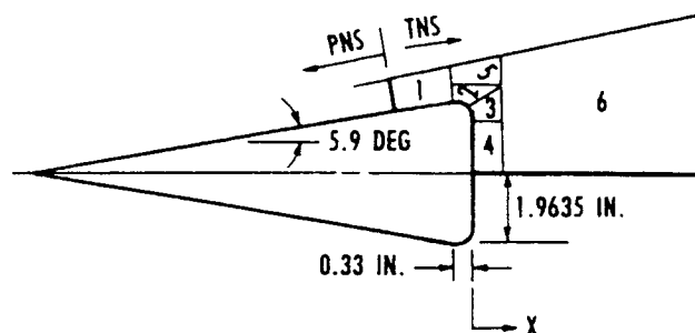
Fig. 12. 5.9-degree sharp cone geometry.
