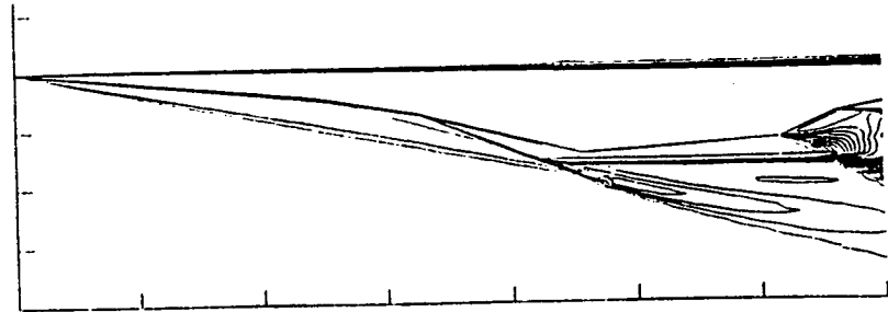
Fig. 10 CFD predicted density contours on vehicle symmetry plane.
