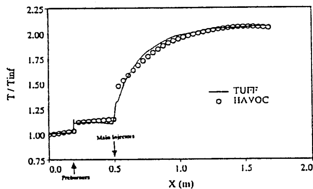
Fig. 11 Temperature as a function of axial location
