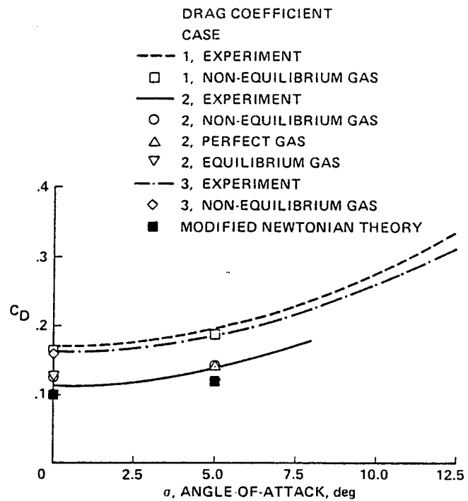
5. Experimental and computed C_D vs angle-of-attack.
