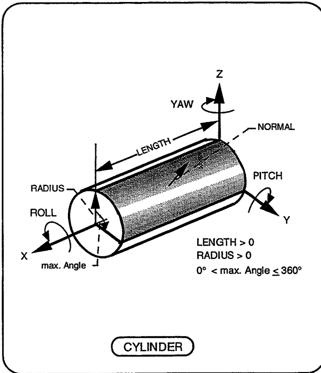
Figure 9. - Cylinder and disk surfaces primitives.
