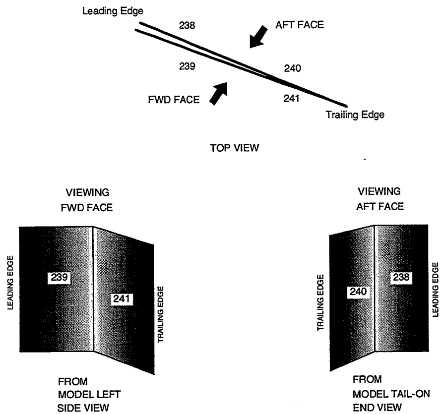
Figure 7. - Vane surface numbering sequence.
