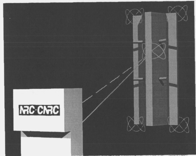
Figure 7: Real-time tracking of geometrical targets (e.g., corner or targets) using Lissajous patterns and the laser range sensor.
