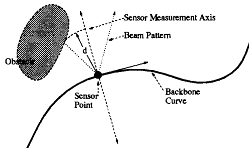
Figure 1: Simplified Distance Measurement Sensor Model
