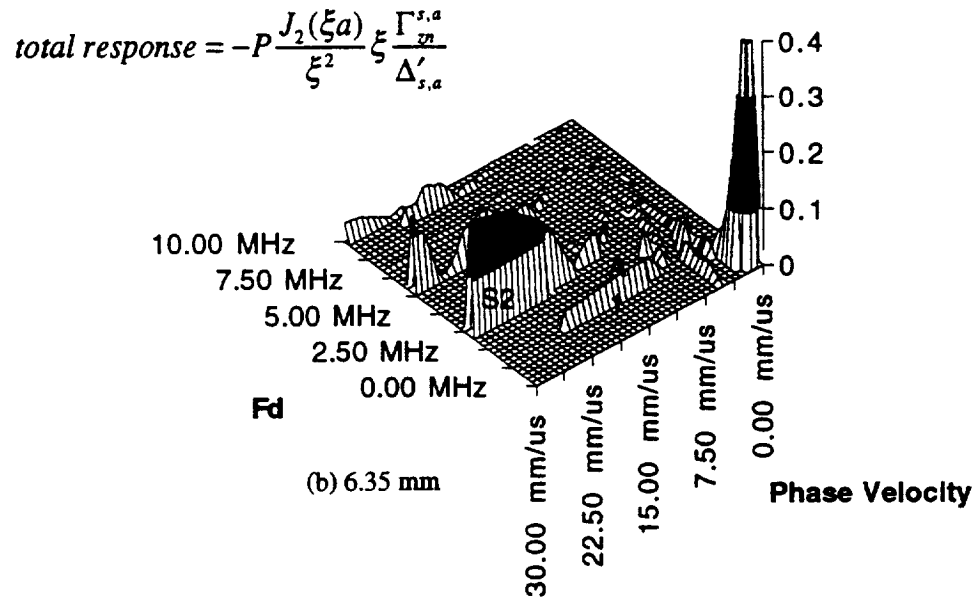
Figure 3.5 The total response (source, wavenumber, and material response) in fd-phase velocity space for (a) 0.77 mm, (b) 6.35 mm, (c) 12.7 mm, and (d) 25.4 mm parabolic source on a simulated aluminum plate.
