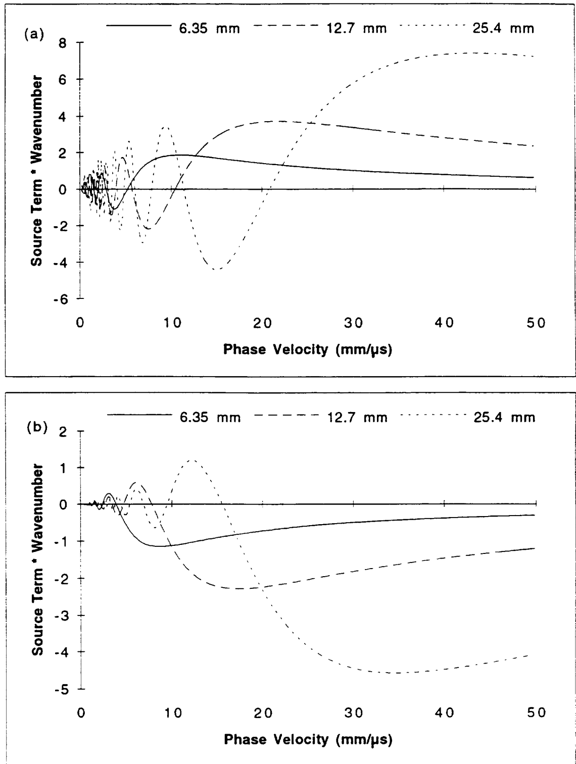
Figure 3.3 The source term multiplied by the wavenumber for three different diameter (a) PISTON (b) PARABOLIC sources, showing the "far field" phase velocity after which the term decays due to energy considerations
