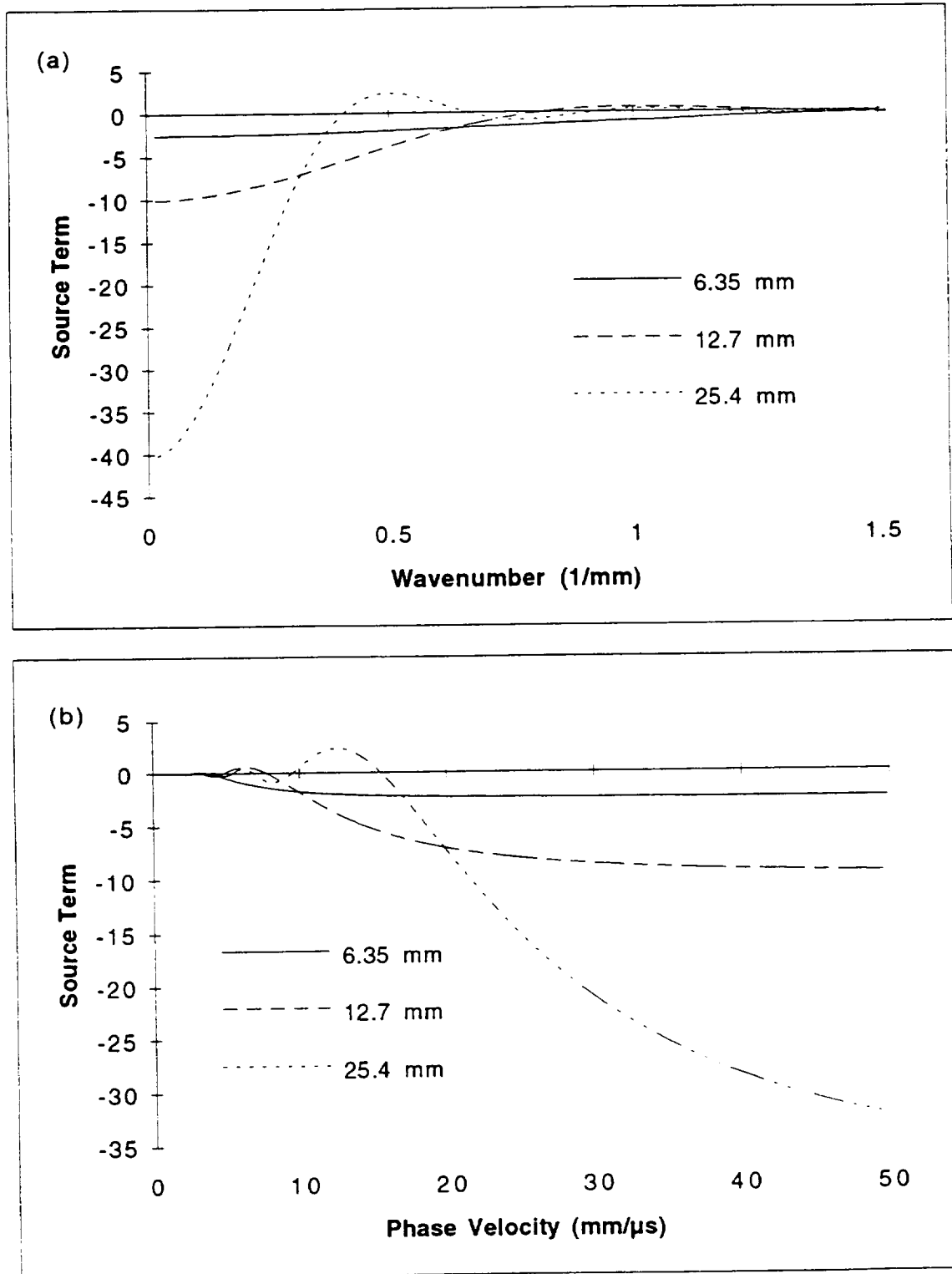
Figure 3.2 The source term for three different diameter PARABOLIC sources as a function of (a) wavenumber and (b) phase velocity, showing that normal surface loads tend to generate waves with infinite phase velocities and zero wavenumbers
