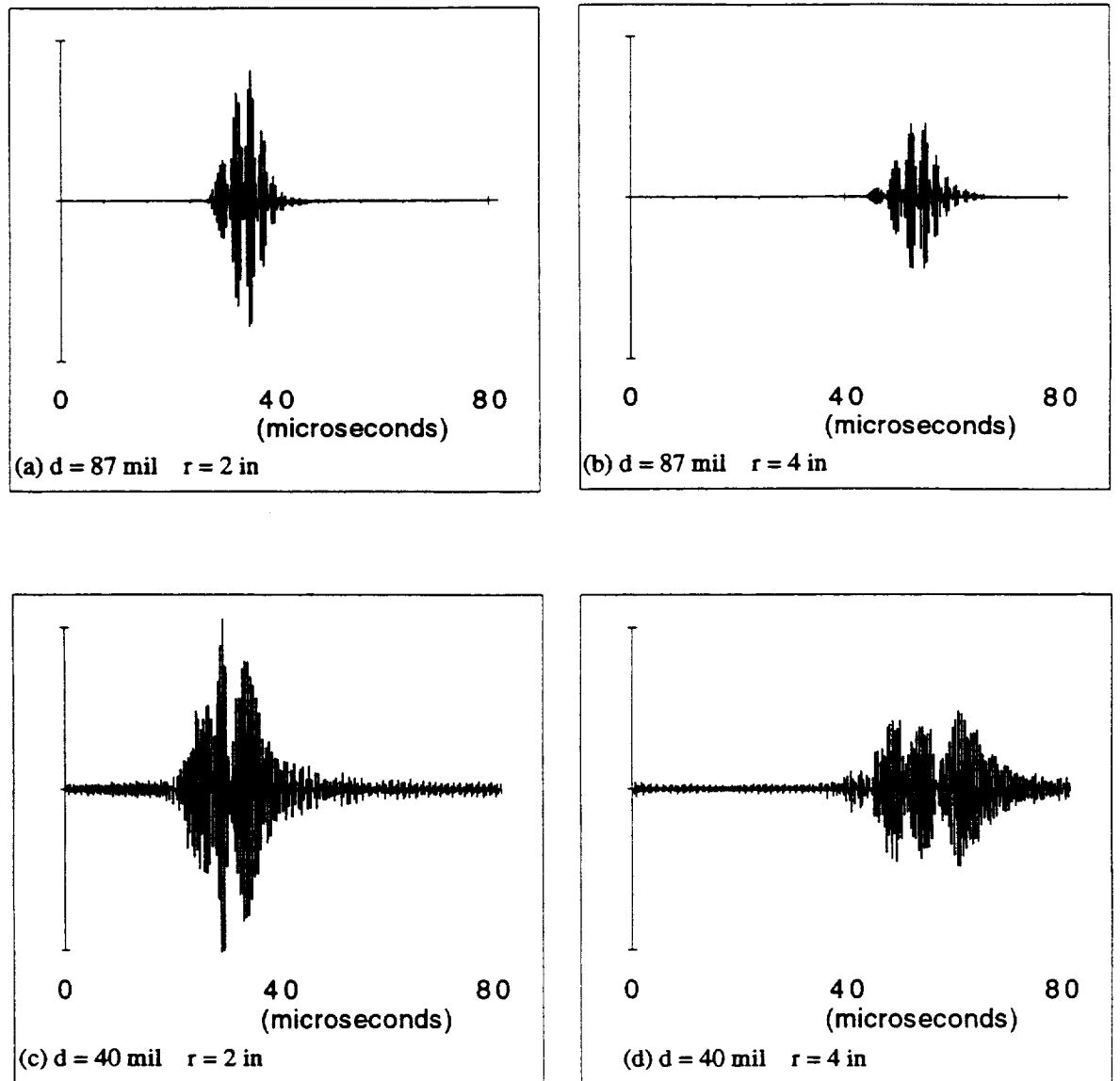
Figure 4.6 Four simulated RF waveforms created at the same fd=3.5 for two thickness plates (40 and 87 mil) and for two separation distances (2 and 4 inches). The signals were created with a half inch piston source, driven by a 20 cycle sine-modulated signal.
