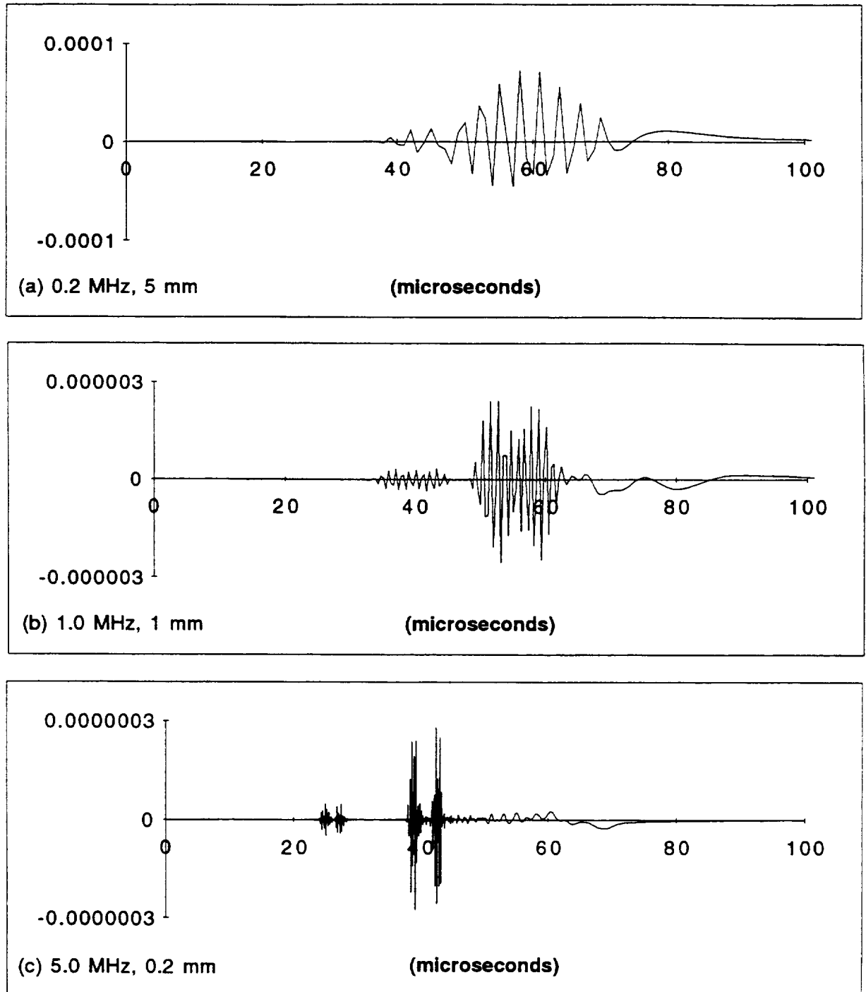
Figure 4.2 Simulated waveforms for three different thickness plates (a) 5 mm (b) 1.0 mm (c) 0.2 mm at f_d=1.0 mm-MHz. A 12.7 mm, 10 cycle sine-modulated, piston source was modeled.
