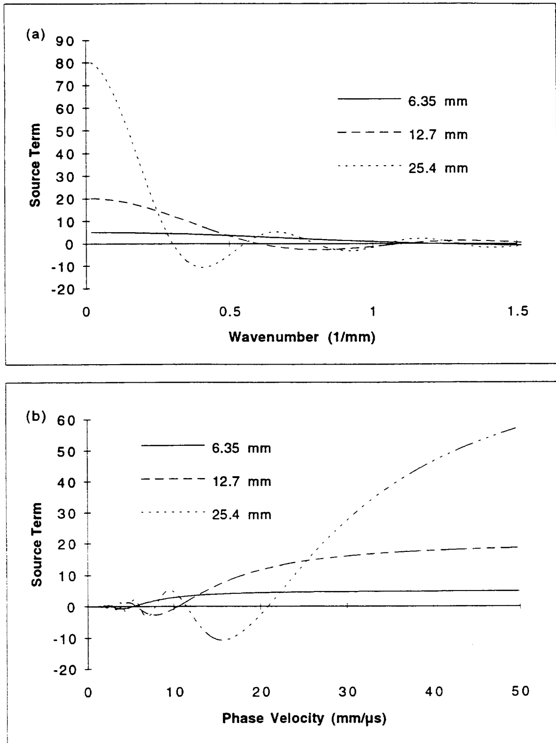
Figure 3.1 The source term for three different diameter PISTON sources as a function of (a) wavenumber and (b) phase velocity, showing that normal surface loads tend to generate waves with infinite phase velocities and zero wavenumbers
