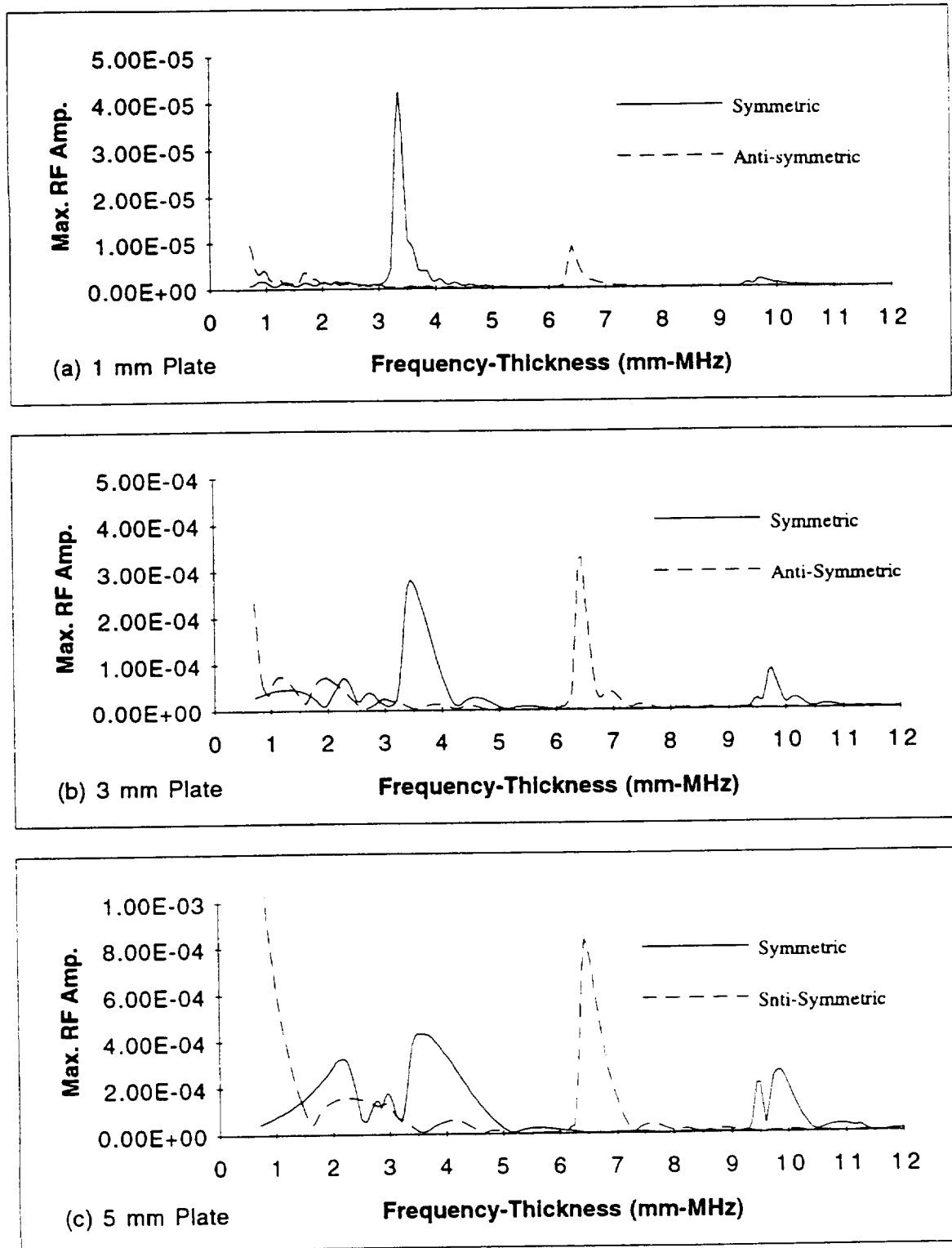
Figure 4.7 Simulated maximum RF amplitude response vs center frequency-thickness for three thickness plates, (a) 1 mm, (b) 3 mm, and (c) 5 mm. (Created for a 12.7 mm parabolic source on an aluminum plate.)
