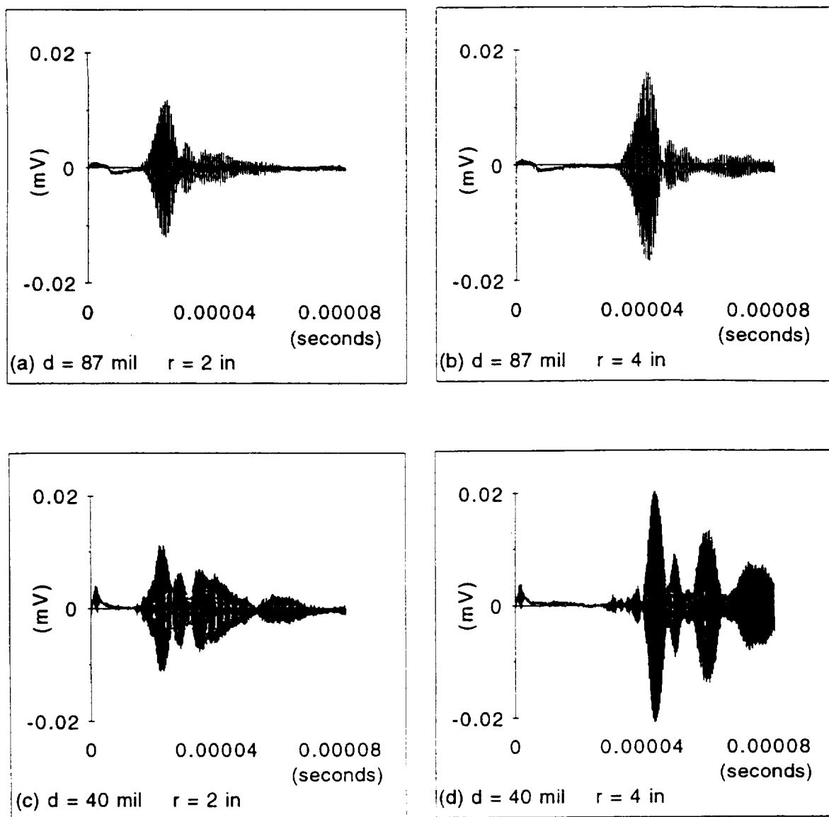
Figure 4.4 Four experimental RF waveforms taken at the same Fd = 3.5 mm-MHz on two thickness plates (40 and 87 mil) and at two separation distances (2 and 4 inches).
