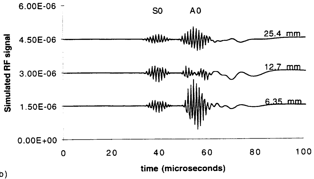
Figure 3.7 The (a) simulated frequency response and (b) simulated RF signal for three different size parabolic sources on a 1 mm Al plate at fd=1.0 . The amplitude of the RF signal from the 6.35 mm source is greater than the signal from the larger sources because the smaller transducer is able to excite lower phase velocities and therefore "reach down" to the fundamental modes. There is also a change in the ratio of the modes as the size of transducer is changed.
