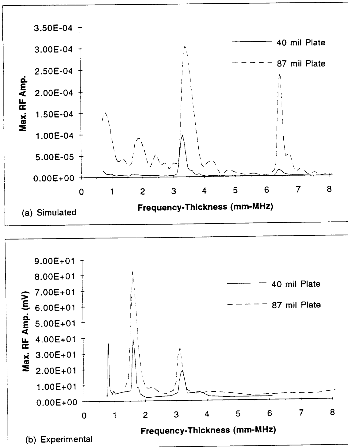
Figure 4.8 The (a) simulated and (b) experimental maximum RF amplitude profiles for two plate thicknesses (for a 12.7 mm parabolic source, 10 cycle sine-modulated signal, sampled two inches from the center of the transmitting transducer on an aluminum plate).
