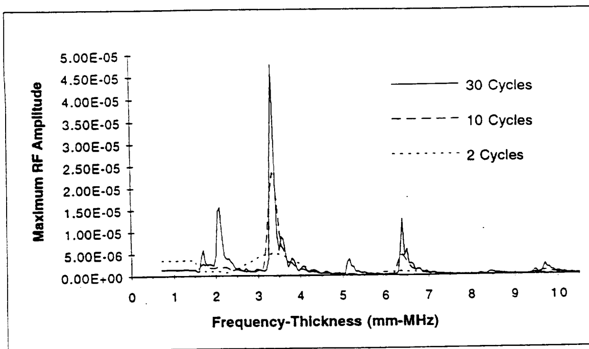
Figure 2.8 Simulated maximum RF amplitude vs center frequency-thickness for a sine-modulated signal consisting of 2, 10, and 30 cycles, propagating in a 1 mm Al plate. A longer wave packet has a narrower frequency bandwidth associated with it. As a result, modes are only generated near their cutoff frequencies.
