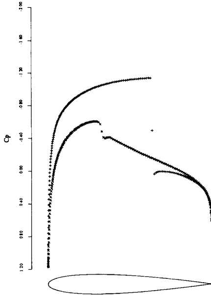
5a: C_p after 75 Cycles. C_l = 0.3620 , C_d = 0.0230 .
