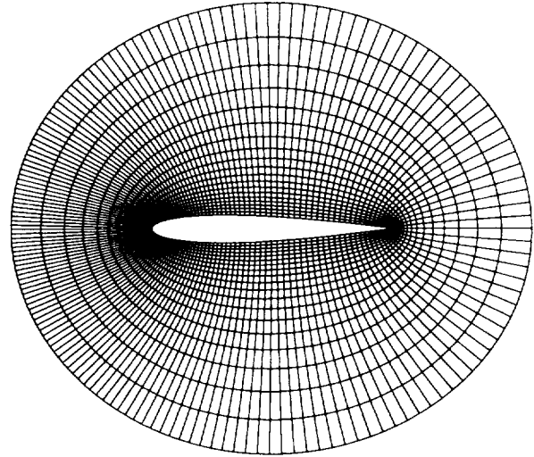
2b: NACA-0012 Airfoil
