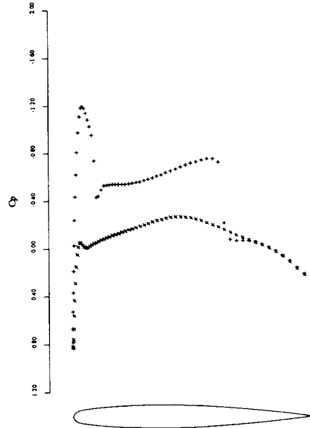
9b: 31.25% Span. C_l = 0.3139, C_d = 0.0159.
