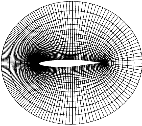
2a: RAE-2822 Airfoil
