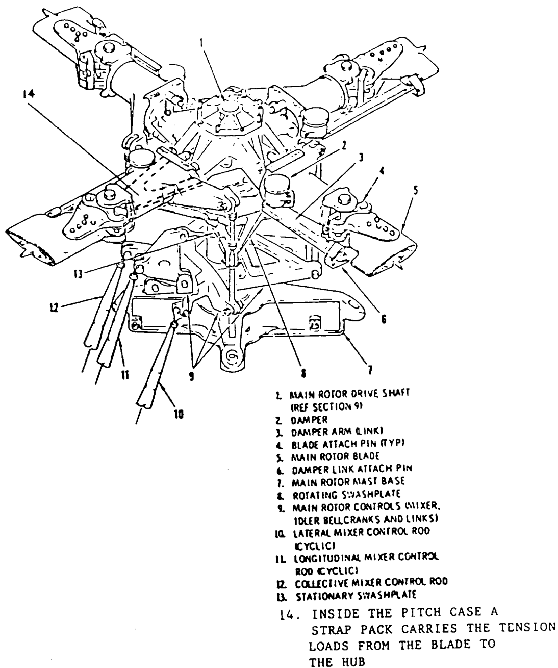
Figure 11.1: OH6A main rotor hub.
