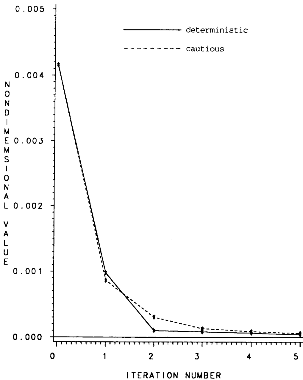
Figure 9.13: Iteration history of longitudinal hub shear for deterministic versus cautious global control, quasisteady aerodynamics, \mu = 0.3 .
