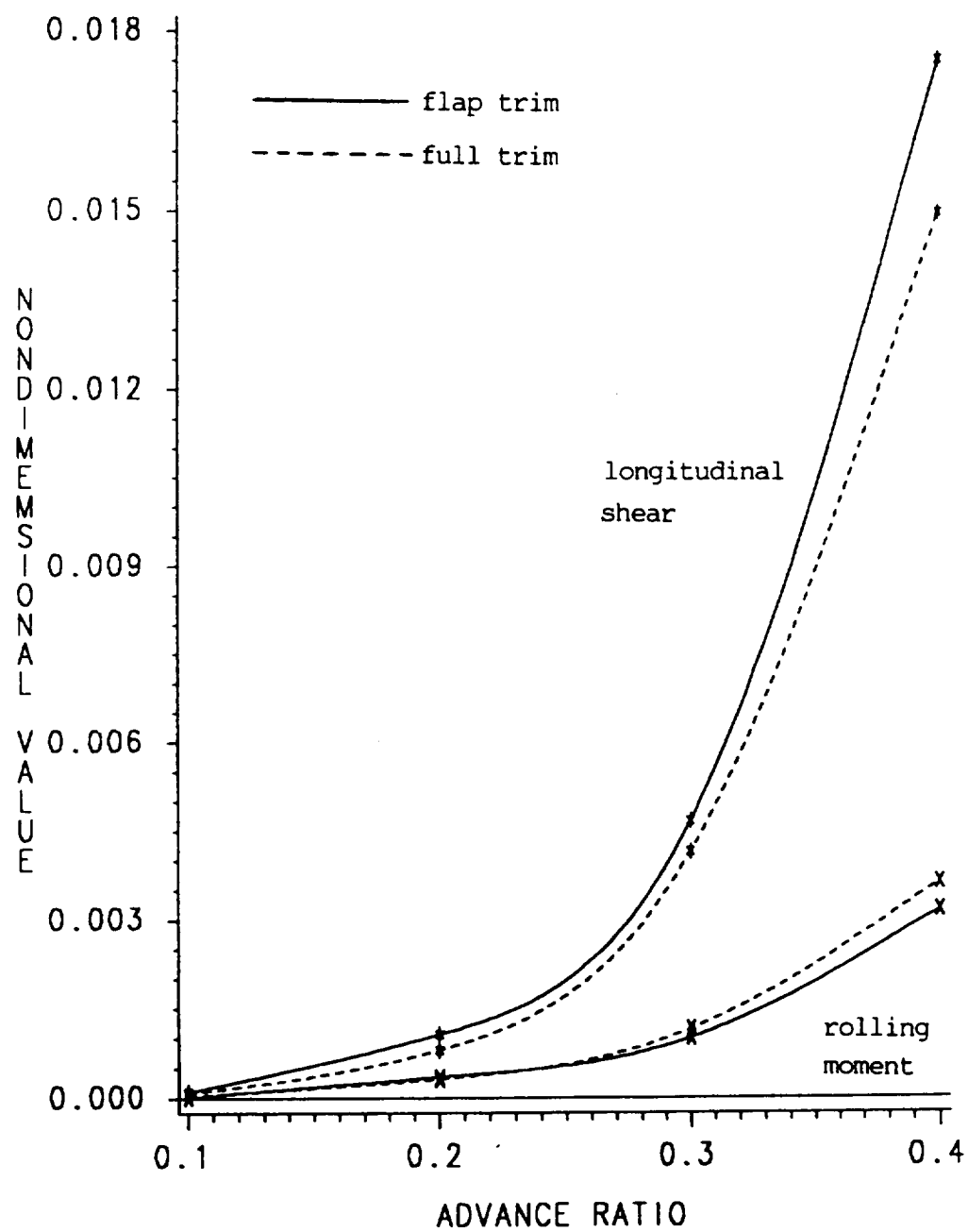
Figure 7.27: Variation of 4/rev. longitudinal shear and rolling moment with advance ratio, soft-in-plane blade, unsteady aerodynamics, flap trim and full trim.
