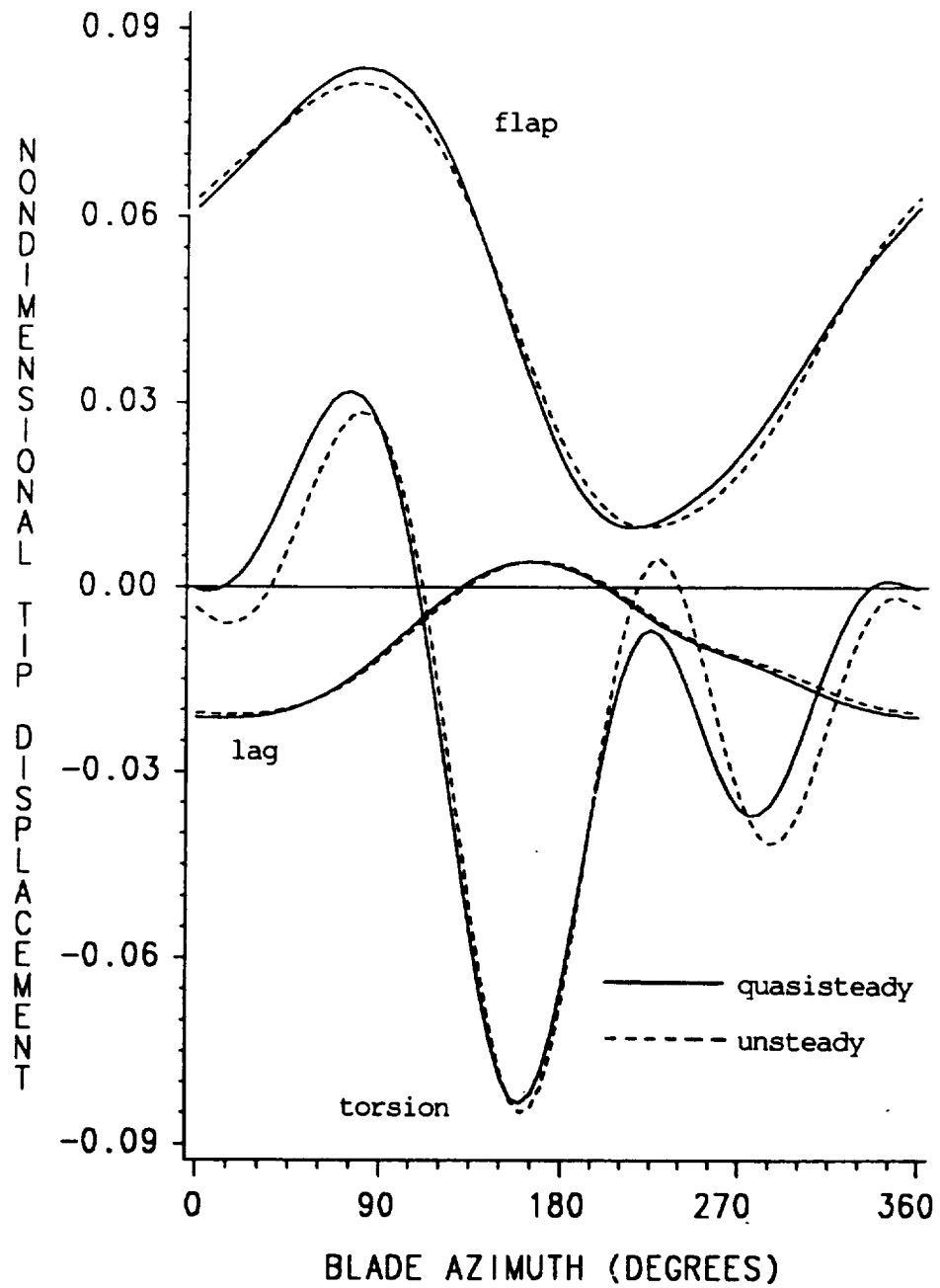
Figure 7.8: Flap, lag, and torsional response, stiff-in-plane blade, advance ratio \mu = 0.4 , quasisteady and unsteady aerodynamics.
