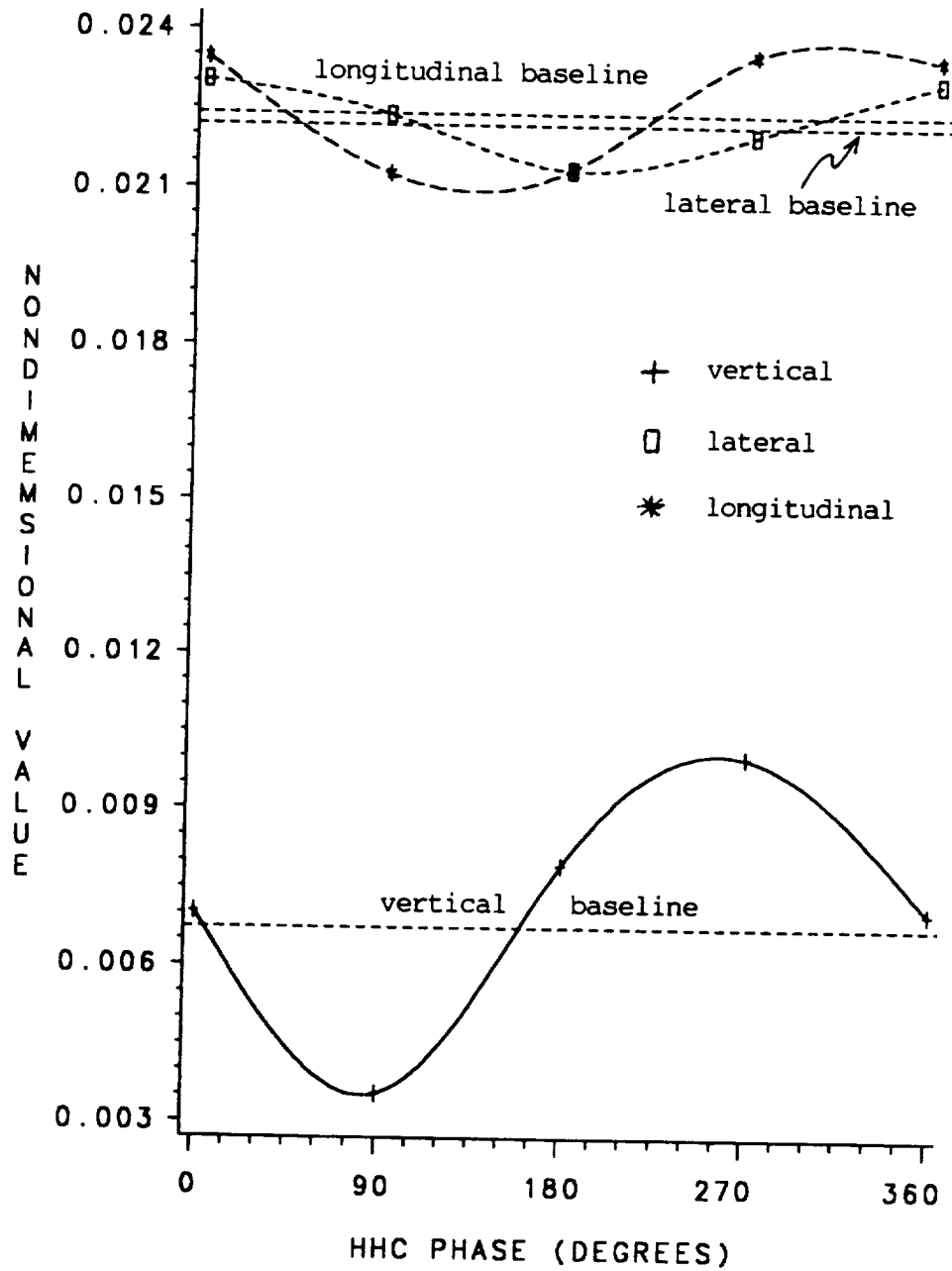
Figure 11.4: Variation of 4/rev. vertical, lateral, and longitudinal hub shears with HHC phase, 1/3^\circ lateral HHC input, OH6A rotor, unsteady aerodynamics, \mu = 0.253 .
