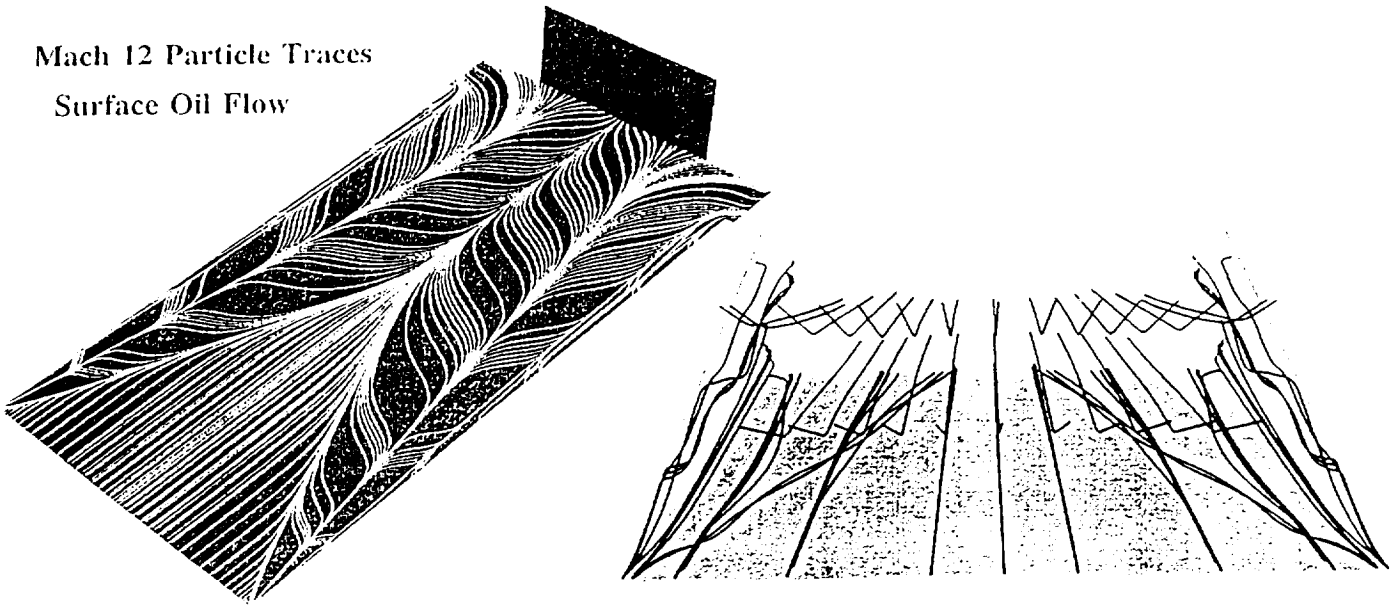
a) Cowl surface path lines
