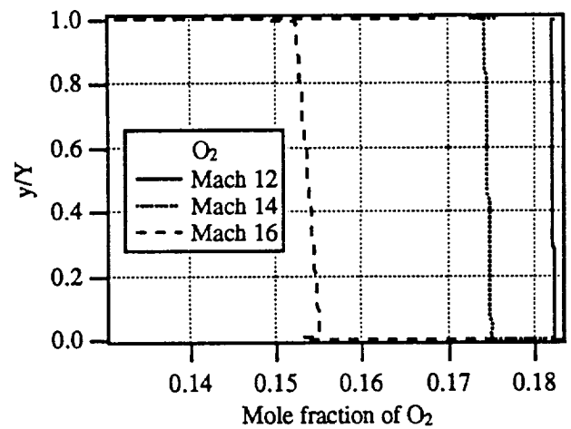
h) Combustor inlet oxygen profiles
