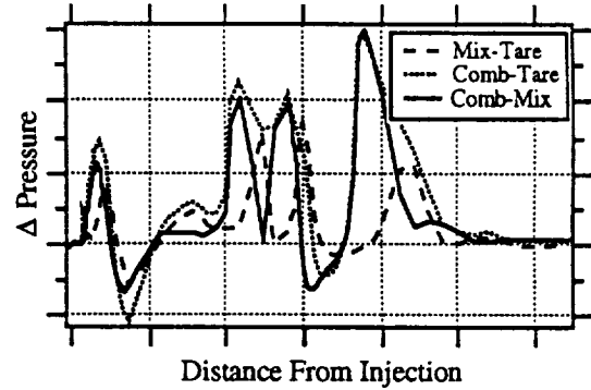
b) Incremental pressure variation
