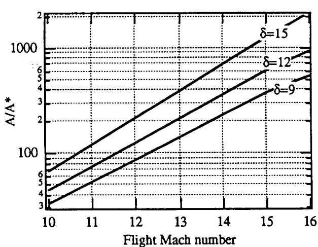
a) Nozzle expansion ratio requirements
