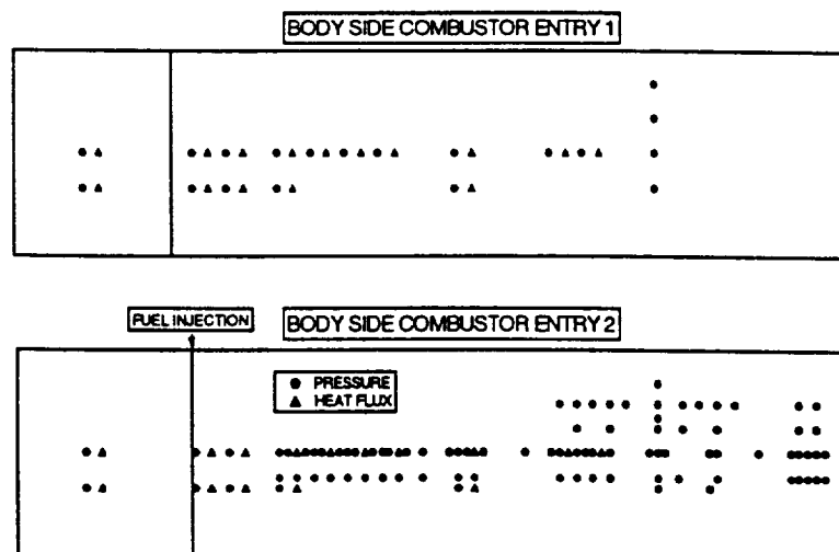
b) Augmented instrumentation layout in combustor
