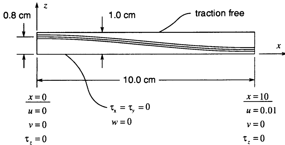
Fig. 5.12 Patch test problem for examining several thin layers.
