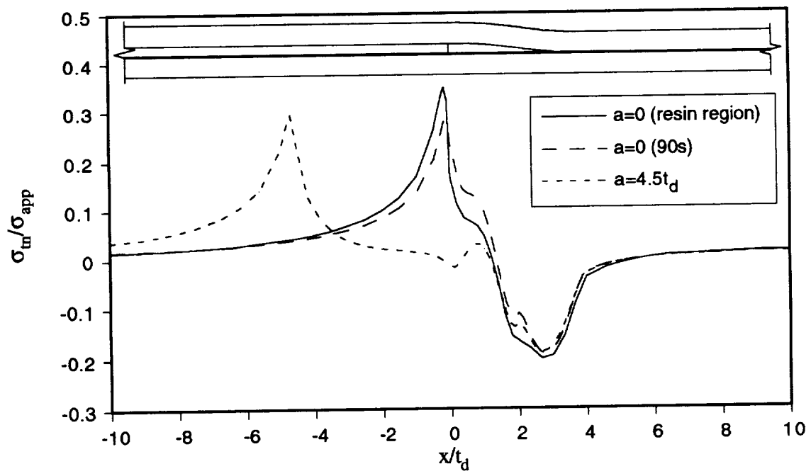
Fig. 6.18 Interlaminar shear stresses along lower interface.
