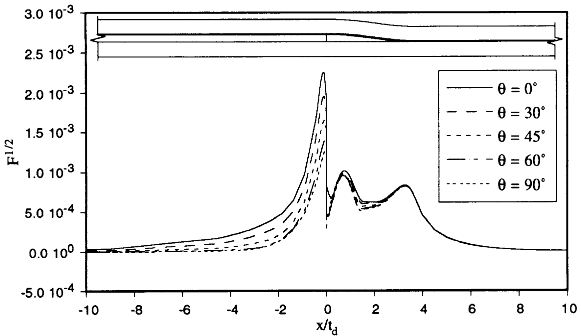
Fig. 6.9 Delamination fraction along the upper interface for different values of \theta of the dropped sublaminate [\pm\theta]_s (longitudinal compression loading).
