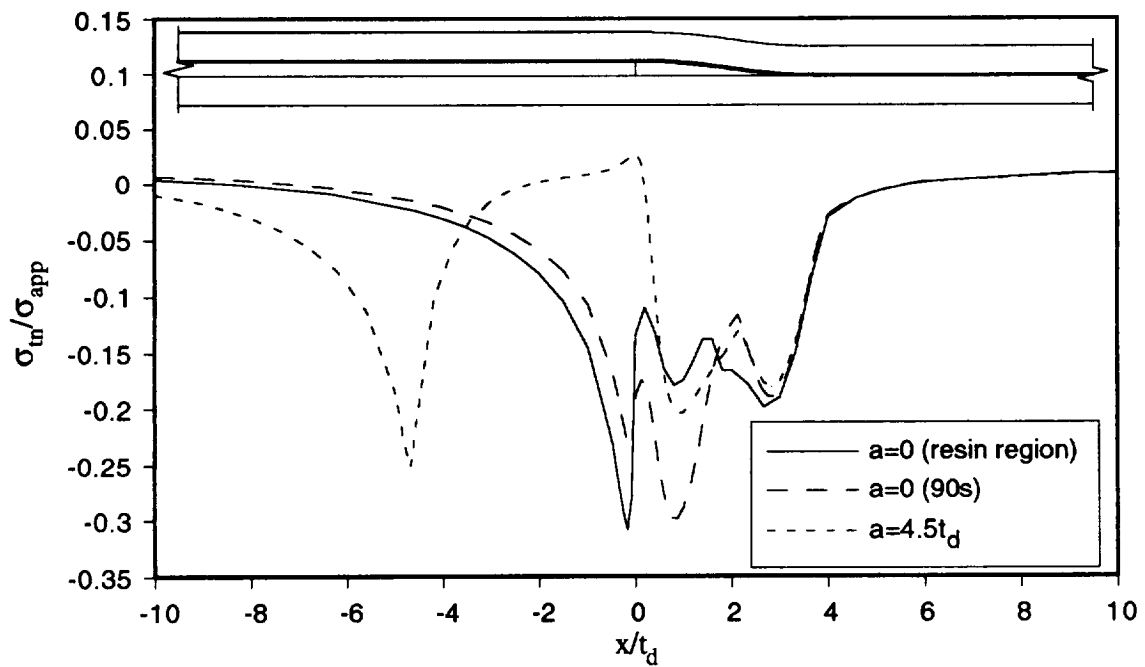
Fig. 6.16 Interlaminar shear stresses along upper interface.
