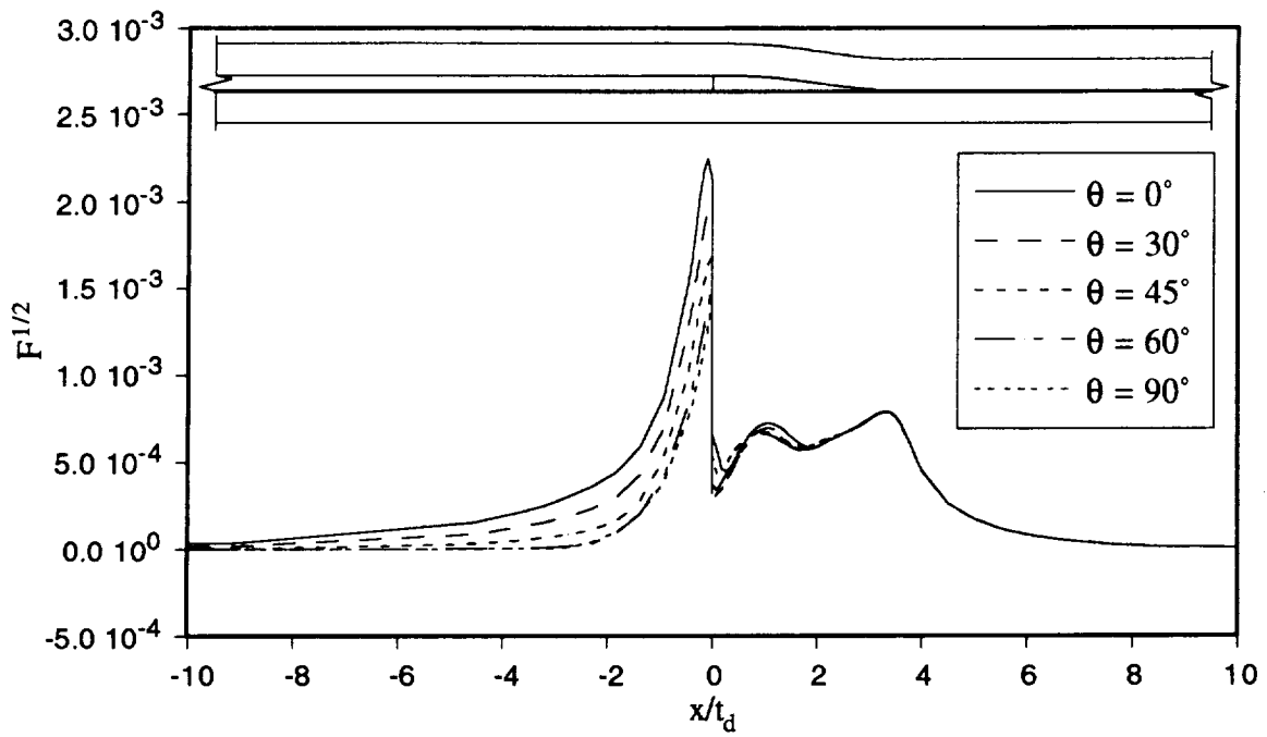
Fig. 6.8 Delamination fraction along the lower interface for different values of \theta of the dropped sublaminate [\pm\theta]_s (longitudinal compression loading).
