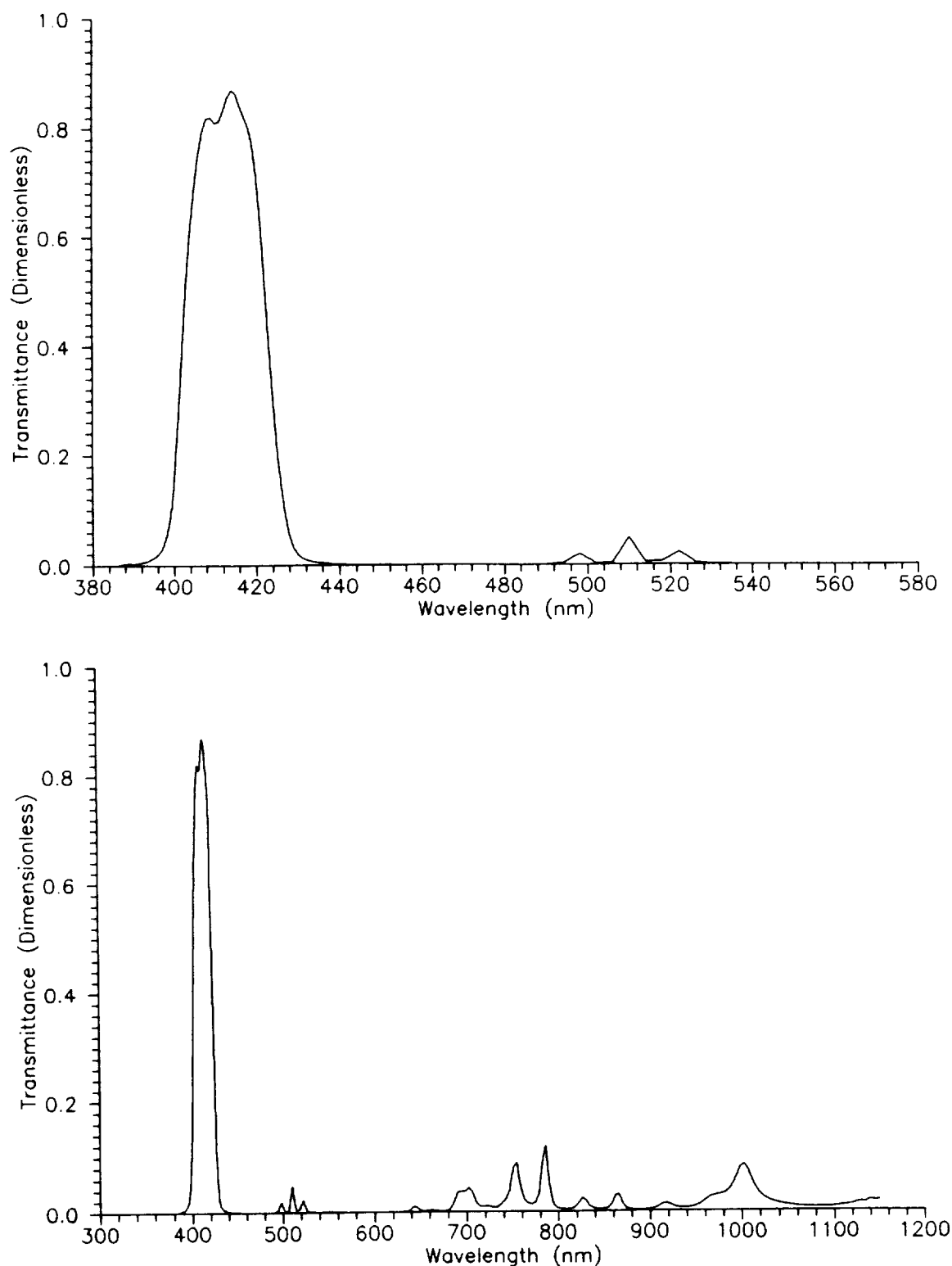
Fig. 12. Transmission curve for the 412nm narrowband interference filter. Vertical scale in linear units. The top panel shows the transmission curve from 380–580 nm covering the pass band of the filter and the out-of-band response near 500 nm. The bottom panel shows the transmission curve for the filter from 380 to 1150 nm showing the complete set of out-of-band responses.
