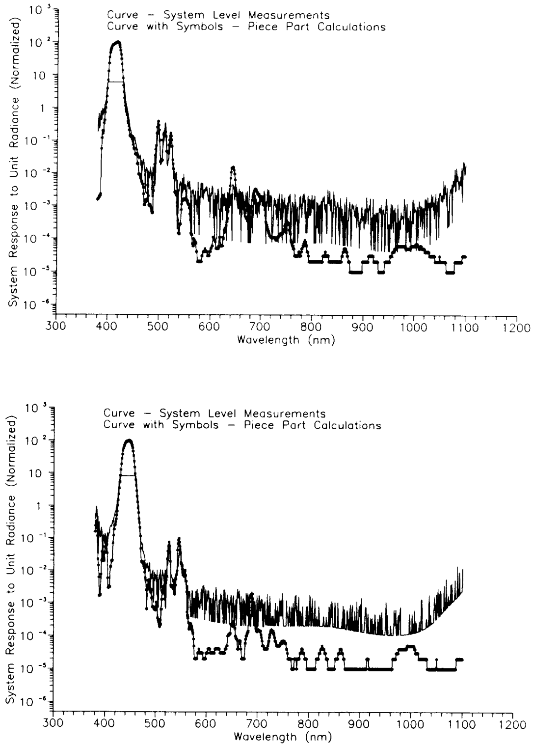
Fig. 28. Out-of-band measurements for the SeaWiFS bands. The curves show the response of the bands to a spectrally flat source as measured at the system level and as calculated from piece part measurements. The responses are normalized to 100%. The top panel shows Band 1 (412 nm). The bottom panel shows Band 2 (443 nm).
