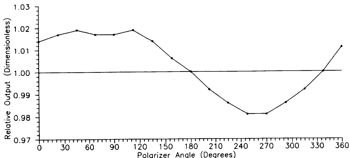
Fig. 7. Polarization sensitivity of SeaWiFS band 1 (412 nm).
