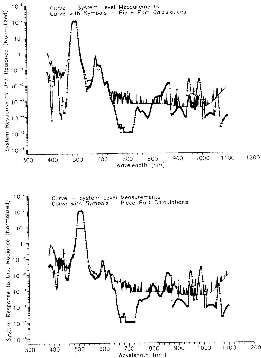
Fig. 29. Out-of-band measurements for the SeaWiFS bands. The curves show the response of the bands to a spectrally flat source as measured at the system level and as calculated from piece part measurements. The responses are normalized to 100%. The top panel shows Band 3 (490 nm). The bottom panel shows Band 4 (510 nm).
