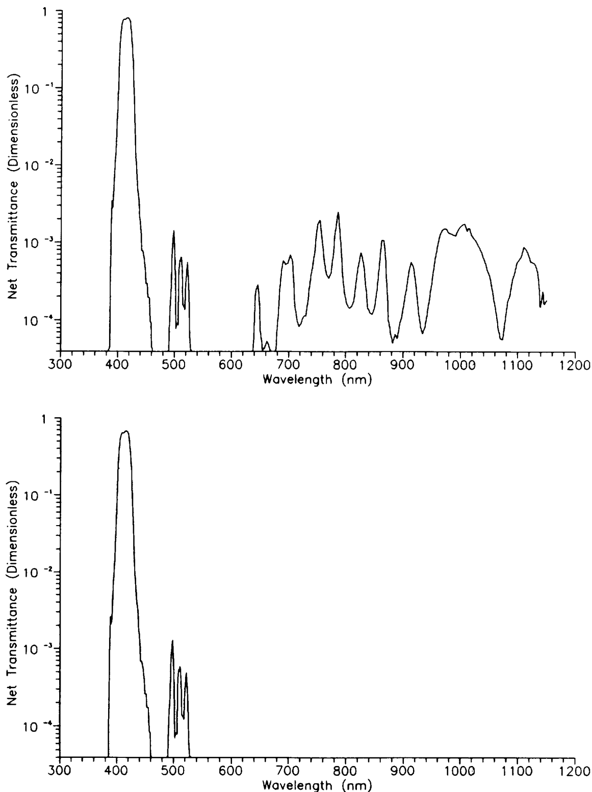
Fig. 14. Combined transmission curves for the interference filter, dichroics, and broadband filters in SeaWiFS band 1. The top panel shows the combined curve for the interference filter and dichroics. Compared with Fig. 10, the out-of-band response has been reduced by about two orders of magnitude. The bottom panel shows the combined curve for the interference filter, dichroics, and broadband filters. The out-of-band response above 600 nm has been further reduced by two orders of magnitude.
