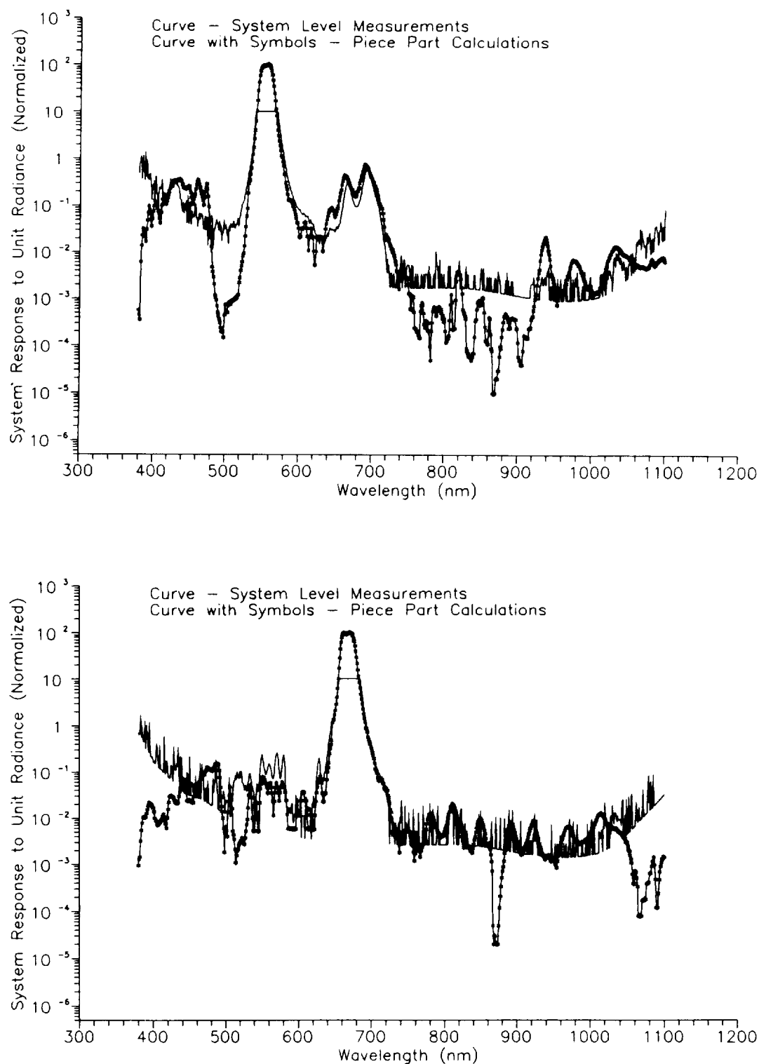
Fig. 30. Out-of-band measurements for the SeaWiFS bands. The curves show the response of the bands to a spectrally flat source as measured at the system level and as calculated from piece part measurements. The responses are normalized to 100%. The top panel shows Band 5 (555 nm). The bottom panel shows Band 6 (670 nm).
