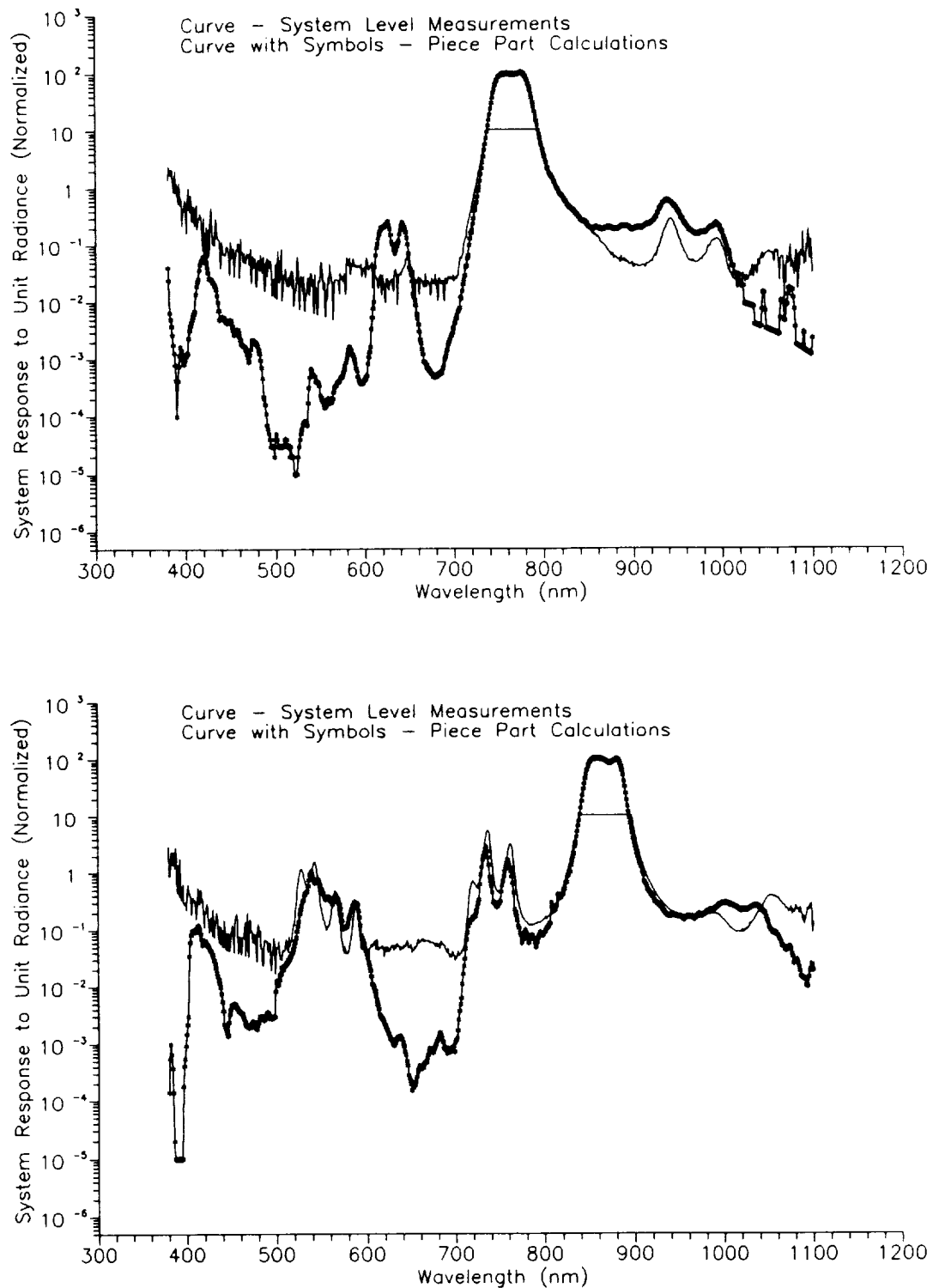
Fig. 31. Out-of-band measurements for the SeaWiFS bands. The curves show the response of the bands to a spectrally flat source as measured at the system level and as calculated from piece part measurements. The responses are normalized to 100%. The top panel shows Band 7 (765 nm). The bottom panel shows Band 8 (865 nm).
