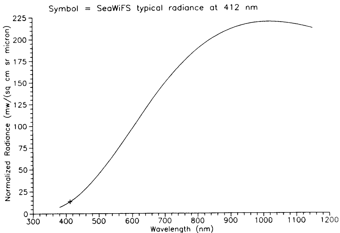
Fig. 17. Blackbody radiance curves normalized to the saturation radiance at 412 nm from the SeaWiFS specifications. The top panel shows the curve for a 5,900 K blackbody that approximates the solar spectrum. The bottom panel shows the curve for a 2,850 K blackbody that approximates the SBRC integrating sphere.
