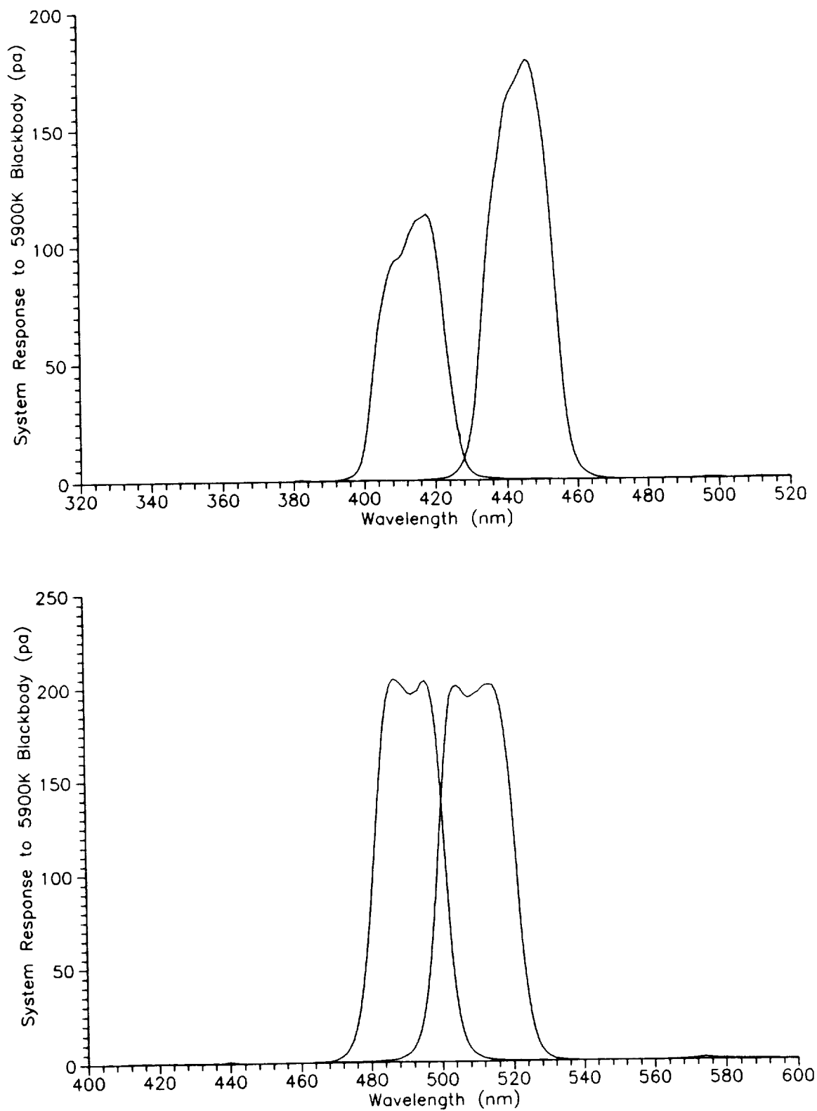
Fig. 19. Instrument output for the SeaWiFS bands. These are the responses of the instrument to a 5,900 K blackbody. The linear scale shows the in-band responses. The top panel shows Bands 1 and 2 (412 and 443 nm). The bottom panel shows Bands 3 and 4 (490 and 510 nm).
