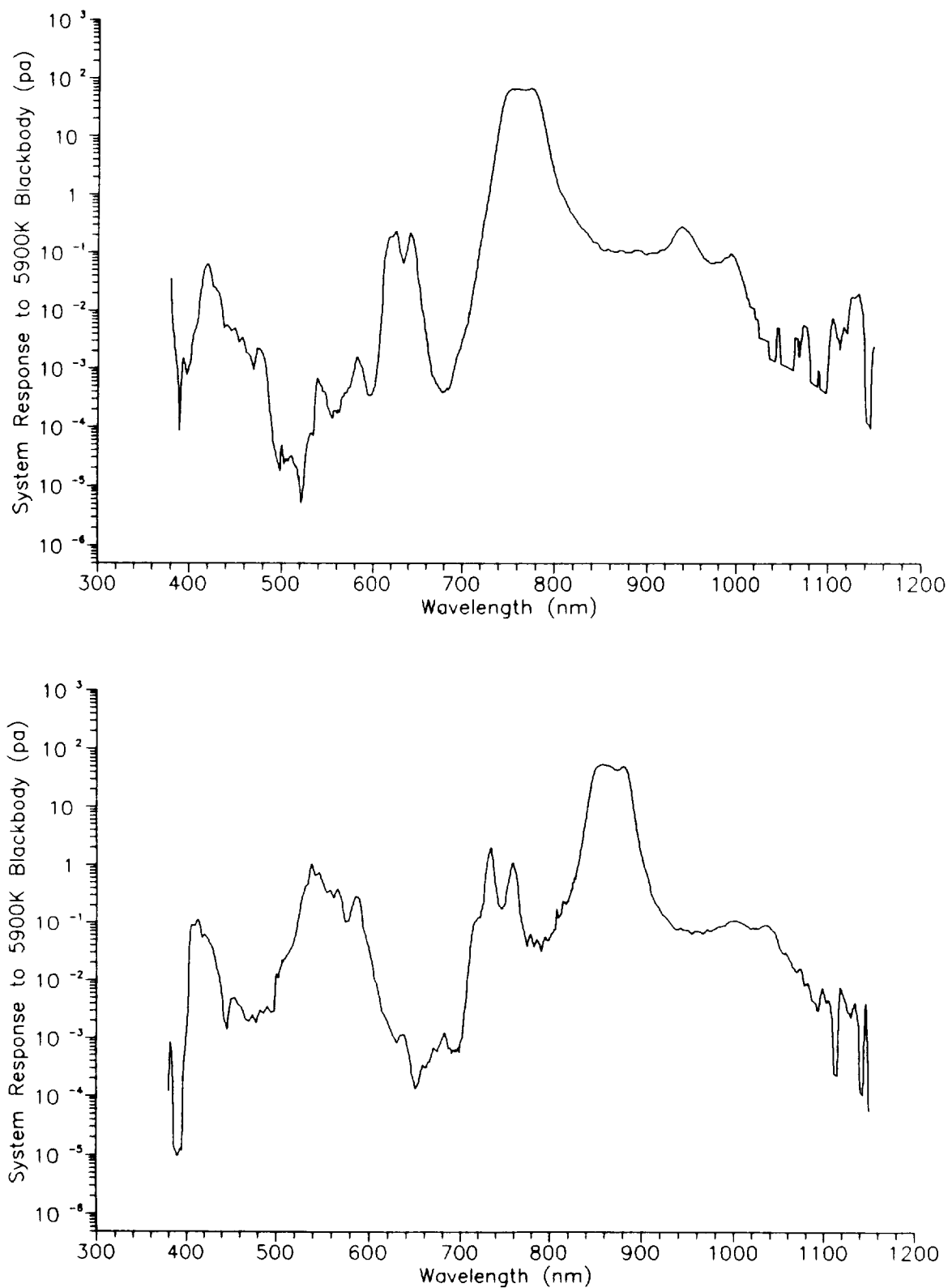
Fig. 24. Instrument output for the SeaWiFS bands. These are the responses of the instrument to a 5,900 K blackbody. The logarithmic scale shows the out-of-band responses. The top panel shows Band 7 (765 nm). The bottom panel shows Band 8 (865 nm).
