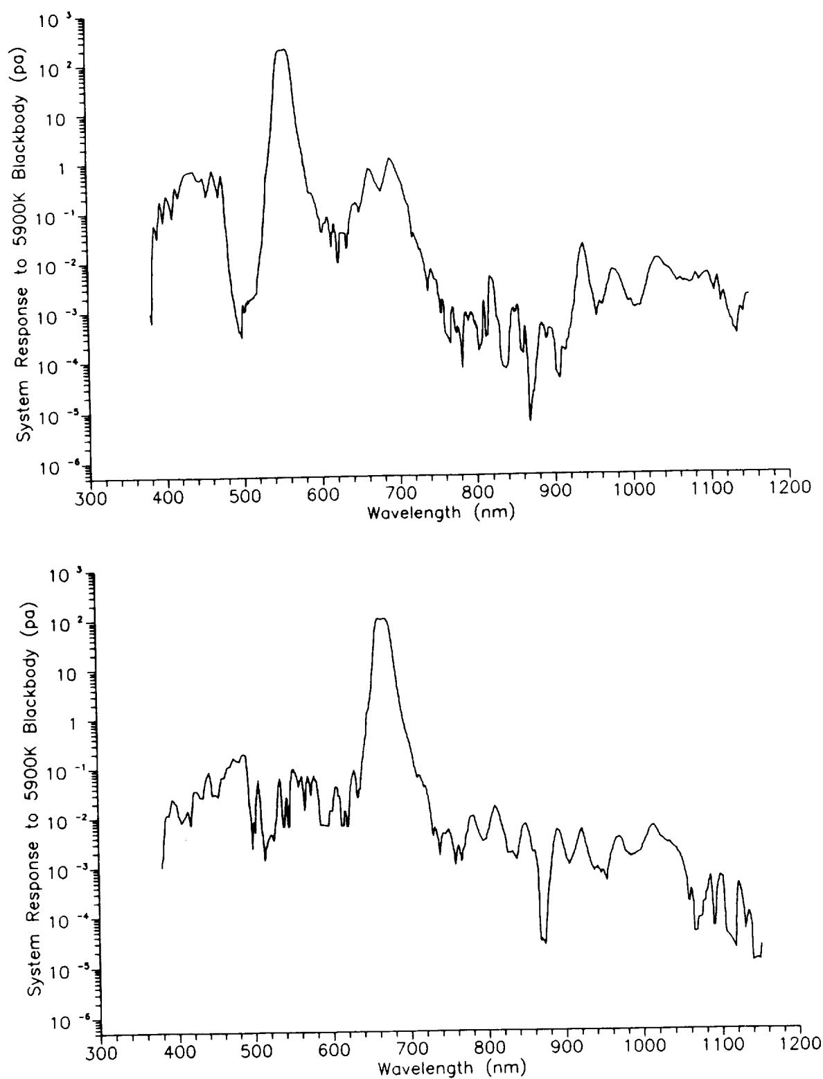
Fig. 23. Instrument output for the SeaWiFS bands. These are the responses of the instrument to a 5,900 K blackbody. The logarithmic scale shows the out-of-band responses. The top panel shows Band 5 (555 nm). The bottom panel shows Band 6 (670 nm).
