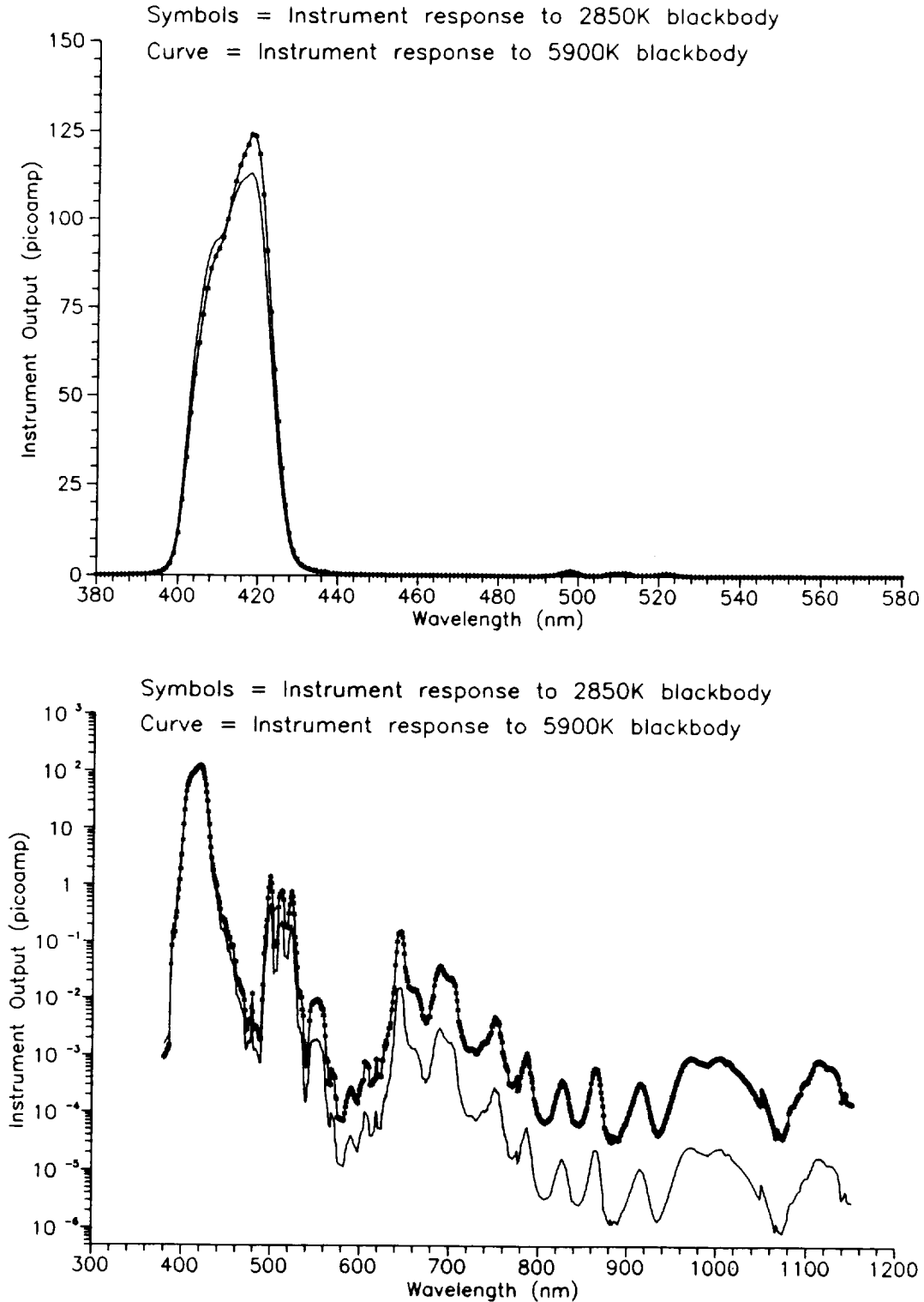
Fig. 18. Instrument output for the two blackbodies. The differences in the instrument's responses to the laboratory and flight sources are a factor in the on-orbit radiometric calibration of the SeaWiFS. The top panel shows the instrument output using a linear scale. This demonstrates the in-band differences from the two light sources. The bottom panel shows the instrument output using a logarithmic scale. This shows the out-of-band differences.
