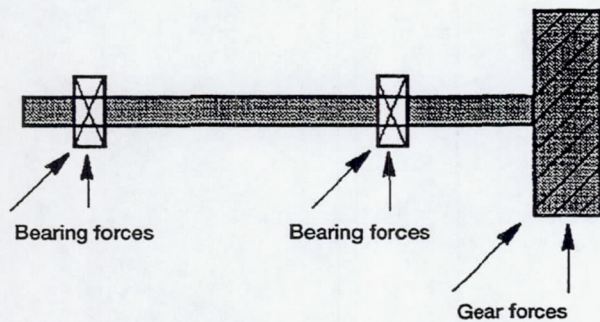
Figure 1.—Schematic of the rotor-gear bearing system.
