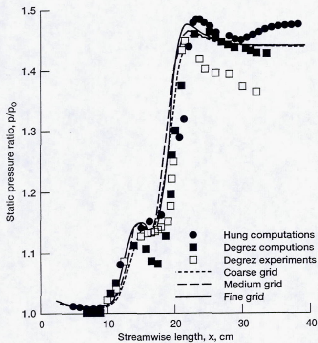
Figure 4.—Comparison of computed and experimental surface pressure distributions at y = 5 cm ( M_o = 2.25 ; \alpha = 6.0^\circ ; and Re_L = 1.08 \times 10^5 ).
