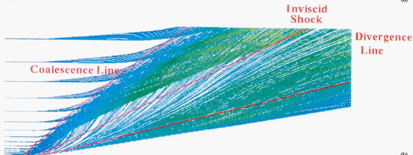
Figure 11.—Computed (a) velocity vectors and (b) particle traces on the flat plate for the turbulent case.
