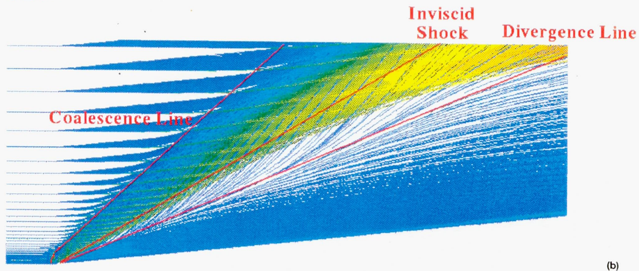
Figure 5.—Computed (a) velocity vectors and (b) particle traces on the flat plate for the laminar case.
