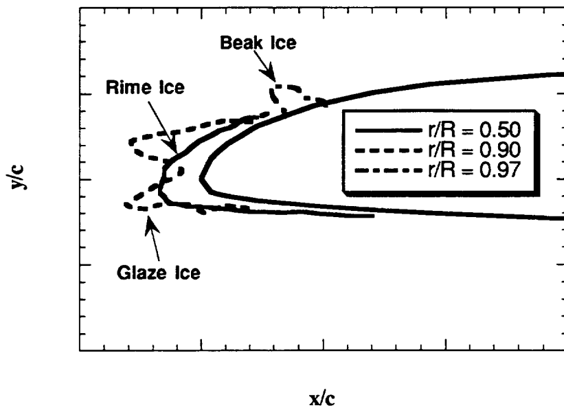
Figure 12. Ice Tracings at several radial locations at a temperature of -12^\circ\text{C} demonstrating transition from Rime to Glaze to Beak ice.
