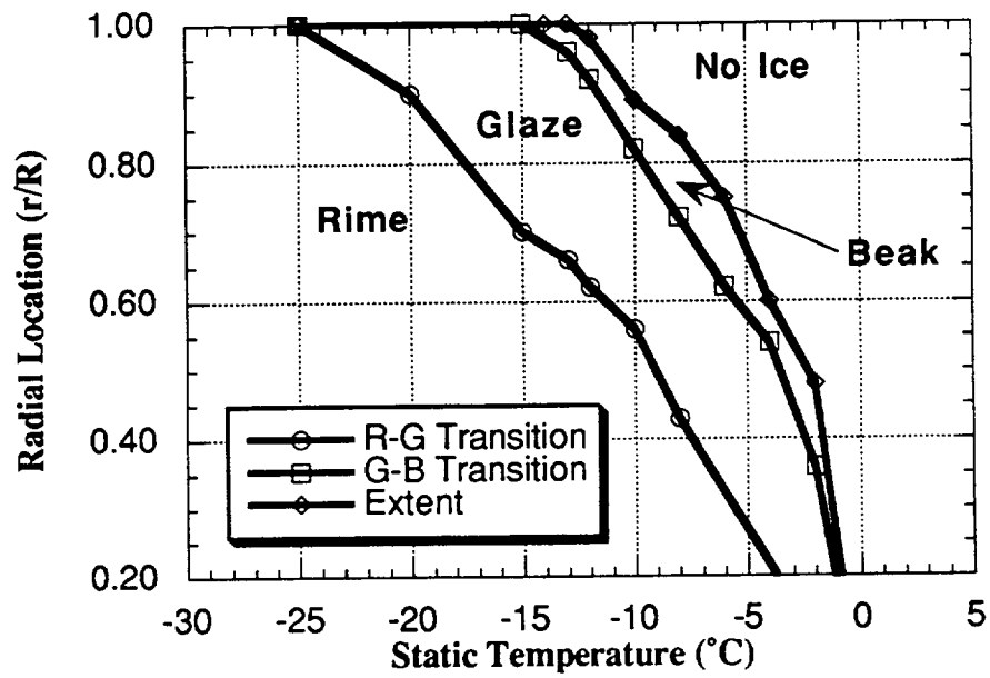
Figure 9. Experimental ice type and extent for \text{LWC} = 0.5 \text{ g/m}^3 (constant collective mode).
