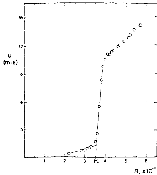
Fig. 4 a) Transition Reynolds number obtained with the fixed hot-wire probe. R_{TR} = 3.5 \times 10^6 .
