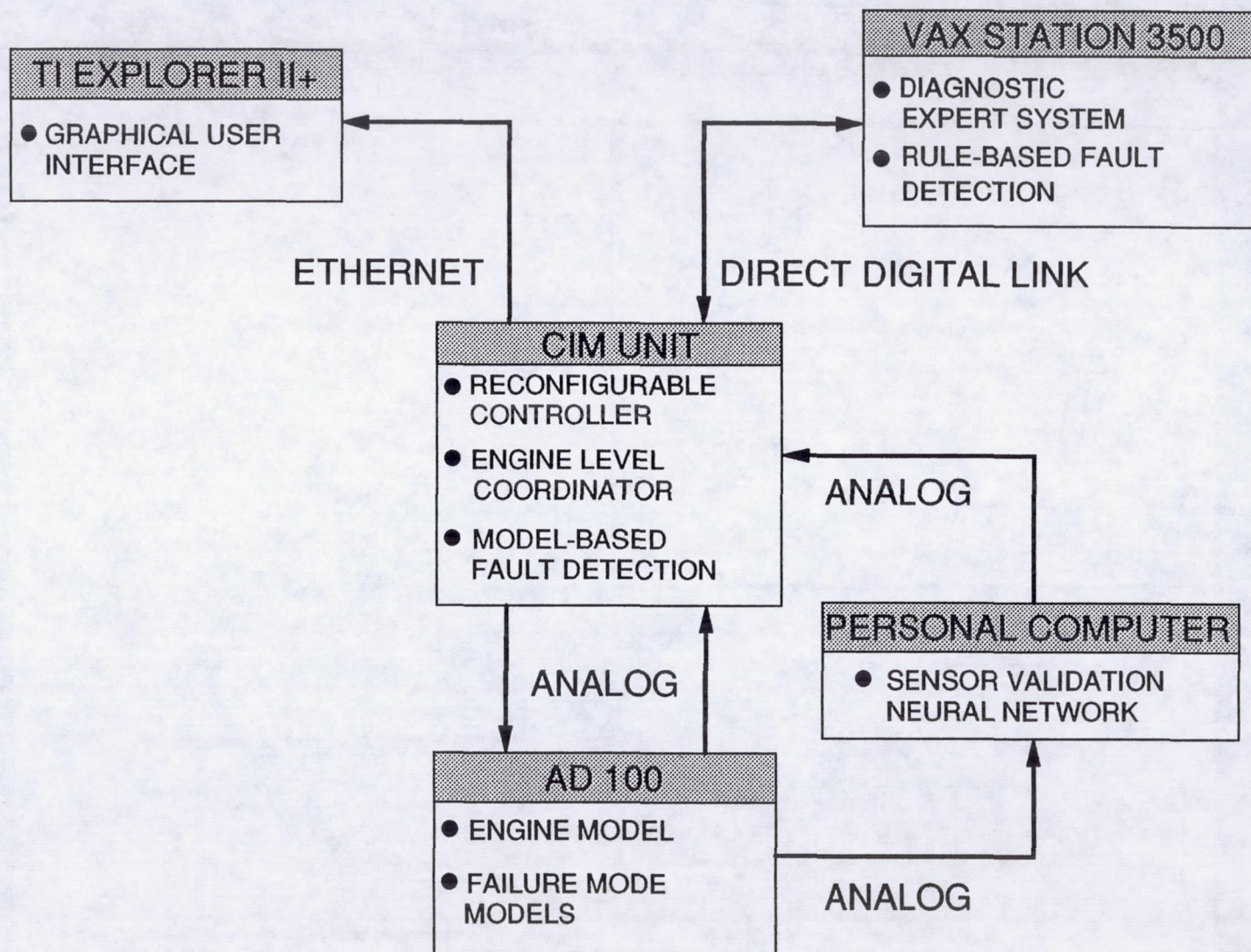
Figure 2. INTELLIGENT CONTROL SYSTEM SIMULATION TEST BED
