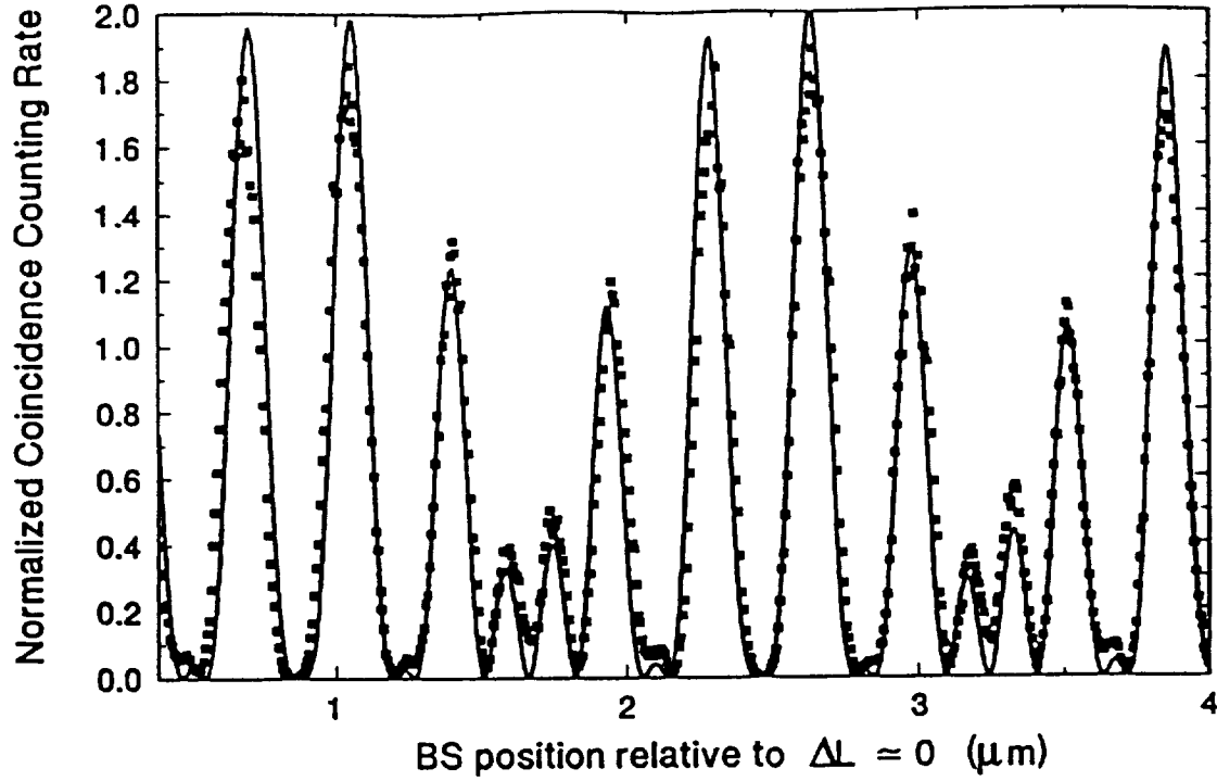
Figure I-2: Normalized coincidence counting rate of N_c at near white light condition ( \Delta L \cong 0 ). The beating frequency, with 3.2 \mu\text{m} period, and sum frequency, with 351.1 \text{ nm} period, are evident from the graph. Signal and idler frequencies, at periods 632.8 \text{ nm} and 788.7 \text{ nm} also contribute. The solid line is a theoretical curve of Eq. (I-10).
