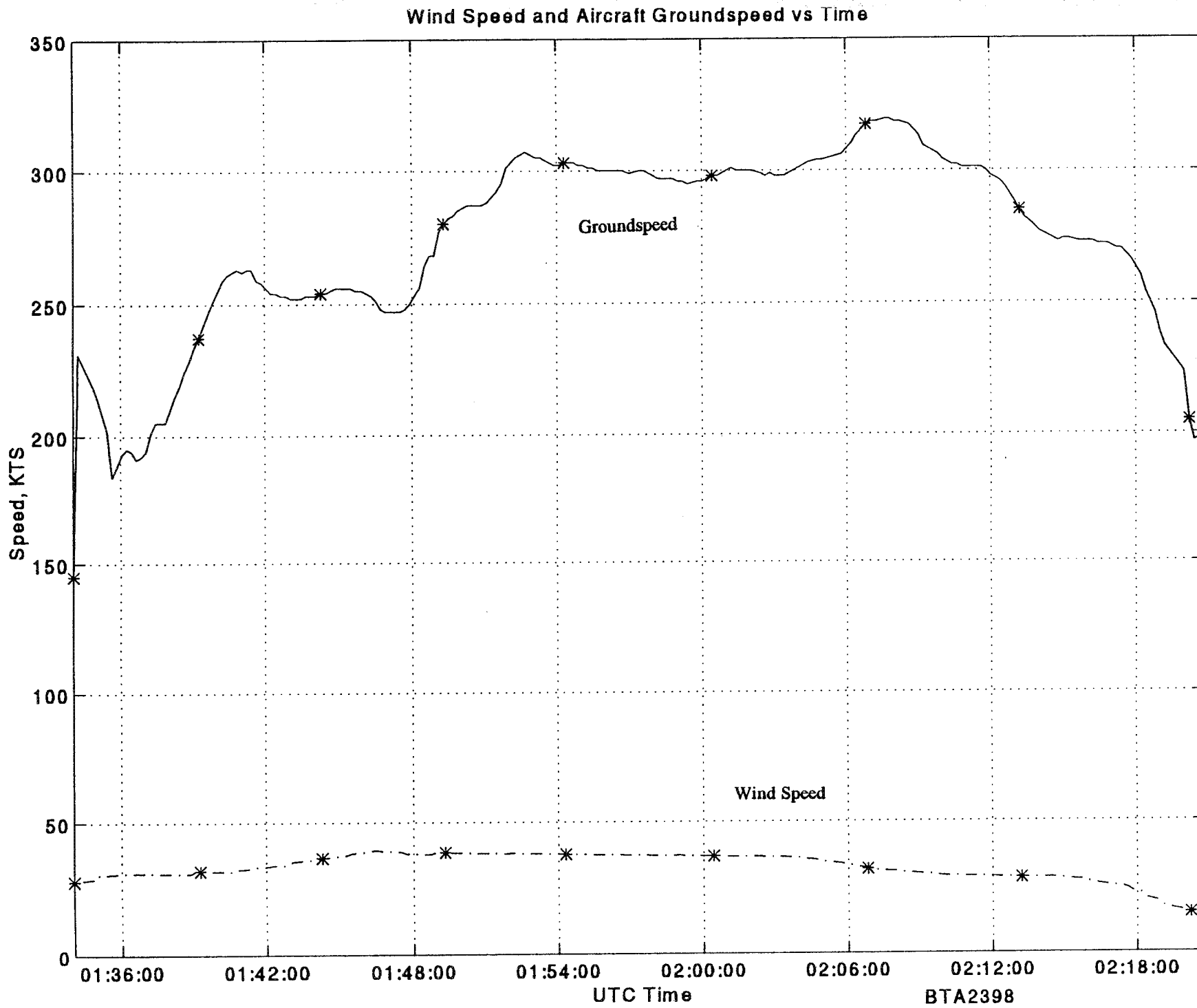
Figure 12: Groundspeed vs Time, BTA2398
