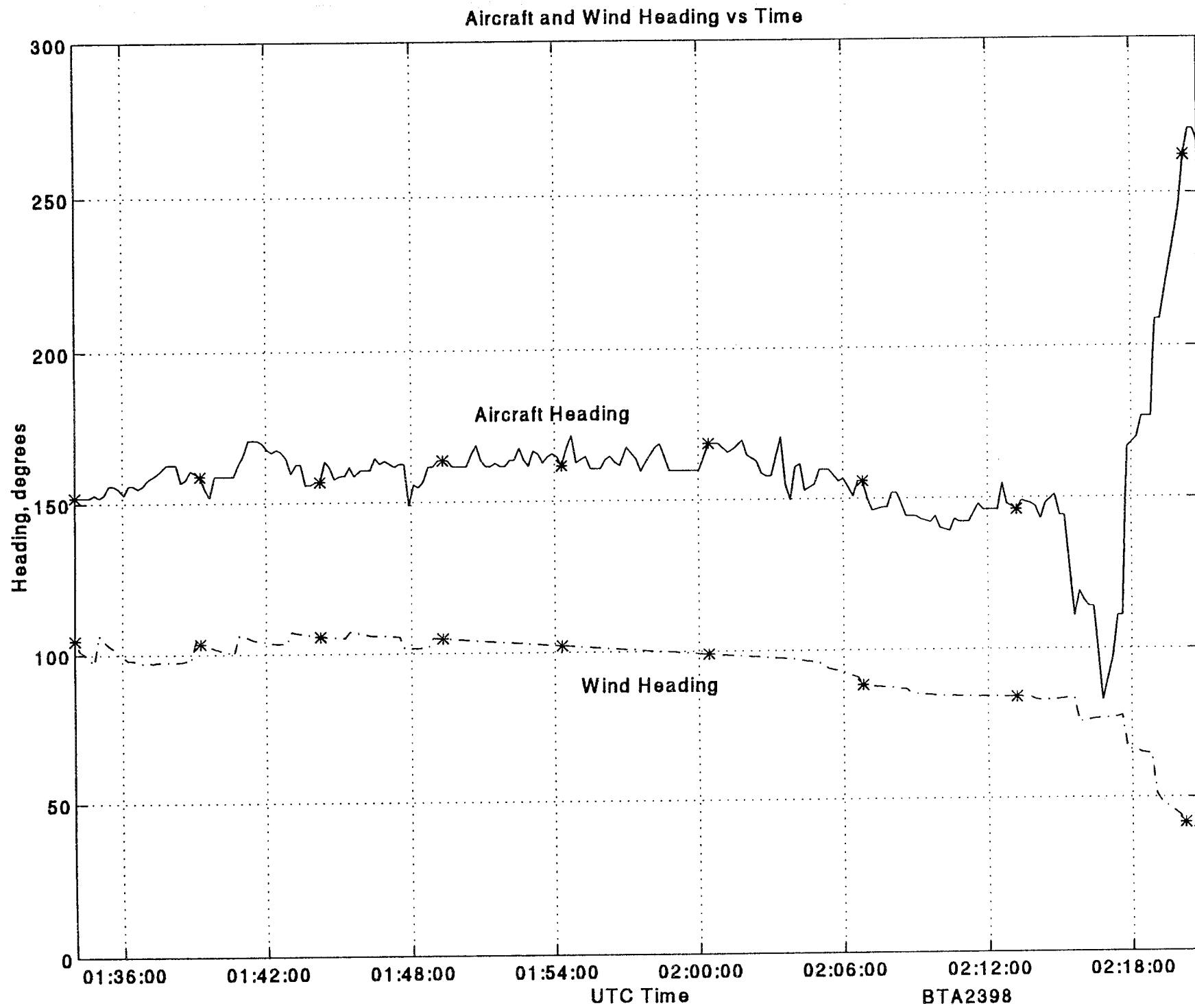
Figure B5: Aircraft Heading and Wind Heading vs Time, BTA2398
