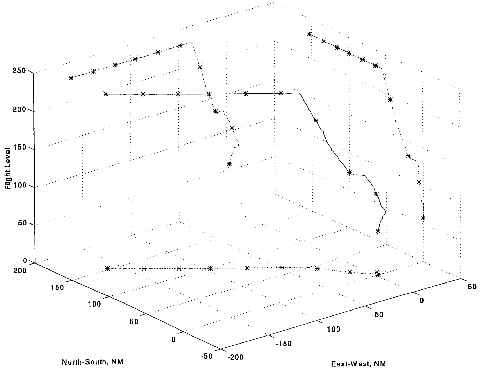
Aircraft Trajectory BTA2296
