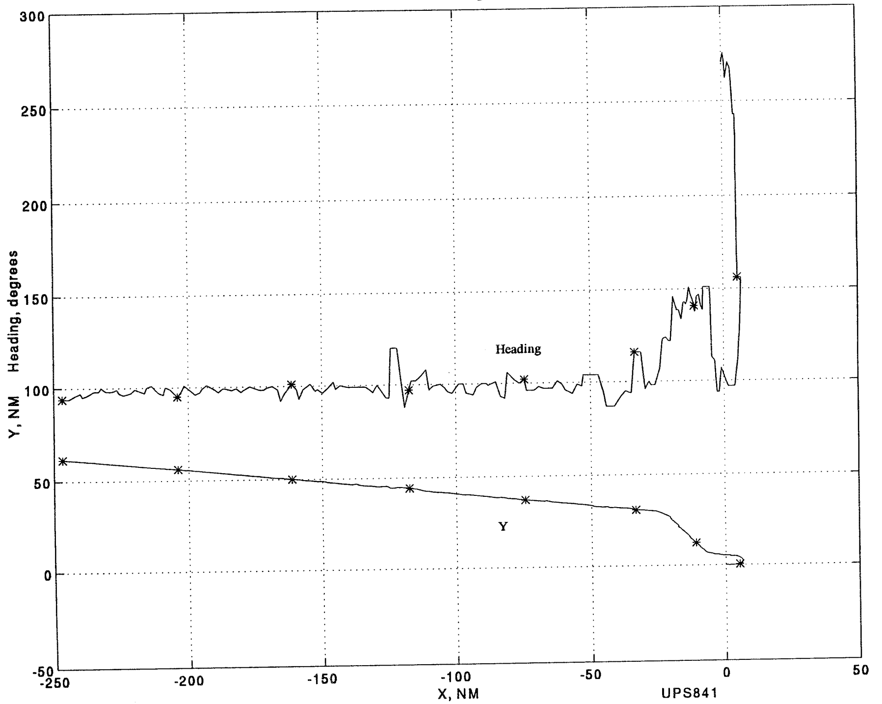
Y and Heading vs X
