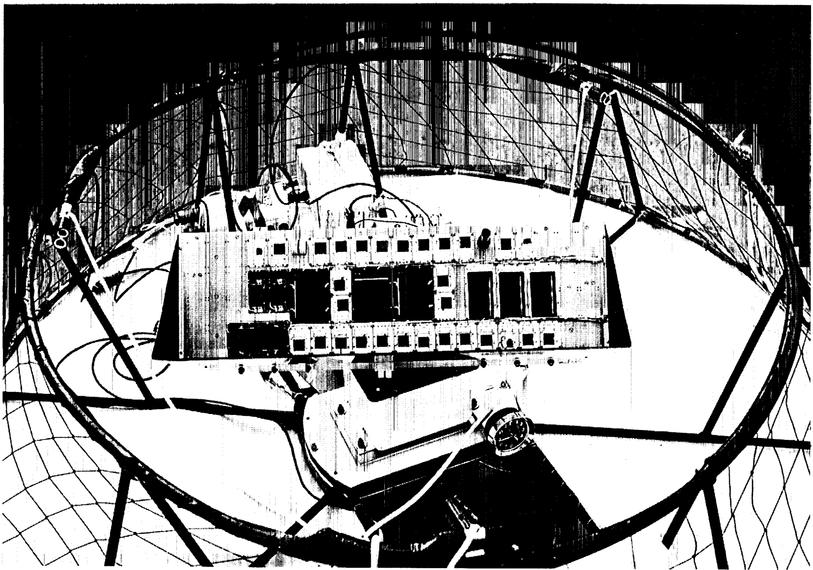
Figure 3. Tracker Mounted on Aluminum Hoop Assembly With 1994 Complement of Flight Modules
