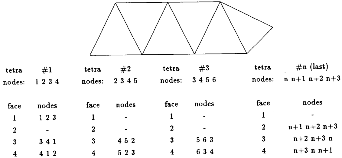
Figure 1: Ploy-Tetrahedral Strip
