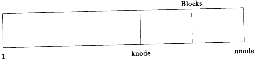
Figure 2: Node Space
